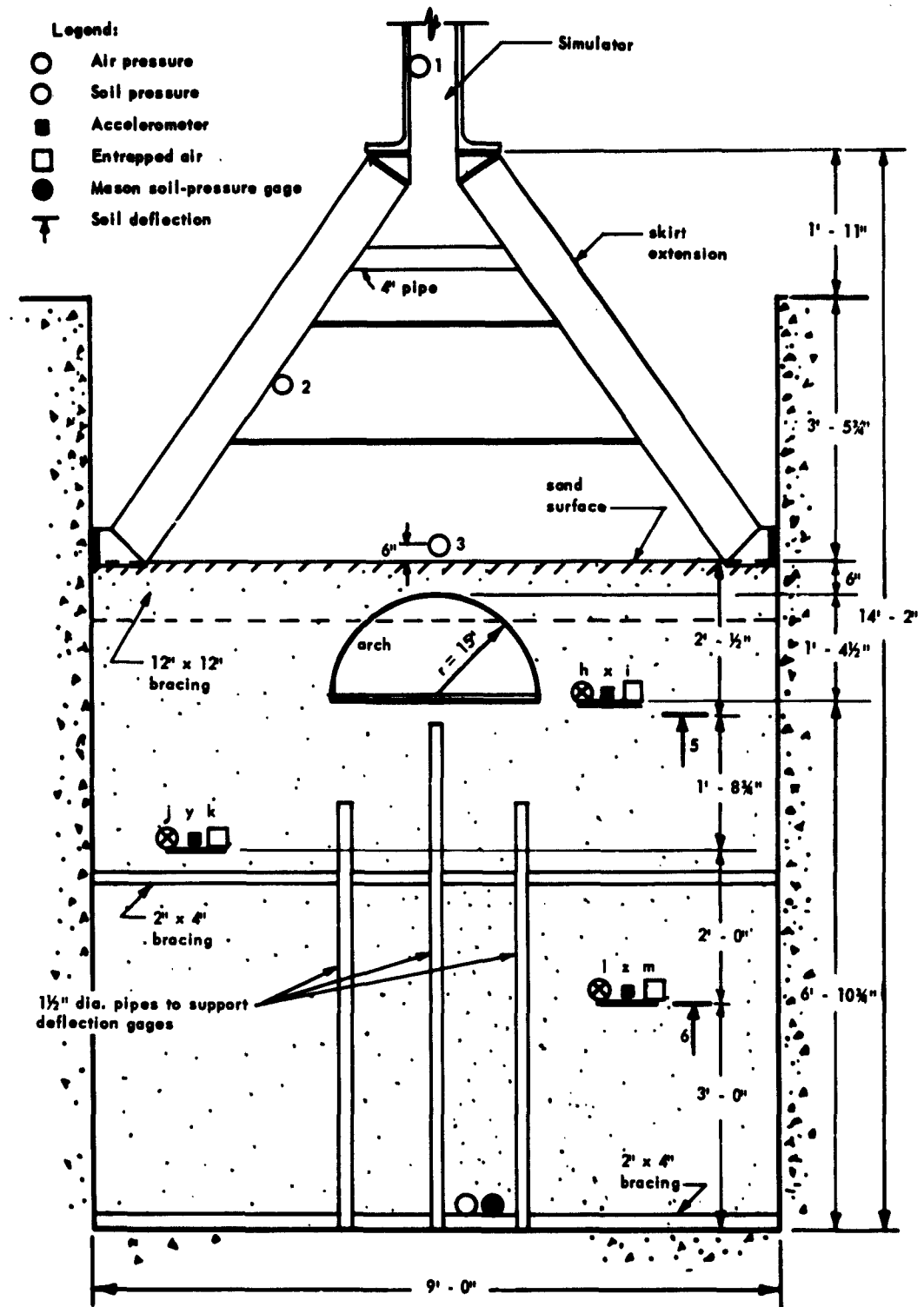
Figure 3. Transverse section of test setup.
