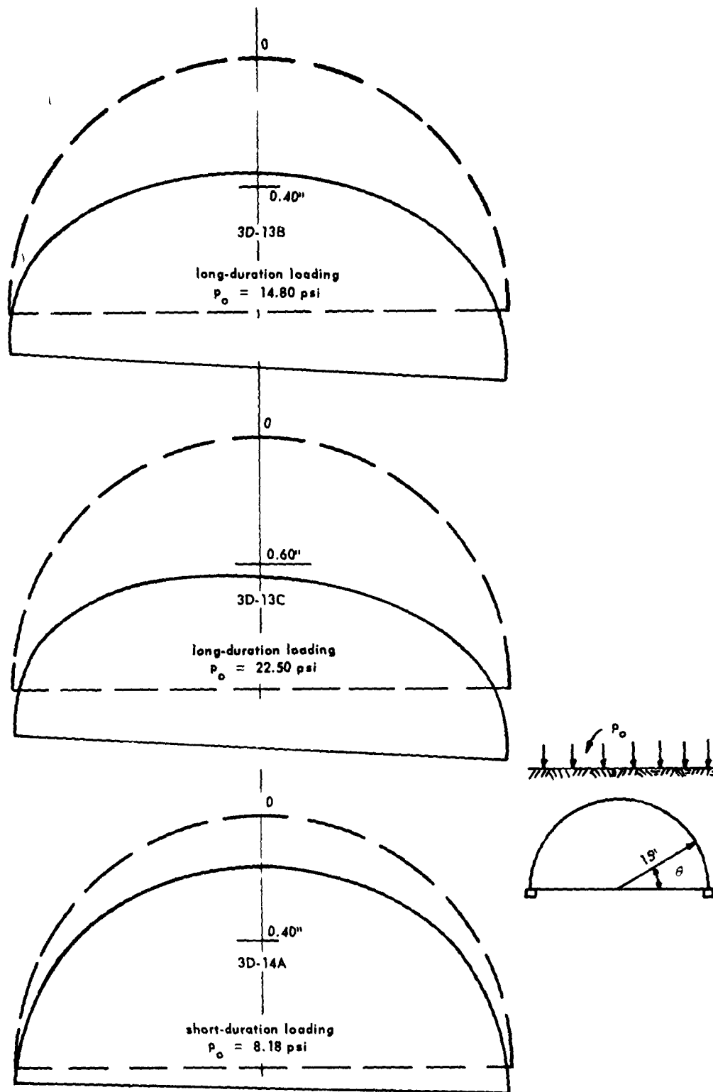
Figure 26. Peak arch deflections due to dynamic loading — 3D-13B, 3D-13C, 3D-14A.
