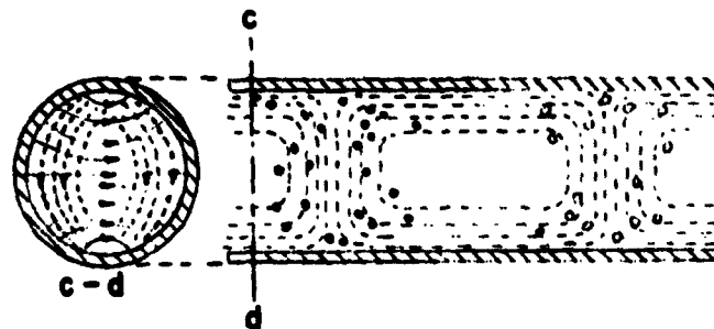
ORIENTATION OF LINES OF ELECTRIC AND MAGNETIC FORCE IN A DOMINANT ( TE_{11} ) WAVE IN A CIRCULAR GUIDE.
