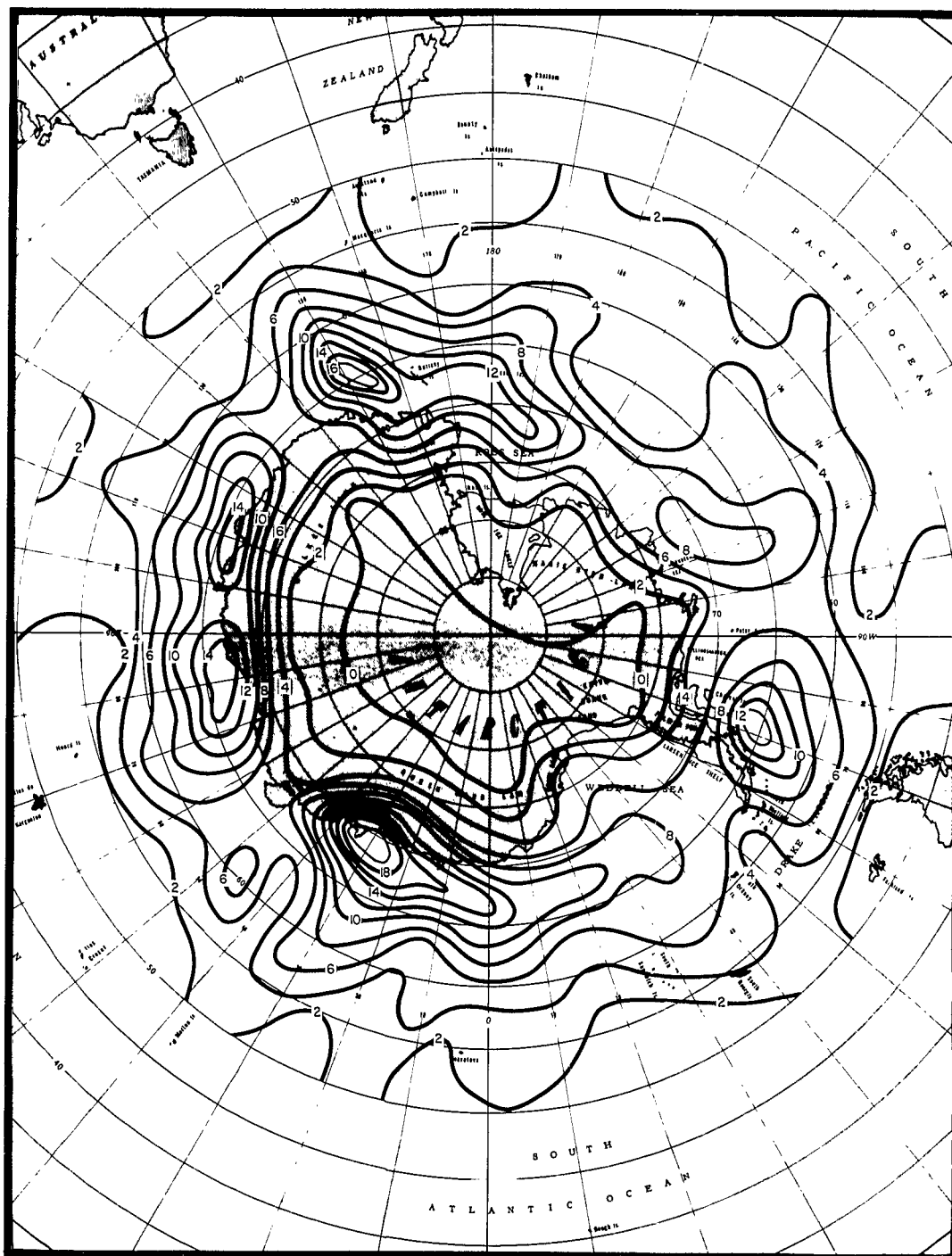
Figure 2.8. Average Percentage Frequency of Occurrence of Low Centers for March.
