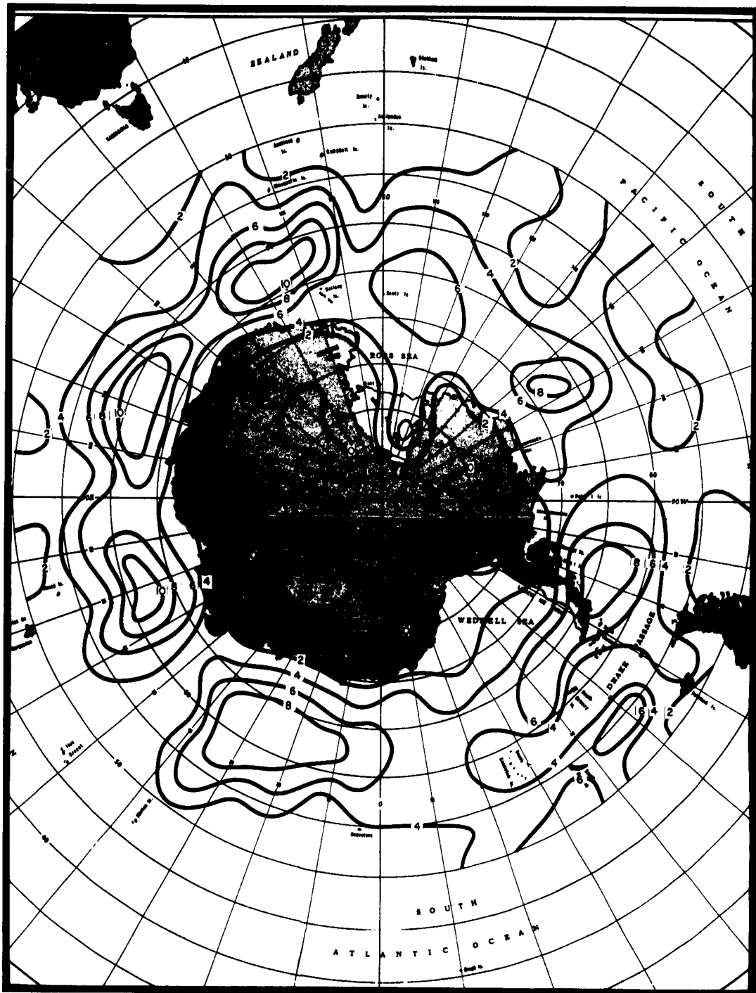
Figure 2.4. Average Percentage Frequency of Occurrence of Low Centers for January.
