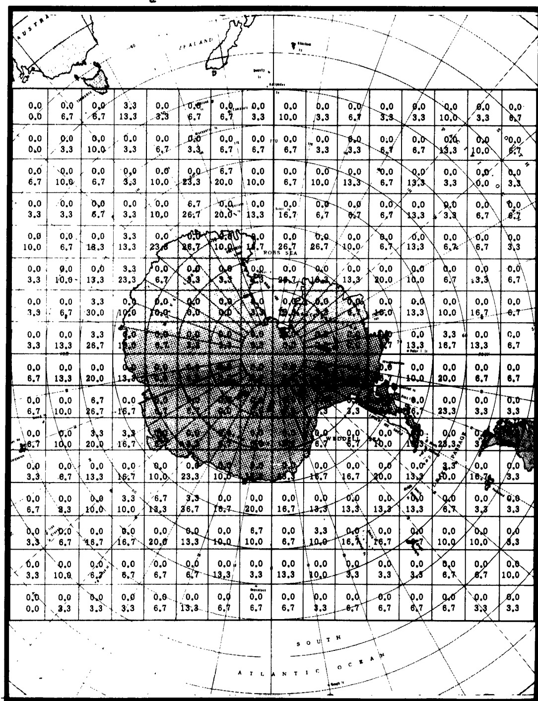
Figure 2.11. Range of Average Monthly Values of Percentage Frequency of Occurrence of Low Centers for April.
