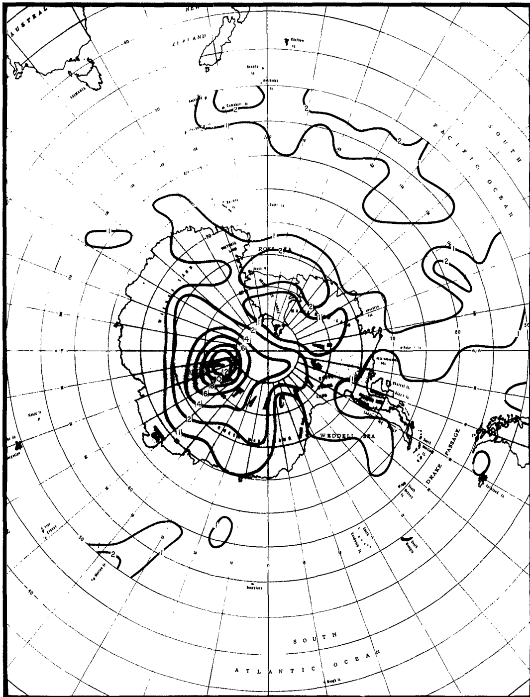
Figure 3.10. Percentage Frequency of Occurrence of High Centers for August.
