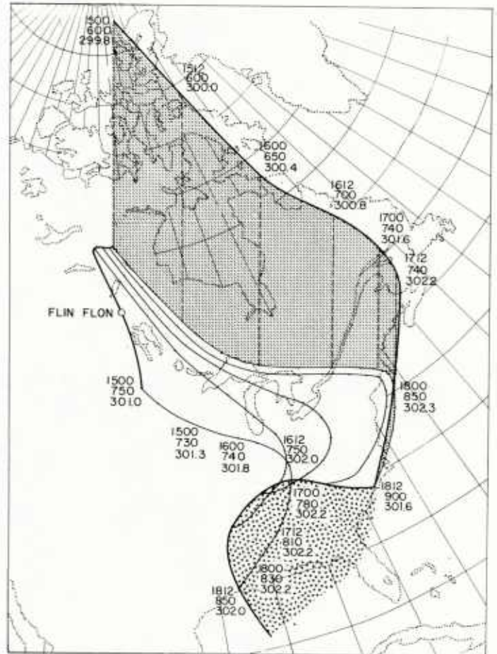
Fig. 20 Same as Fig. 19, only for boundary of fallout region of September 18, 12 GCT. Map times, isentropic stream-function values, and pressures, again, are plotted along the "three-dimensional" and the southernmost trajectories. Marks along the plane trajectories indicate 6-hour displacements.
