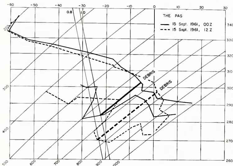
Fig. 6 Temperature and dew point temperature soundings of The Pas(867), 15 September 1961, 0000 and 1200 GCT, plotted on a tephigram. Horizontal coordinate: temperature; vertical coordinate: potential temperature; curved lines from lower left to upper right: pressure; lines labeled 0.8 and 1.0 are lines of constant mixing ratio. The pressure levels at which the debris clouds were encountered are marked by a heavy solid, respectively dashed line.
