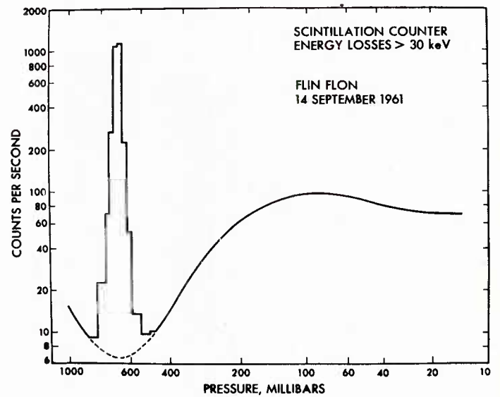
Fig. 4 Scintillation counts per second (ordinate) as a function of pressure (mb) for balloon flight of 14 September 1961, 22 GCT, released from Flin Flon, Canada.
