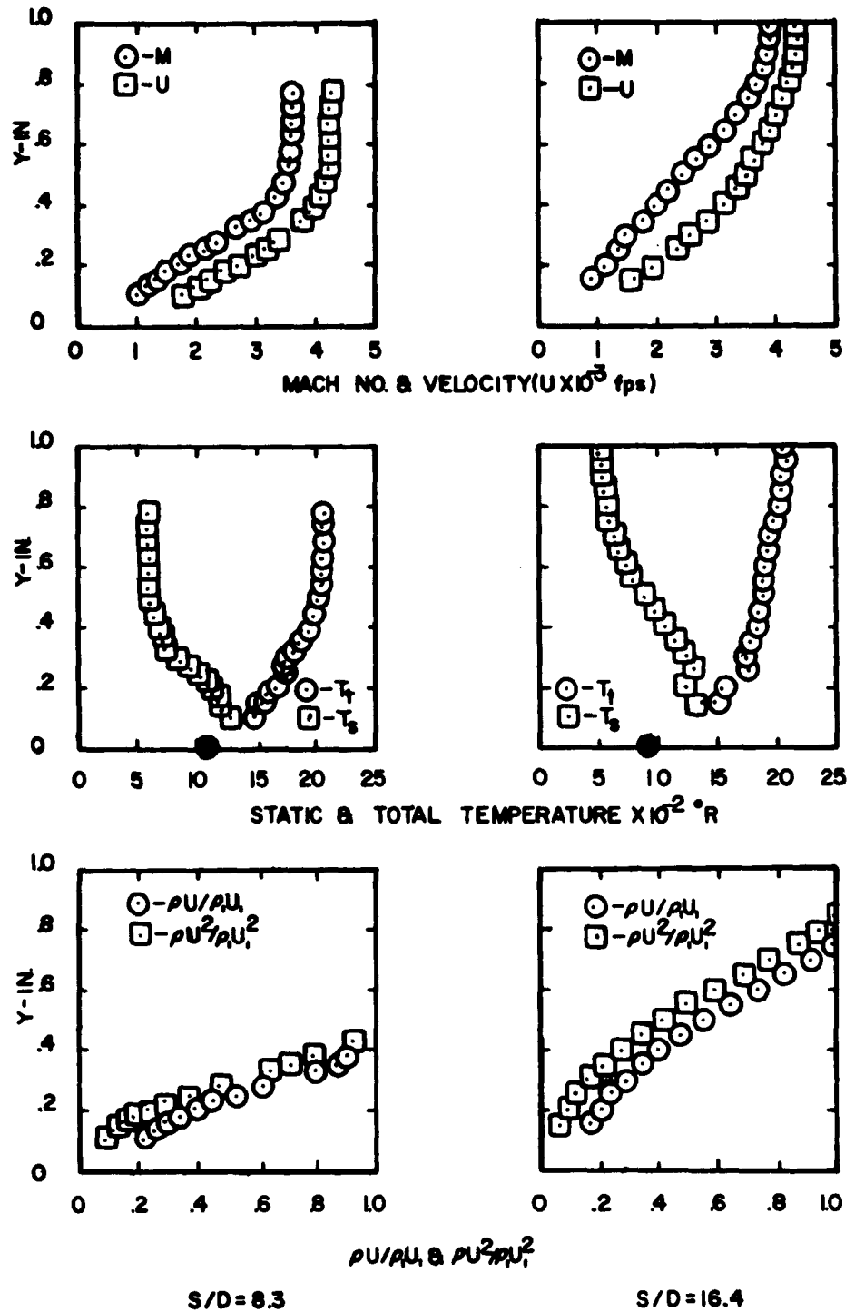
FIG.17 BOUNDARY LAYER ON PLATE AT ANGLE OF ATTACK ( 15^\circ EXP.) FOR M_\infty=10 AND Re_D=11,000
