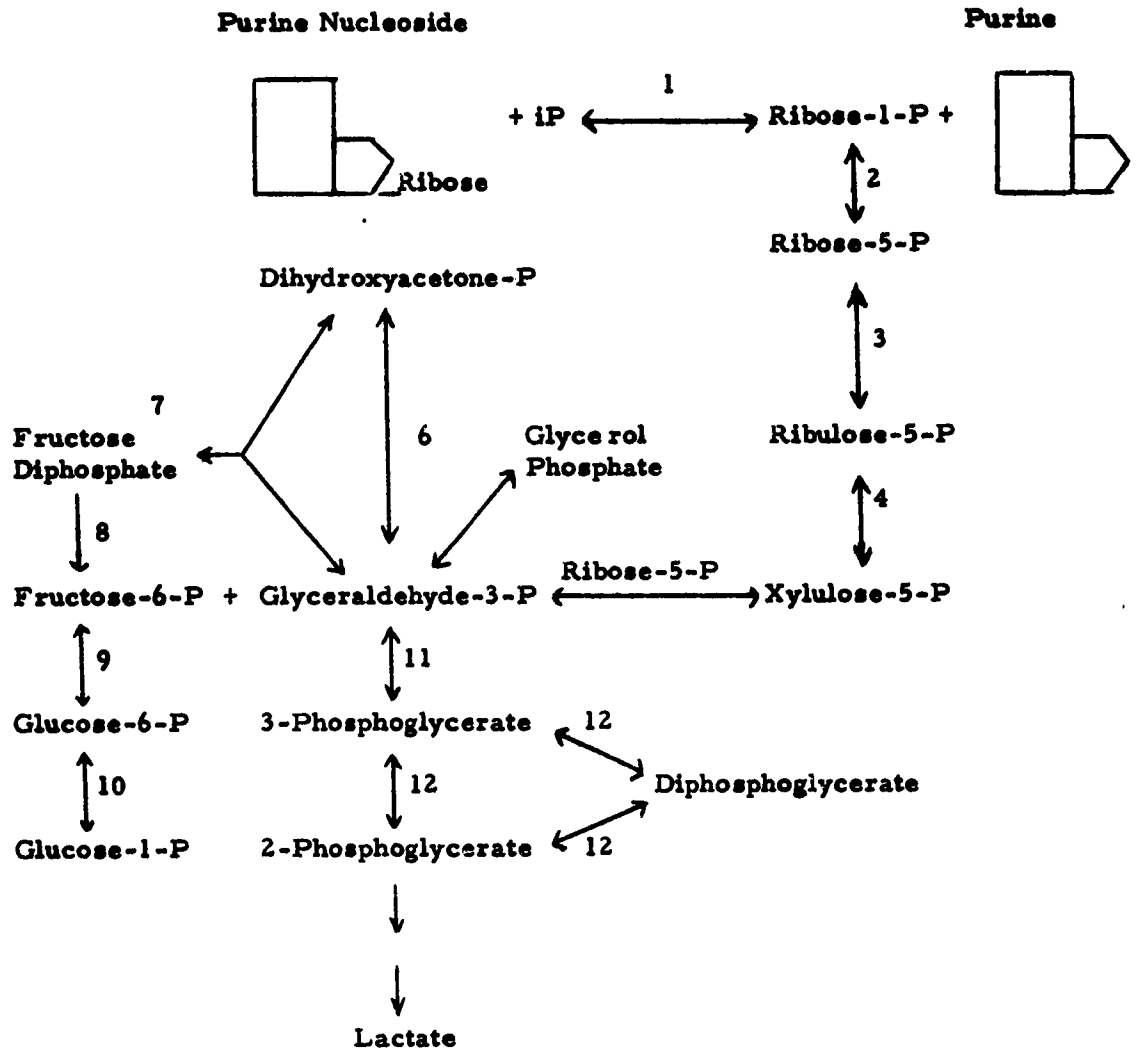
Fig. 1. Diagrammatic representation of the metabolic reactions of purine nucleosides in erythrocytes. The enzymes involved are: (1) nucleoside phosphorylase; (2) phosphoribomutase; (3) phosphoriboisomerase; (4) phosphoketopentosepimerase; (5) transketolase; (6) triosephosphate isomerase; (7) aldolase; (8) fructose diphosphatase; (9) phosphoglucoisomerase; (10) phosphoglucomutase; (11) triosephosphate dehydrogenase; (12) phosphoglyceric mutase.
