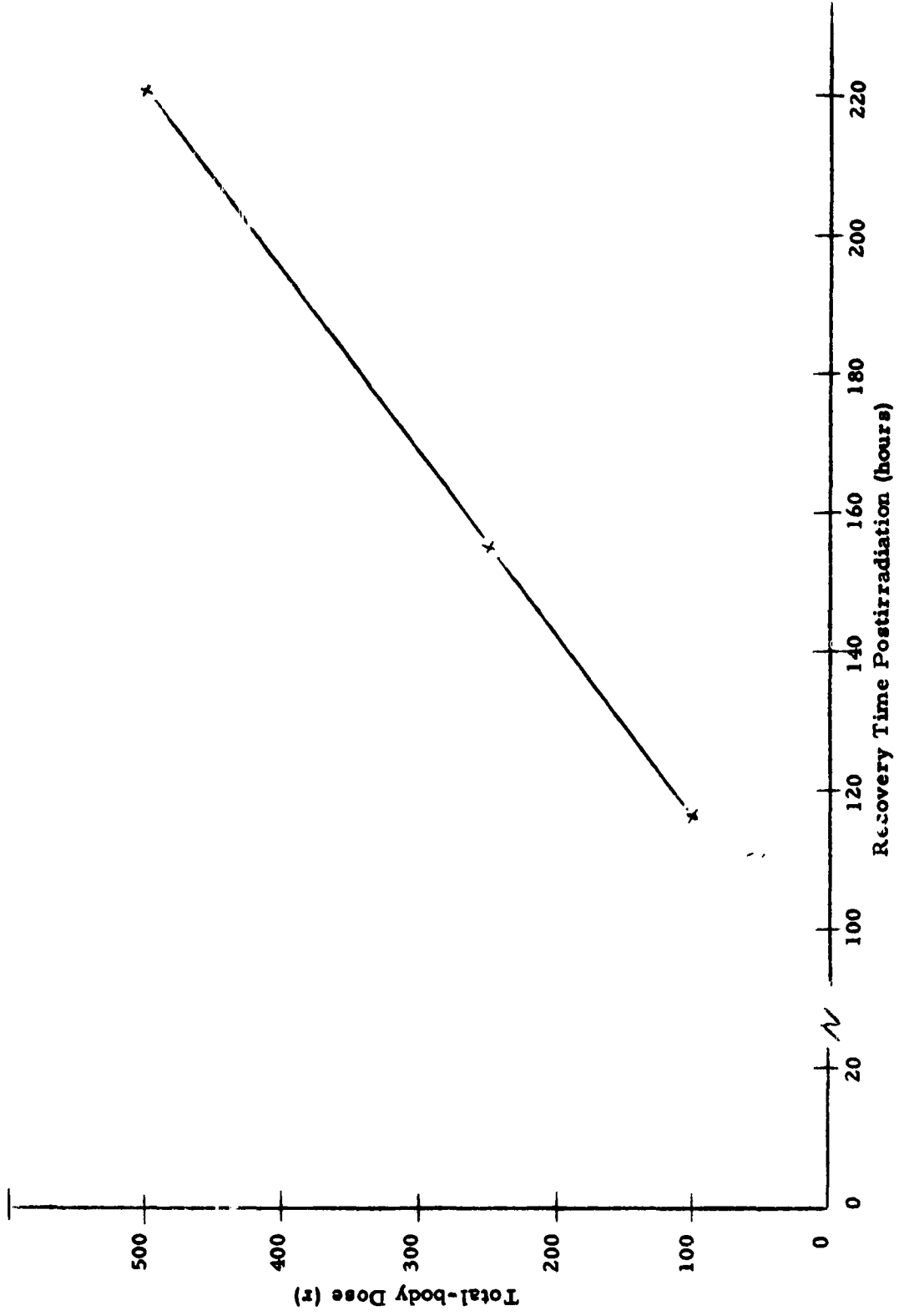
Fig. 4. Recovery of Rat Erythrocyte Nucleoside Phosphorylase Activity
