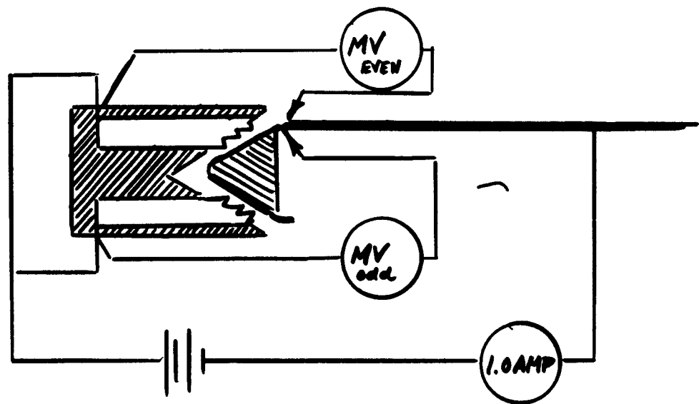
TEST CIRCUIT
