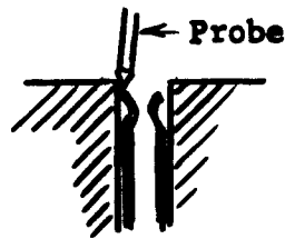
Contact finger
