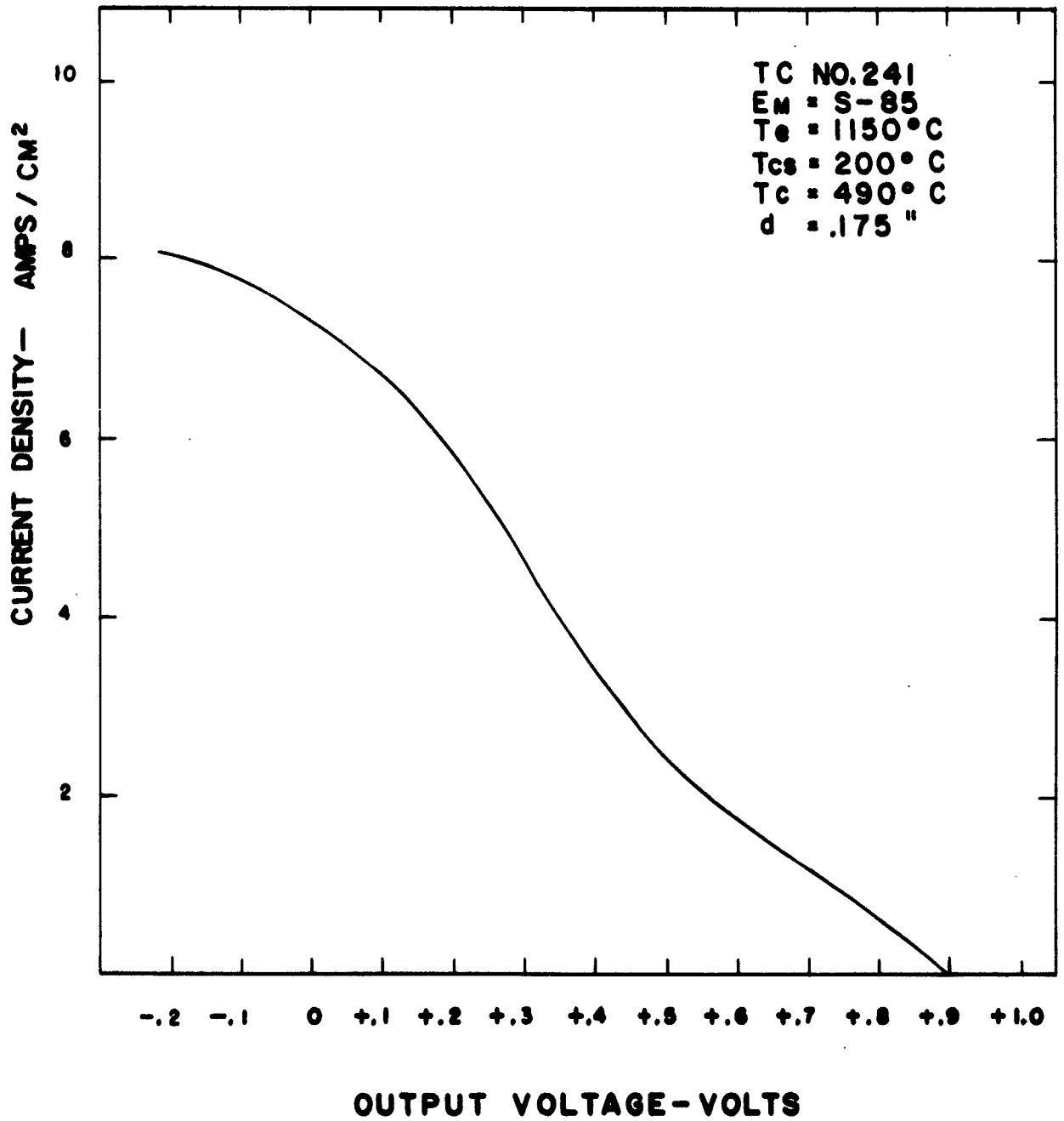
FIGURE 21 CURRENT DENSITY VS OUTPUT VOLTAGE
