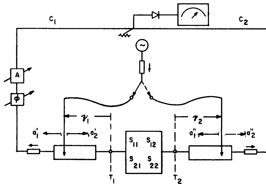
Fig. 7 Reversed bridge
