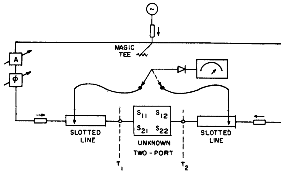
Fig. 6 Forward bridge
