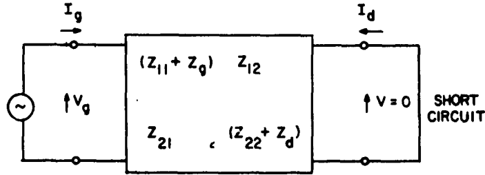
Fig. 4 Two-port incorporating generator and detector impedances
