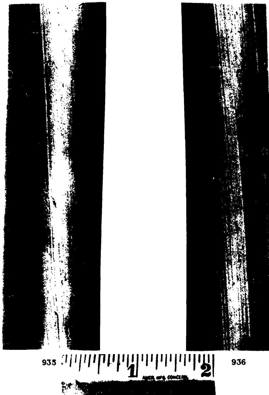
Figure 23 - Closeup of Extrusion Surfaces. Bars were Sandblasted to Remove Lubricant and Sil-O-Cel.
