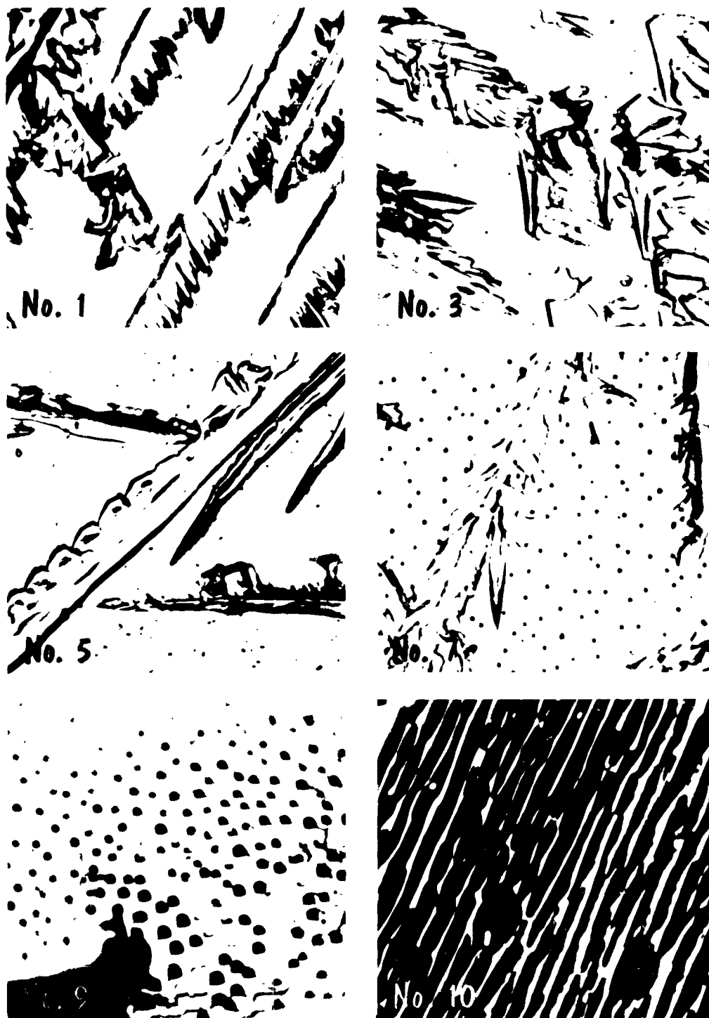
FIGURE 1 - Fracture Rating Scale for Carbon-Deoxidized Arc-Cast Molybdenum. All Fractographs X2000.
