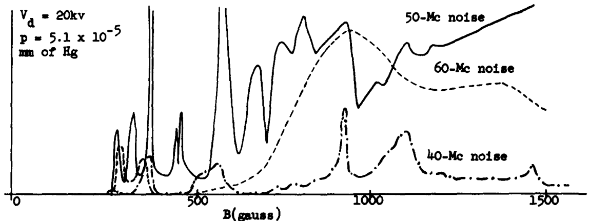
Fig. 14.--Noise at tungsten filament for particular frequencies ( 5.1 \times 10^{-5} mm of Hg, SS-2.4).
