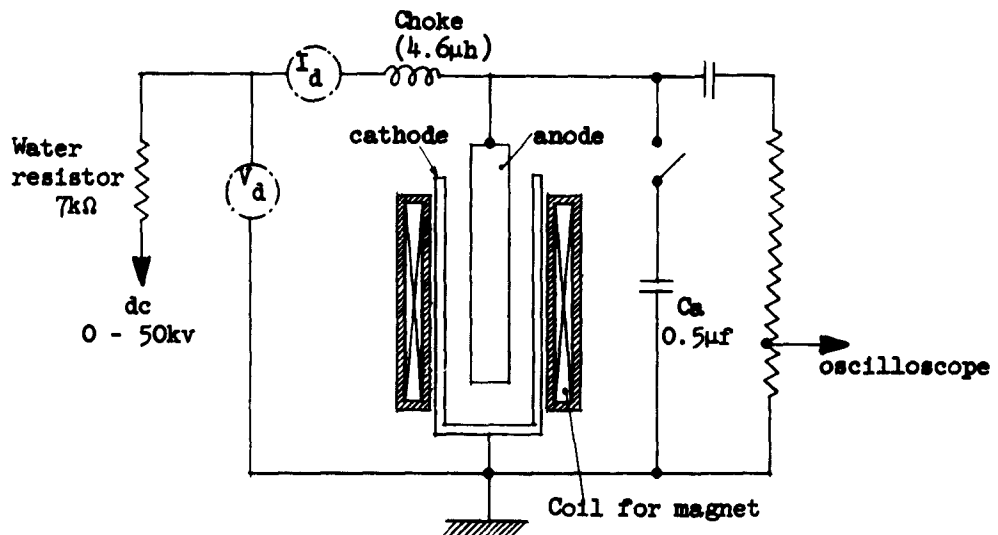
Fig. 1.--Schematic of experimental equipment.
