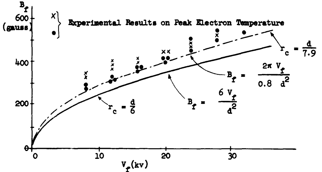
Fig. 26.--Optimum relation between V_f and B_f for magnetron action.
