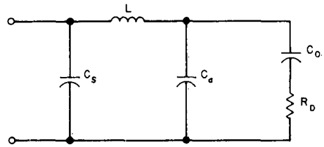
FIGURE E-1. EQUIVALENT CIRCUIT OF UNPUMPED VARACTOR
