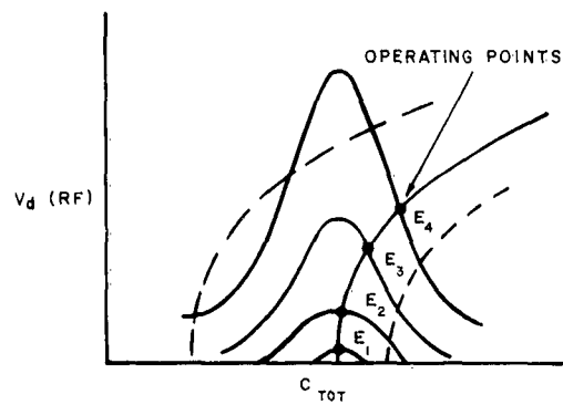
B. RESPONSE OF RESONANT CIRCUIT AND RESULTANT OPERATING POINTS
