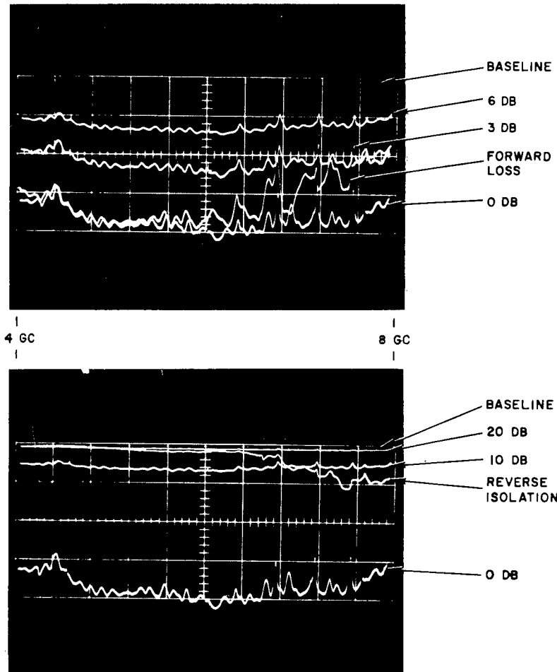
FIGURE 10. PERFORMANCE OF MATCHED BENDIX C-BAND CIRCULATOR WITH MODIFIED CENTER CONDUCTOR VS FREQUENCY
