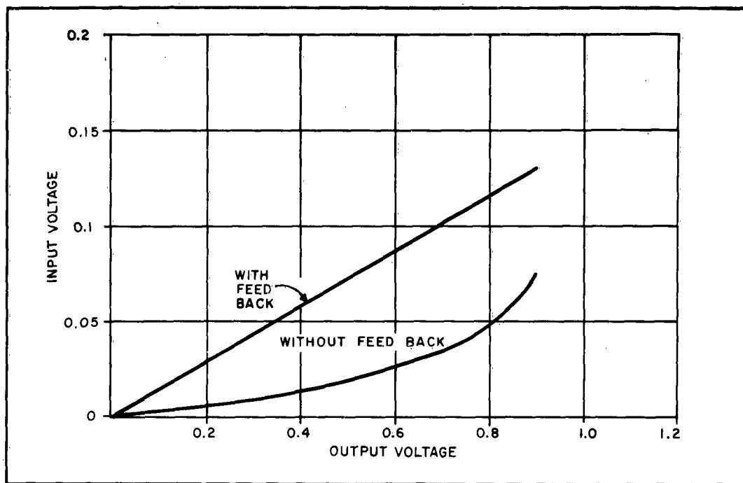
Figure 15. Amplifier Linearity
