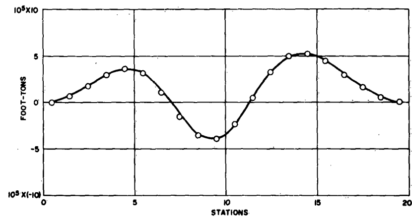
Figure 4c - 4-Noded Mode
