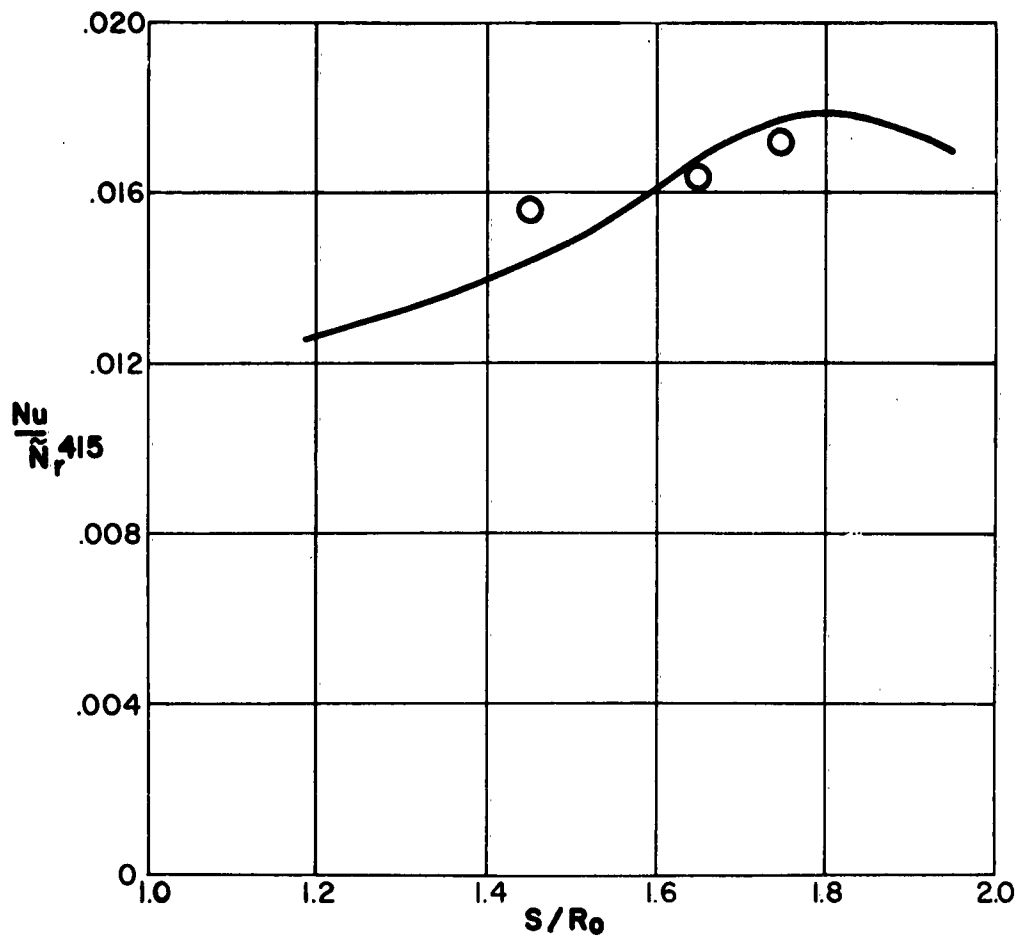
Fig. 10a. Nu/\tilde{N}_r^{1/5} vs. \bar{S} - \theta = 20^\circ
