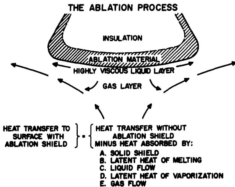
Fig. 2 Diagram showing Ablation Process
