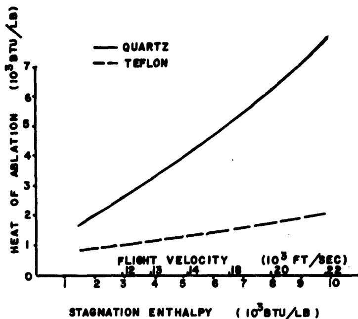
Fig. 3 Estimates of the heat of ablation for quartz and teflon. Subjected to turbulent heating.
