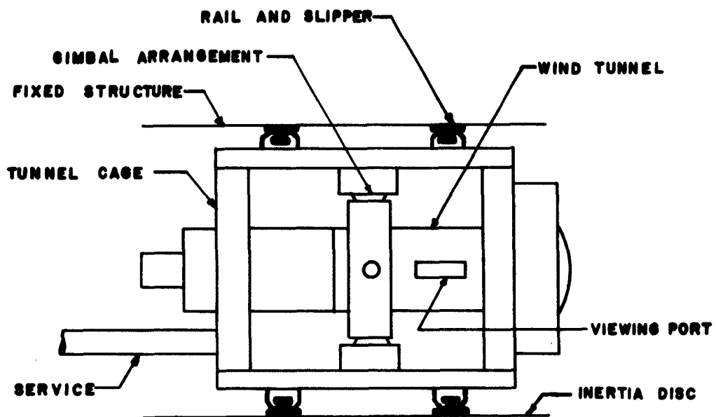
Fig. 15 Wind tunnel carriage and track arrangement
