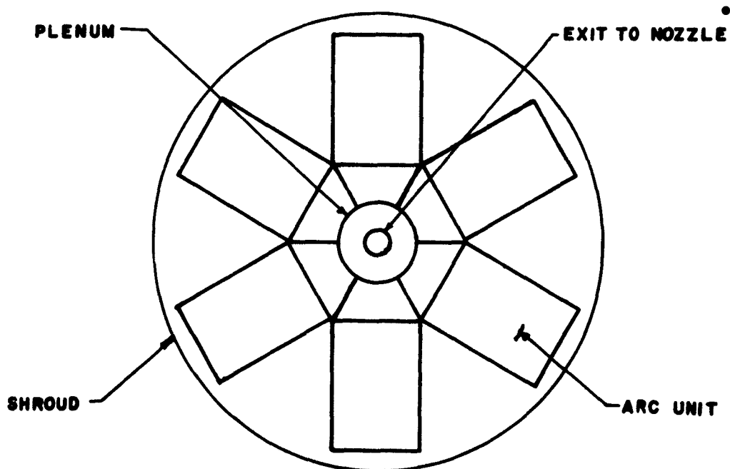
Fig. 12 Radial ARC Arrangement
