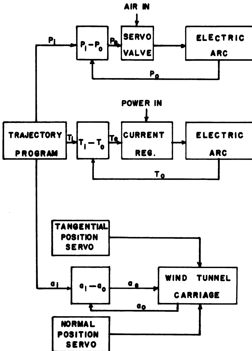
Fig. 20 Diagram for combined pressure, temperature and acceleration control systems
