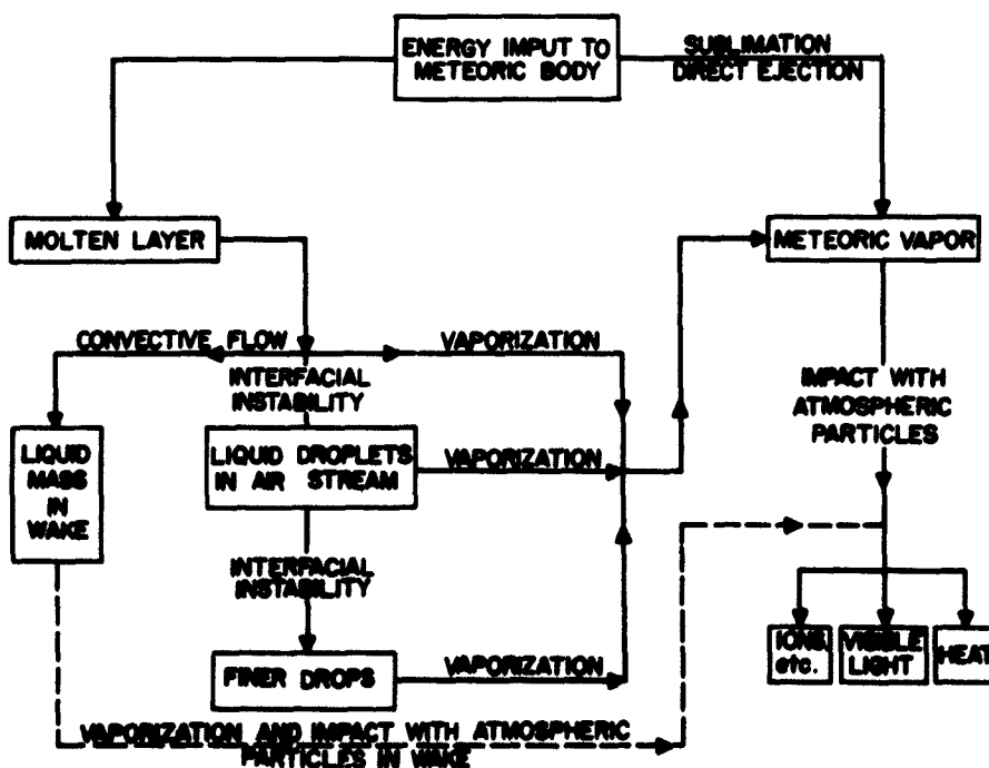
Fig. 4 Mechanisms of meteoric ablation. Courtesy Sin-I Cheng
