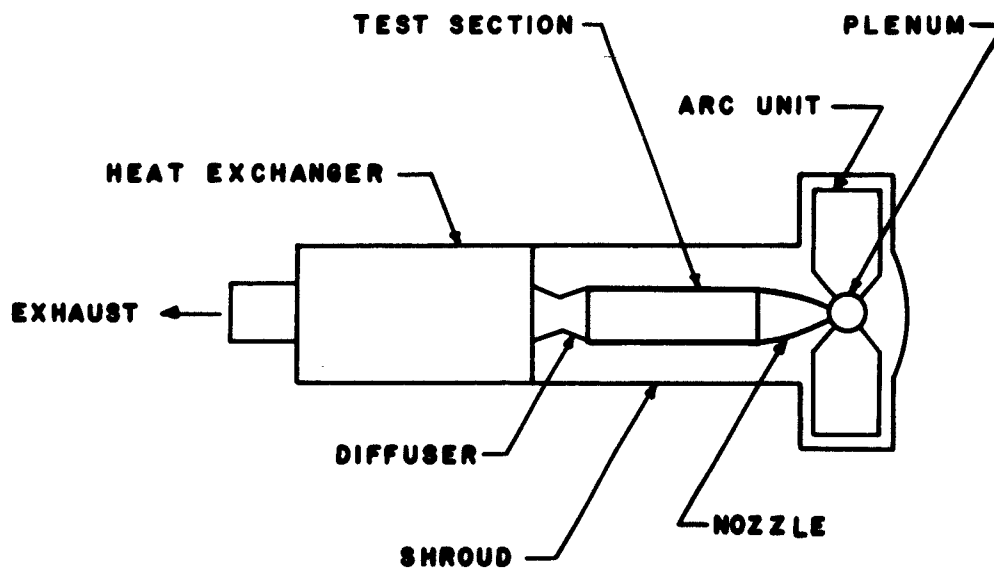
Fig. 14 Arrangement of wind tunnel components
