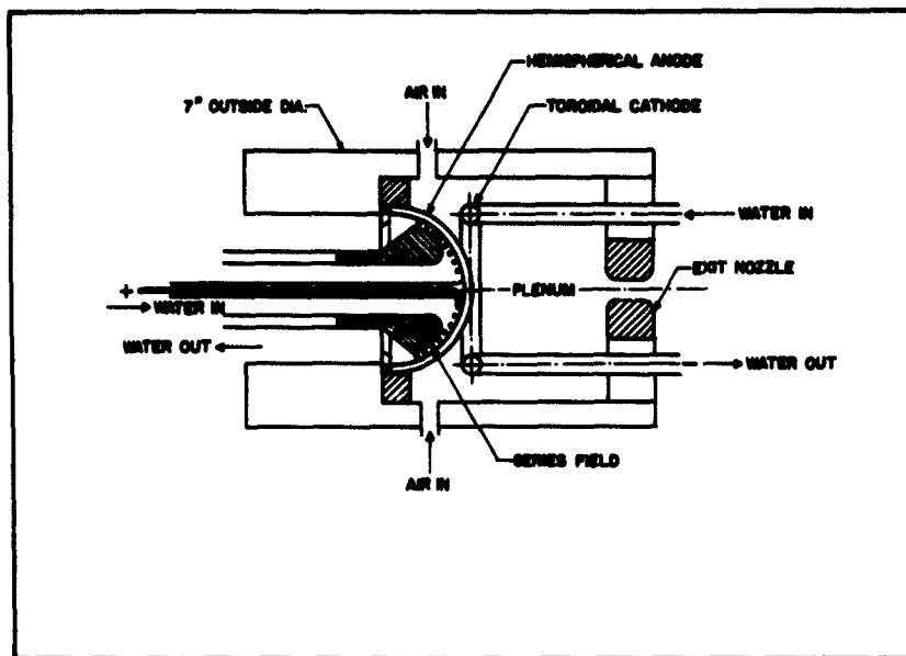
Fig. 11 Prototype A/C ARC Unit
