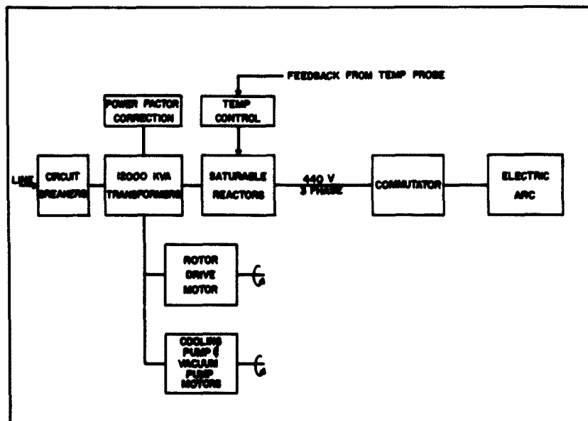
Fig. 17 Electrical Power System
