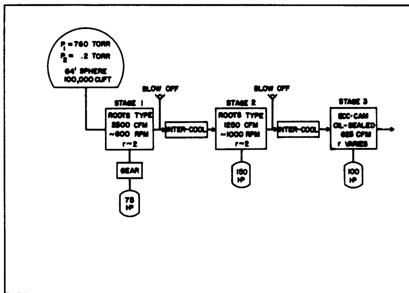
Fig. 19 Vacuum System
