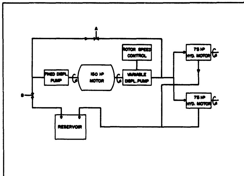
Fig. 16 Hydraulic System
