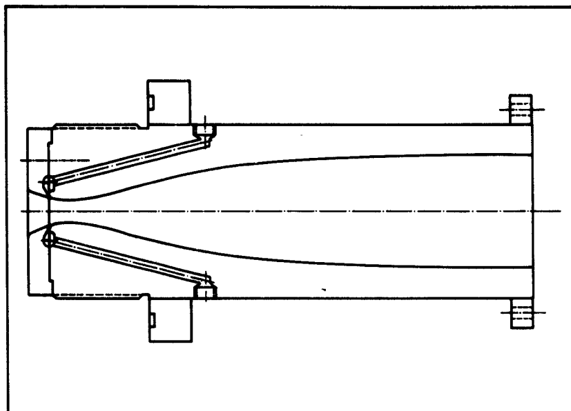
Fig. 13 Cross section of mach 5 nozzle showing injection cooling
