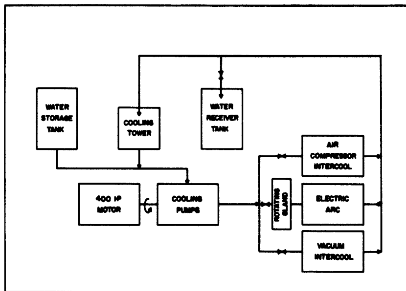
Fig. 18 Cooling System
