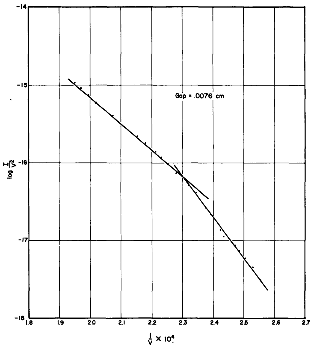
Figure 9.2. Fowler-Nordheim Plot.
