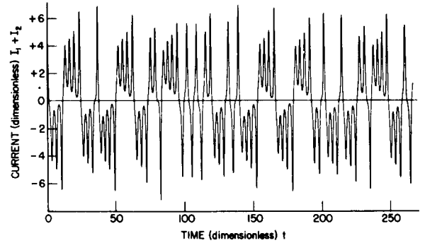
Fig. 7 - Expanded scale of current sum for P = 1.000 (see Fig. 6(b)) to illustrate typical ripple content. Initial conditions: I_1 = 3.000 , I_2 = 1.914 , \Omega_1 = 4.000 , and \Omega_2 = 0.000 (slightly different value than that of Fig. 6(b)).
