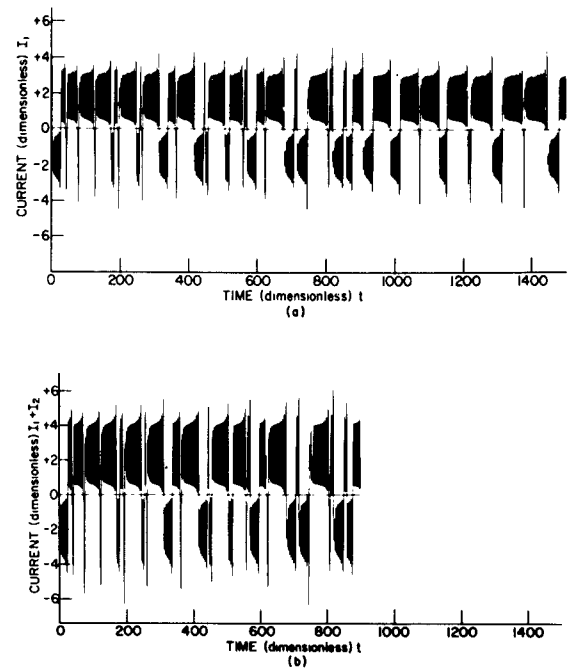
Fig. 10 - Simultaneous recording of (a) the individual current I_1 and (b) the current sum I_1 + I_2 , both for P = 0.600 and the initial conditions: I_1 = 3.000 , I_2 = 1.914 , \Omega_1 = 4.000 , and \Omega_2 = 0.037 .
