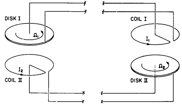
Fig. 2 - Rikitake-type, two-disk, mutually excited dynamo model. The break in the drawing serves to indicate that the individual sections, left and right, are sufficiently separated to exclude interaction except the mutual excitation.
