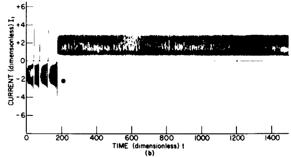
Fig. 8 - Individual current for P = 0.580 . (a) Initial conditions: I_1 = 3.000 , I_2 = 1.914 , \Omega_1 = 4.000 , and \Omega_2 = 0.037 ; (b) Initial conditions: I_1 = 3.000 , I_2 = 1.915 , \Omega_1 = 3.802 , and \Omega_2 = 0.0 .
