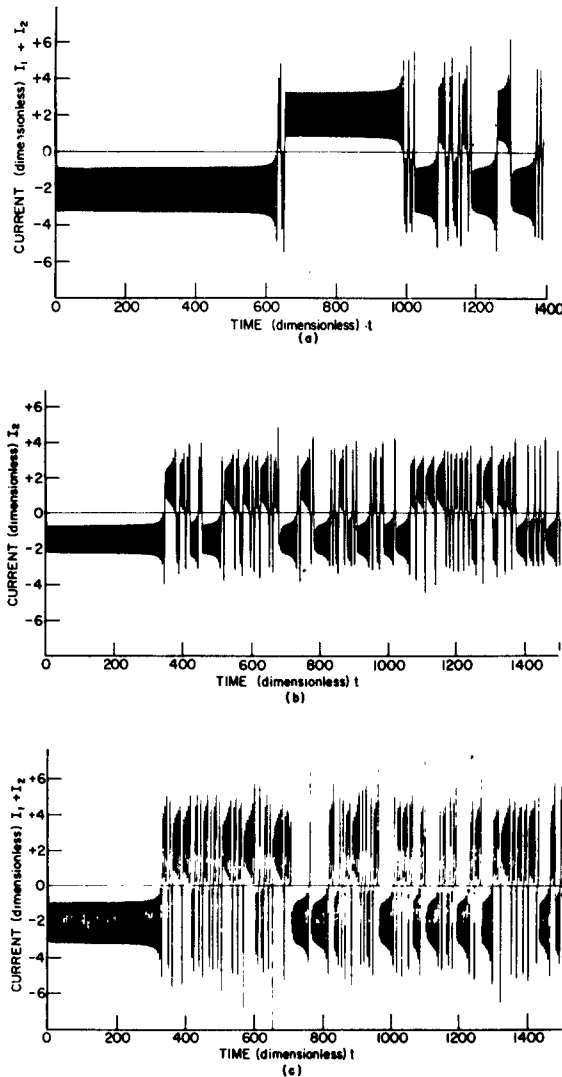
Fig. 9 - Three separate runs for P = 0.715 with initial conditions: I_1 = 3.300 , I_2 = 0.0 , \Omega_1 = 0.0 , and \Omega_2 = 2.400 . (a) illustrates a long duration in the upper polarity which occurred after three rapid-order reversals; (b) and (c) illustrate the general similarity of style for the more random reversals of the longer runs. (a) and (c) are for the current sum I_1 + I_2 , and (b) is for the individual current I_2 .
