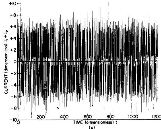
Fig. 6 - Current sum I_1 + I_2 for (a) P = 0.550 , (b) P = 1.000 , and (c) P = 1.400 . Initial conditions: I_1 = 3.000 , I_2 = 1.914 , \Omega_1 = 4.000 , and \Omega_2 = 0.037 .
