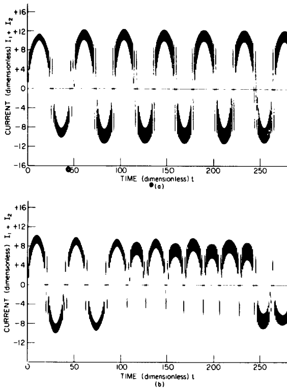
Fig. 11 - The current sum I_1 + I_2 for (a) K = 0.0 , F = 0.0075 , and Q = 0.0350 , and (b) K = 0.0025 , F = 0.0075 , and Q = 0.0850 . Initial conditions: I_1 = 3.000 , I_2 = 1.914 , \Omega_1 = 4.000 , and \Omega_2 = 0.0 .
