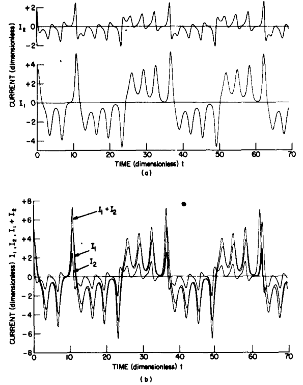
Fig. 4 - (a) Two individual currents I_1 and I_2 for P = 1.000 . Initial conditions: I_1 = 3.000 , I_2 = 1.914 , \Omega_1 = 4.000 , \Omega_2 = 0.037 . (b) Repeat runs of the same curves, and their sum I_1 + I_2 .
