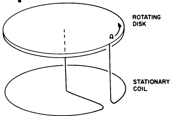
Fig. 1 - Bullard-type, self-excited, disk-dynamo model
