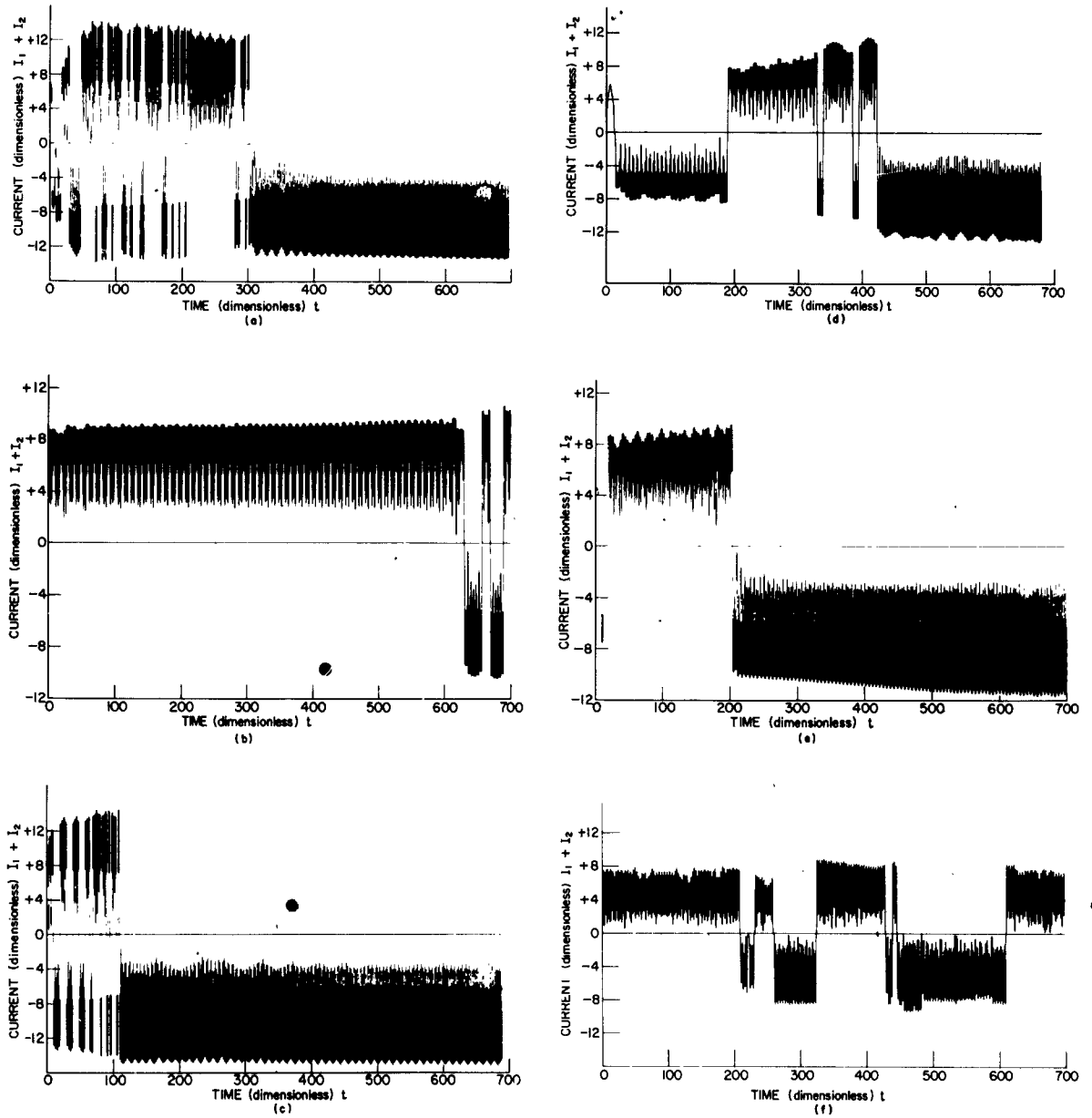
Fig. 12 - The current sum I_1 + I_2 for (a) K = 0.0002 , F = 0.0400 , and Q = 0.4000 , with initial conditions: I_1 = 6.6000 , I_2 = 0.0040 , \Omega_1 = 0.8000 , and \Omega_2 = 0.8000 ; (b) K = 1.5 \times 10^{-5} , F = 0.0210 , and Q = 0.4000 , with initial conditions: I_1 = 6.1800 , I_2 = 2.3800 , \Omega_1 = 0.5000 , and \Omega_2 = 1.9400 ; (c) K = 0.0001 , F = 0.0400 , and Q = 0.4000 , with initial conditions: I_1 = 5.6000 , I_2 = 4.4000 , \Omega_1 = 3.4400 , and \Omega_2 = 0.0 ; (d) K = 0.0001 , F = 0.0200 , and Q = 0.4000 , with initial conditions: I_1 = 1.4000 , I_2 = 0.7660 , \Omega_1 = 1.8000 , and \Omega_2 = 0.0 ; (e) K = 1 \times 10^{-5} , F = 0.0285 , and Q = 0.5000 , with initial conditions: I_1 = 0.7640 , I_2 = 1.2000 , \Omega_1 = 0.0040 , and \Omega_2 = 1.6000 ; and (f) K = 1 \times 10^{-5} , F = 0.1050 , and Q = 0.4000 , with initial conditions: I_1 = 2.7880 , I_2 = 4.2380 , \Omega_1 = 1.8080 , and \Omega_2 = 1.0440 .
