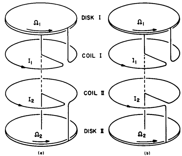
Fig. 3 - Axially stacked two-disk system. The dynamo in (b) differs from the dynamo in (a) in that the connections of Coil II have been reversed.
