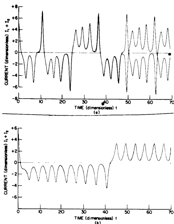
Fig. 5 - Two runs of the current sum I_1 + I_2 for (a) P = 1.000 and (b) P = 0.550 . Initial conditions: I_1 = 3.000 , I_2 = 1.914 , \Omega_1 = 4.000 , and \Omega_2 = 0.037 .
