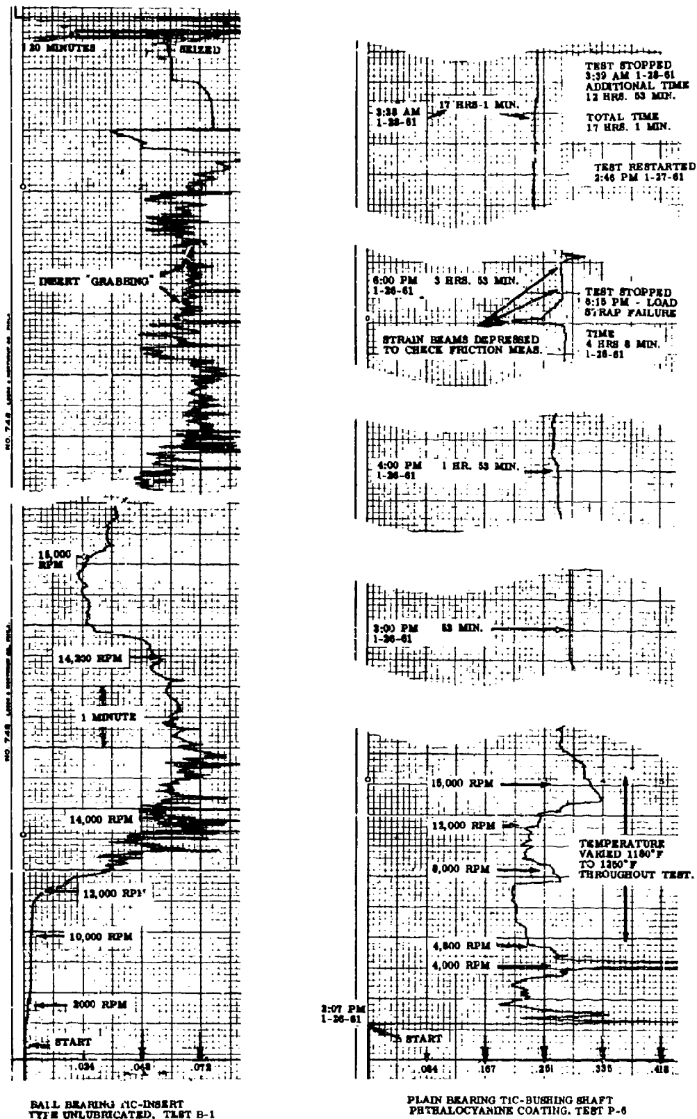
FIGURE 5 FRICTION CURVES FOR BALL AND PLAIN BEARINGS
