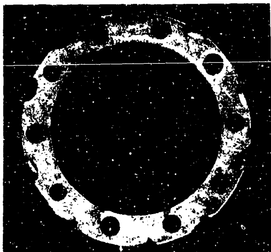
SLOTTED CAGE RING FOR ROLLER BEARING TEST R-4
