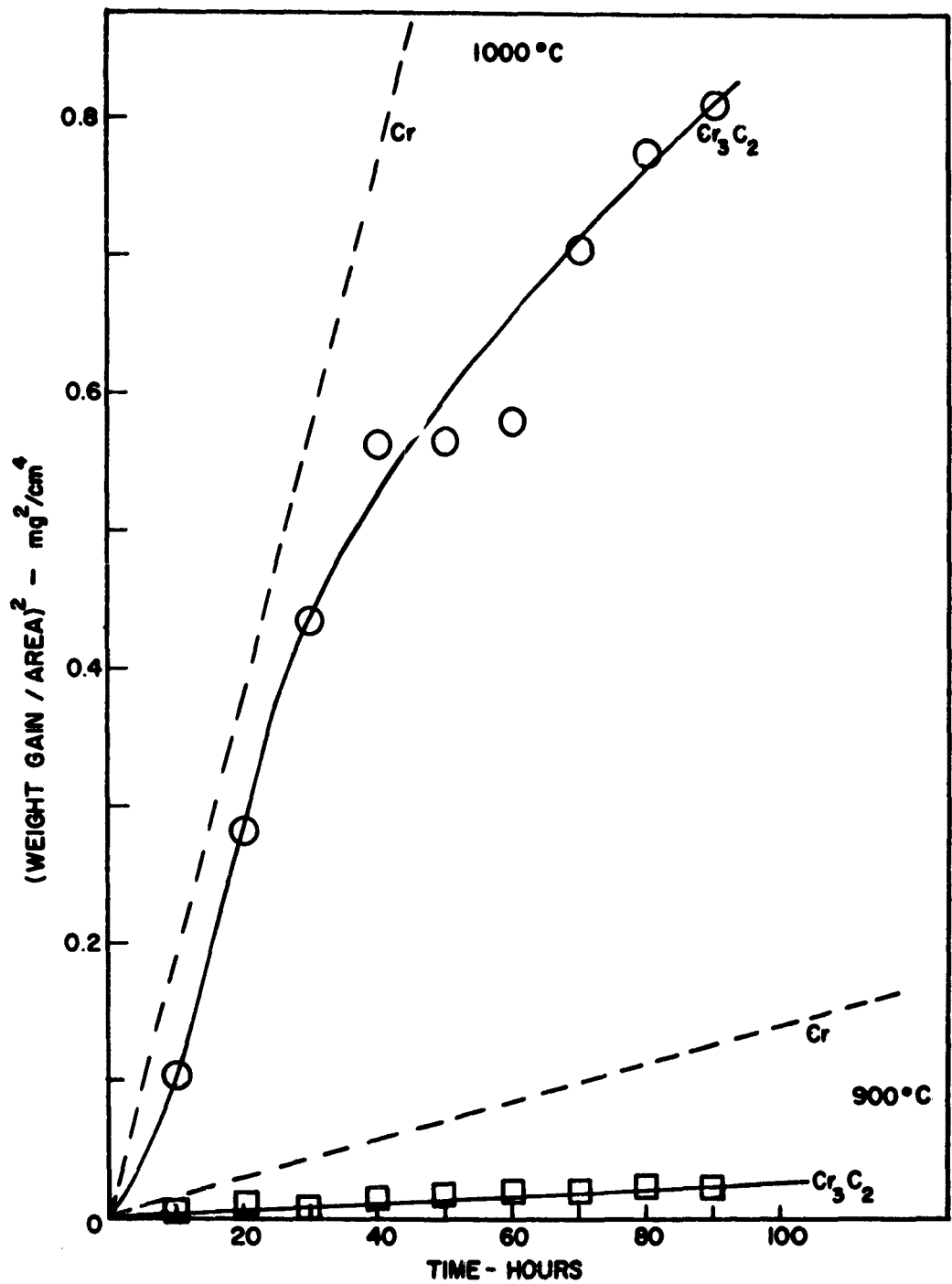
FIGURE II-11 PARABOLIC PLOT FOR OXIDATION OF Cr 3 C 2 & Cr IN OXYGEN
