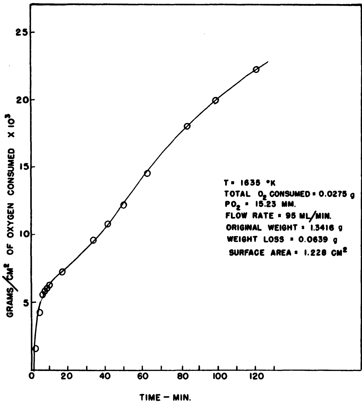
FIGURE IV-1 OXIDATION OF W 5 Si 3 (XI-20) AT 1635 °K
