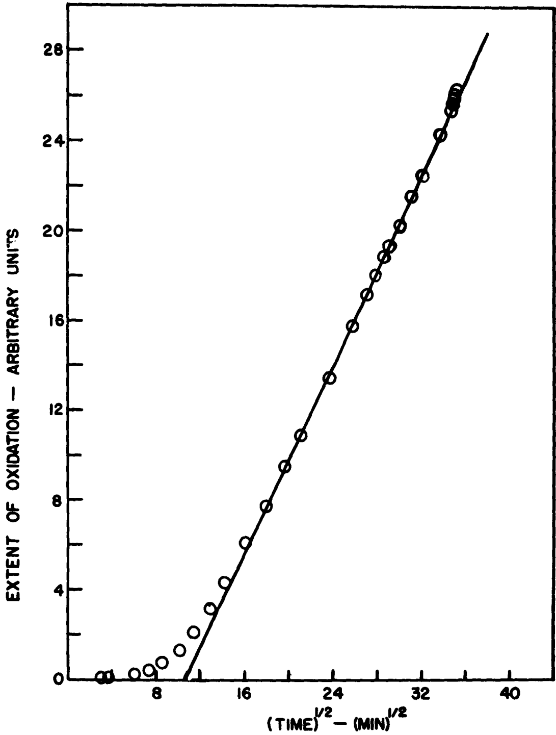
FIGURE II - 9 OXIDATION OF HfC, AT 2305 °K, P_{O_2} 4.2 TORR 49
