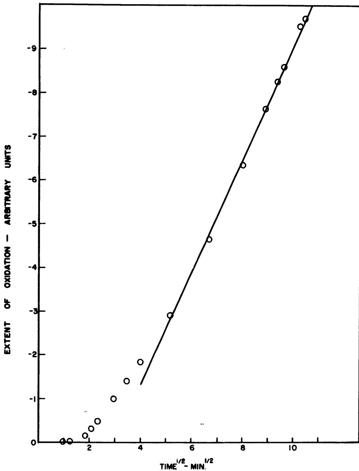
FIGURE II - 10 OXIDATION OF TaC, AT 2432°K, P_{O_2} 6.8 TORR
