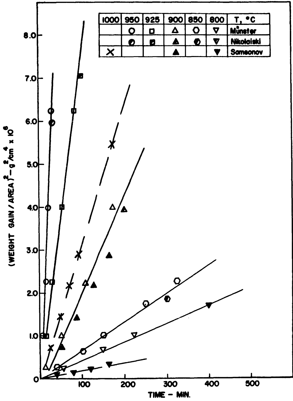
FIGURE II-1 OXIDATION OF TiC
