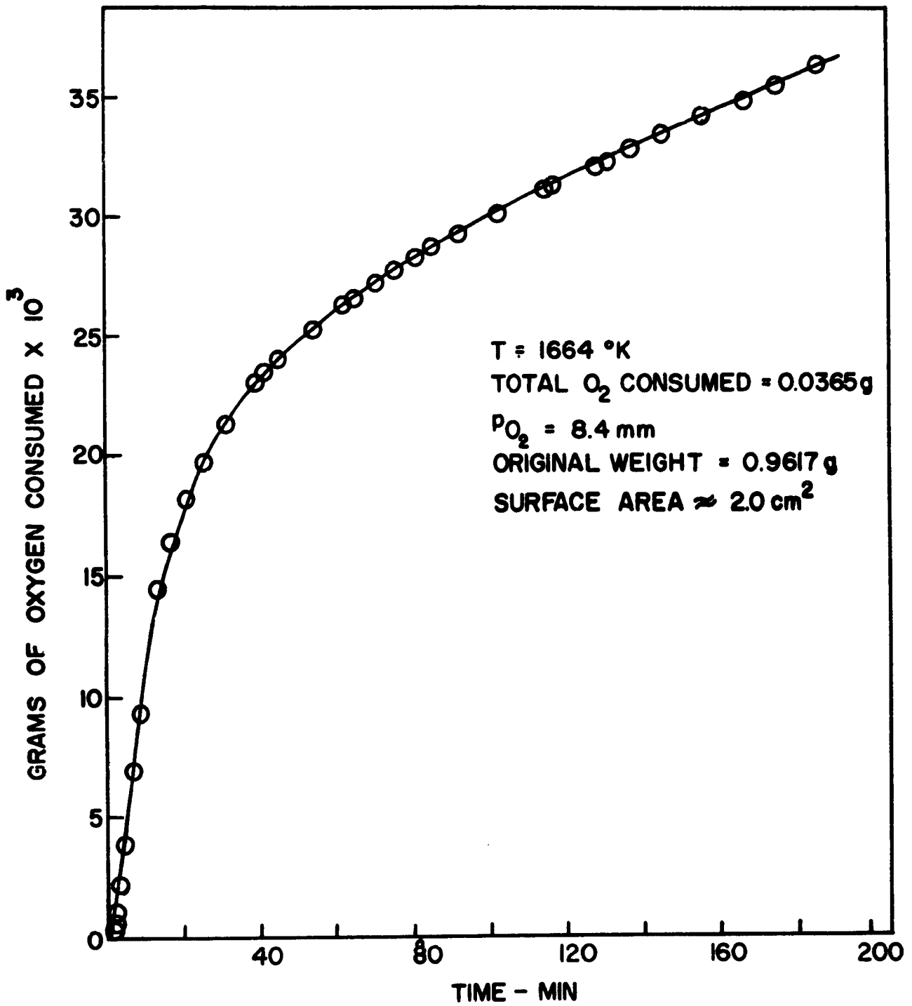
FIGURE IV - 10 OXIDATION OF Ta 2 Be 17 (XI-5I) AT 1664 °K 104
