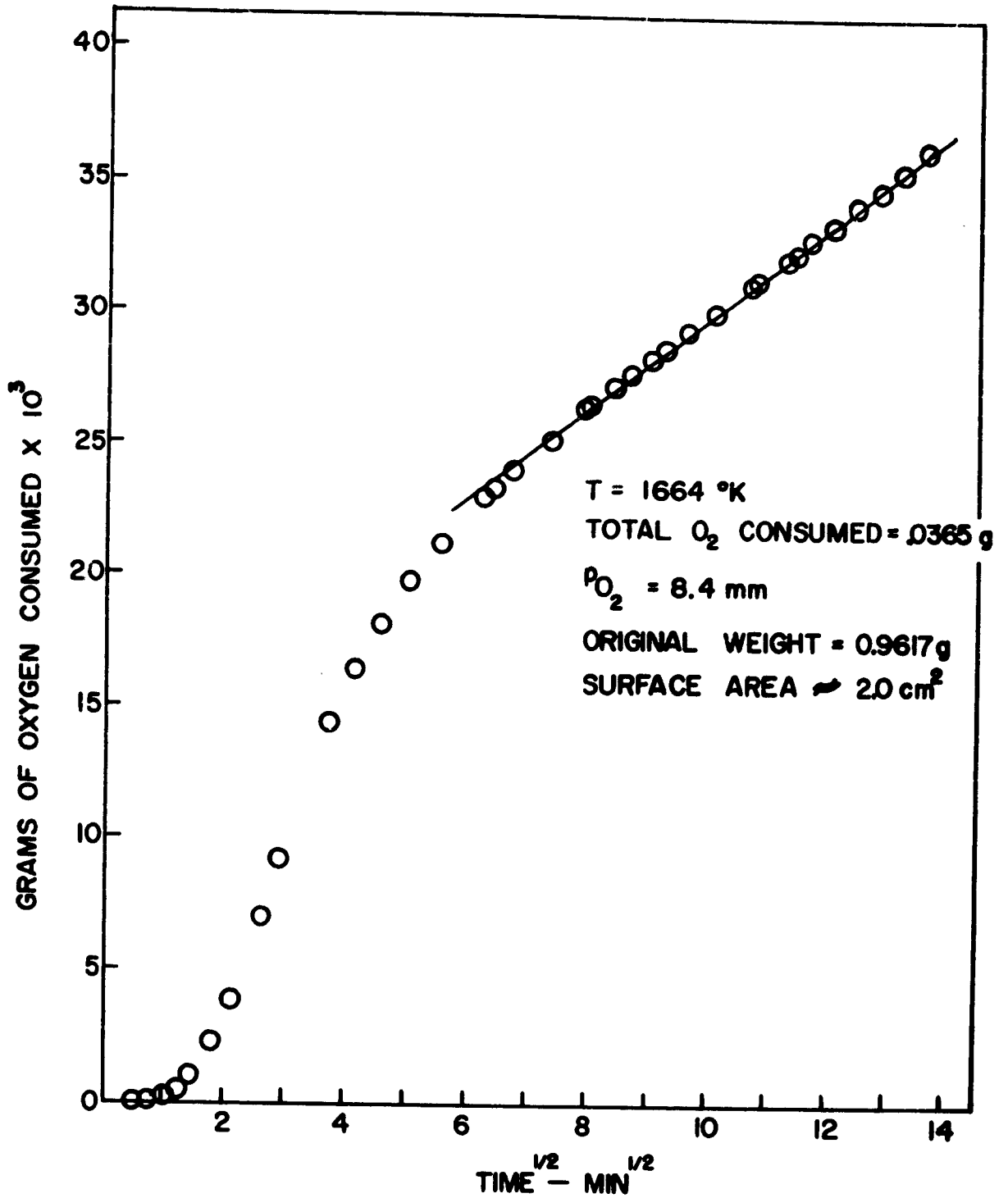
FIGURE IV - 11 OXIDATION OF \text{Ta}_2\text{Be}_{17} (XI-51) AT 1664 °K
