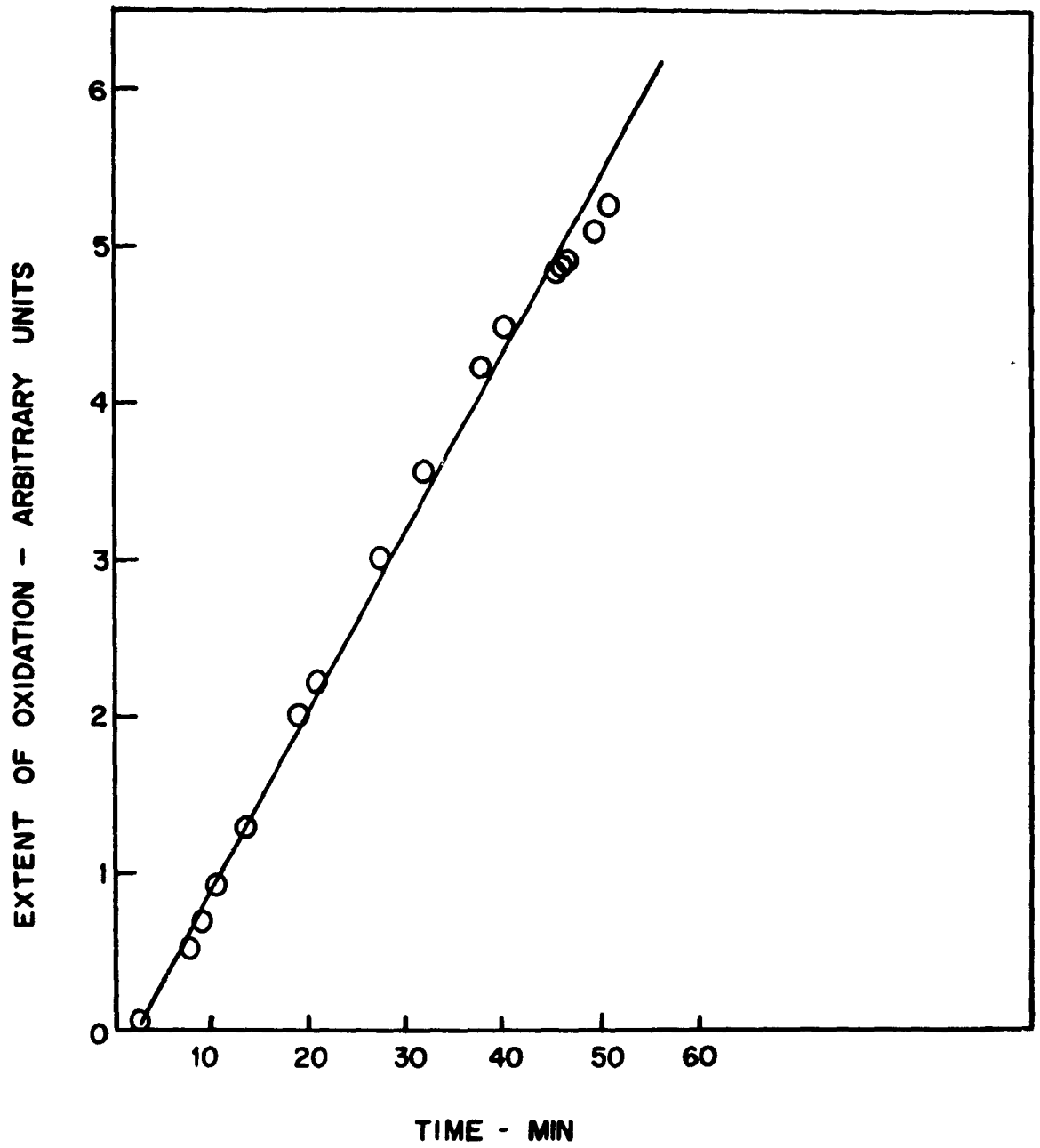
FIGURE II - 4 OXIDATION OF ZrC, AT 1126 °K, P_{O_2} 22.9 TORR
