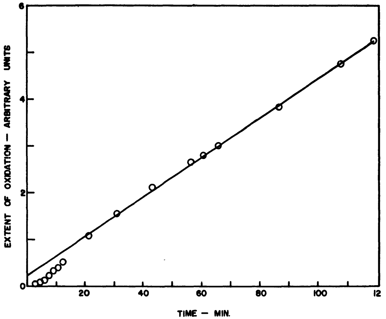
FIGURE II - 7 OXIDATION OF ZrC, AT 2165°K, P_{O_2} 8.9 TORR
