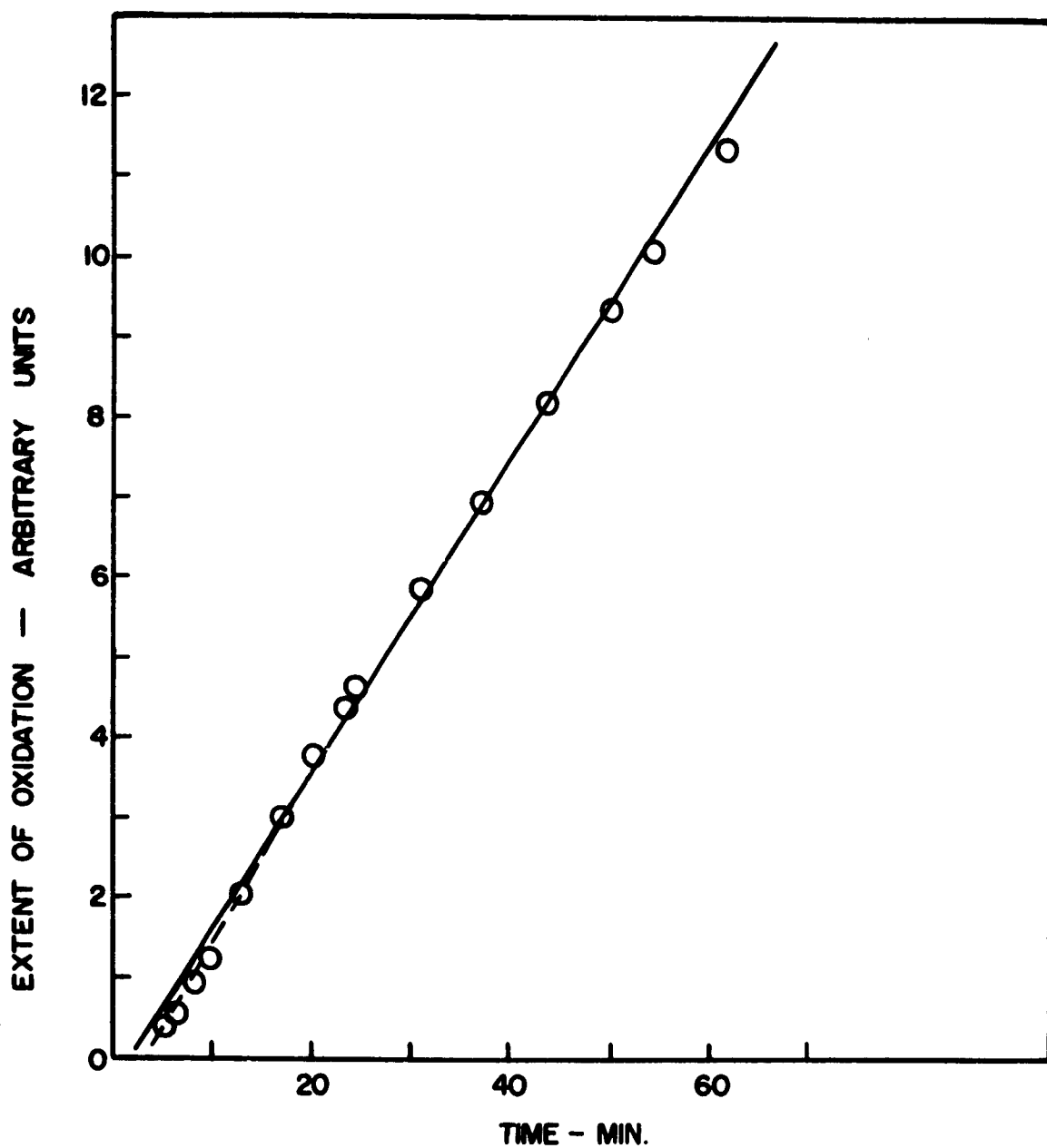
FIGURE II - 5 OXIDATION OF ZrC, AT 1559 °K, P_{O_2} 21.2 TORR
