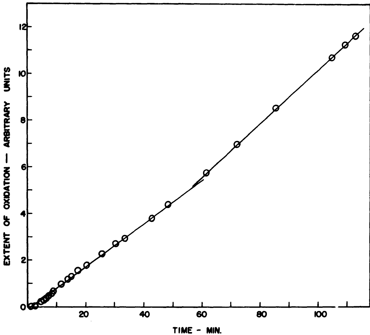
FIGURE II-6 OXIDATION OF ZrC, AT 1969 °K, P_{O_2} 25.9 TORR
