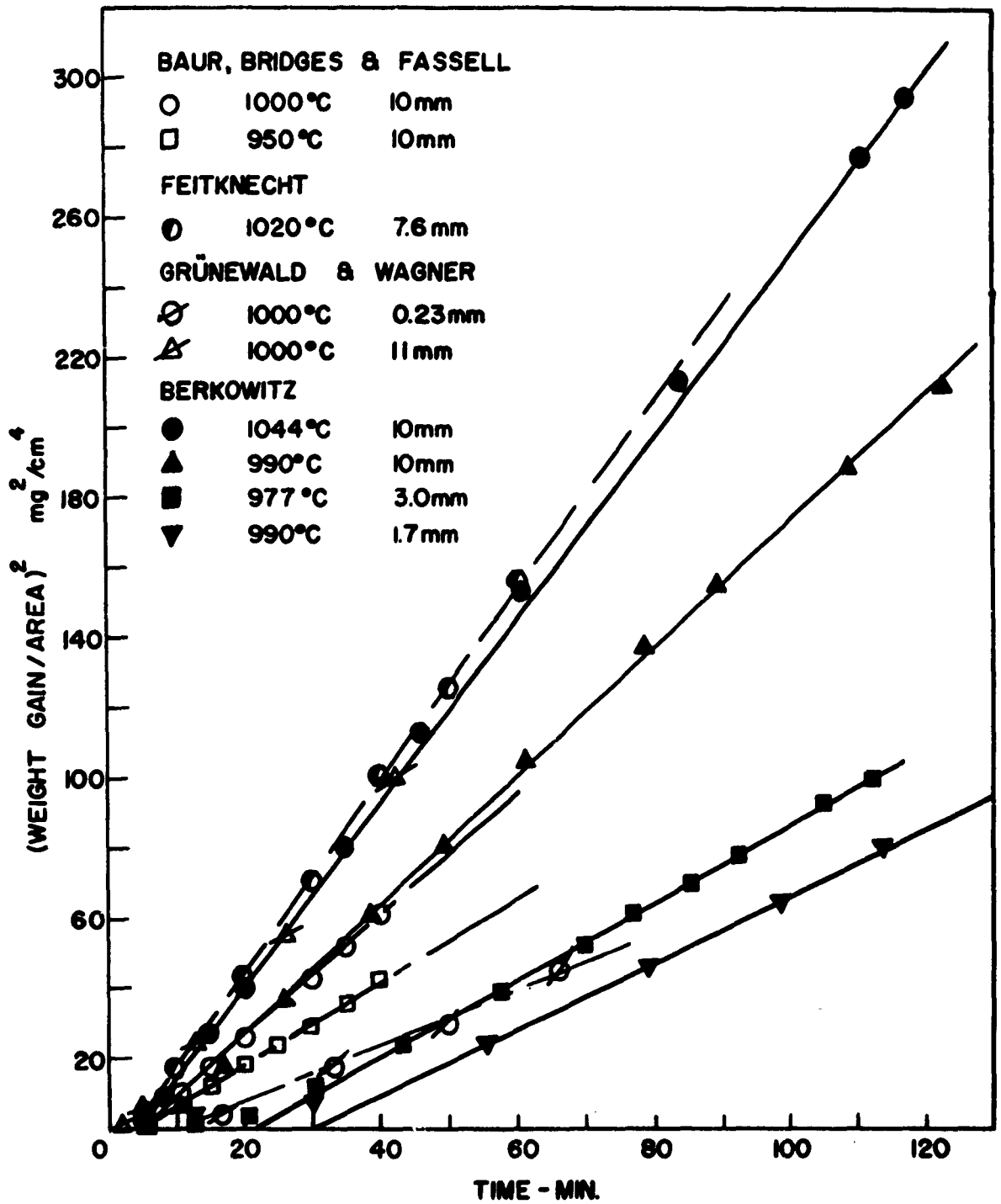
FIGURE I-5 PARABOLIC PLOT FOR THE OXIDATION OF Cu,
