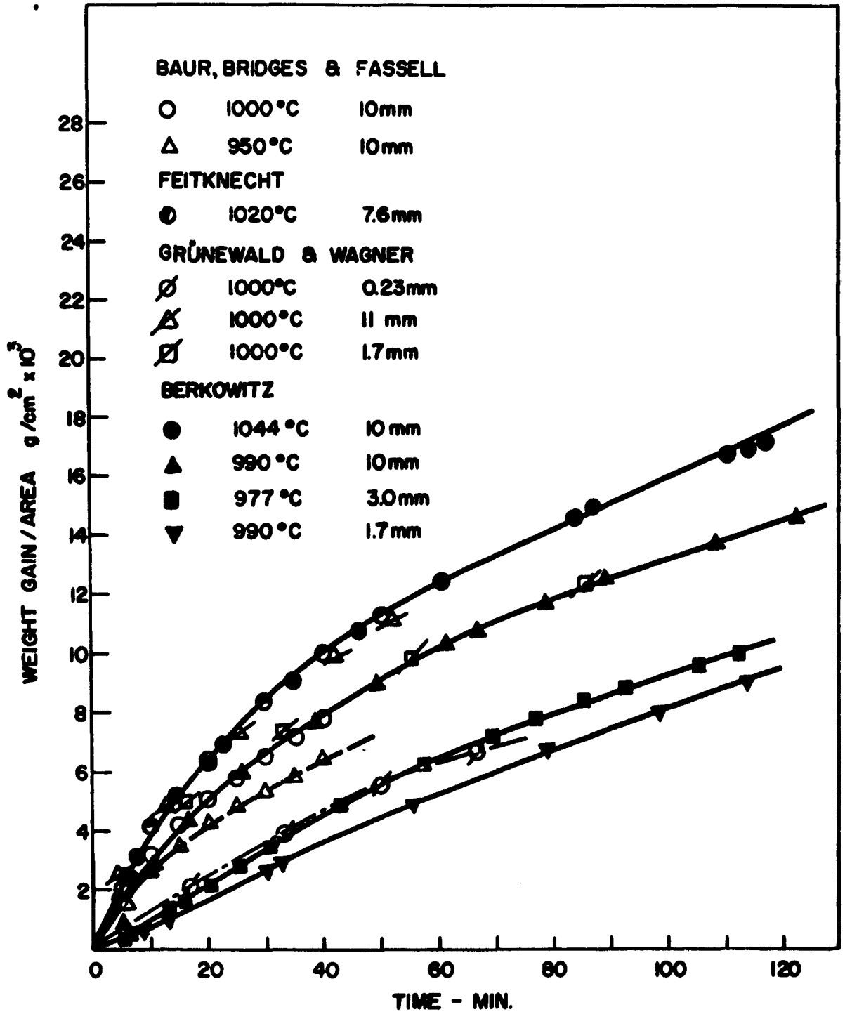
FIGURE I-4 TOTAL OXYGEN CONSUMPTION versus TIME FOR Cu
