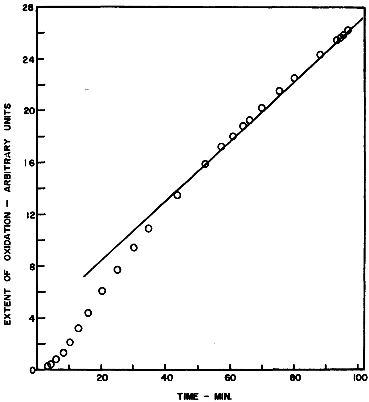
FIGURE II - 8 OXIDATION OF HfC, AT 2305 °K, P_{O_2} 4.2 TORR
