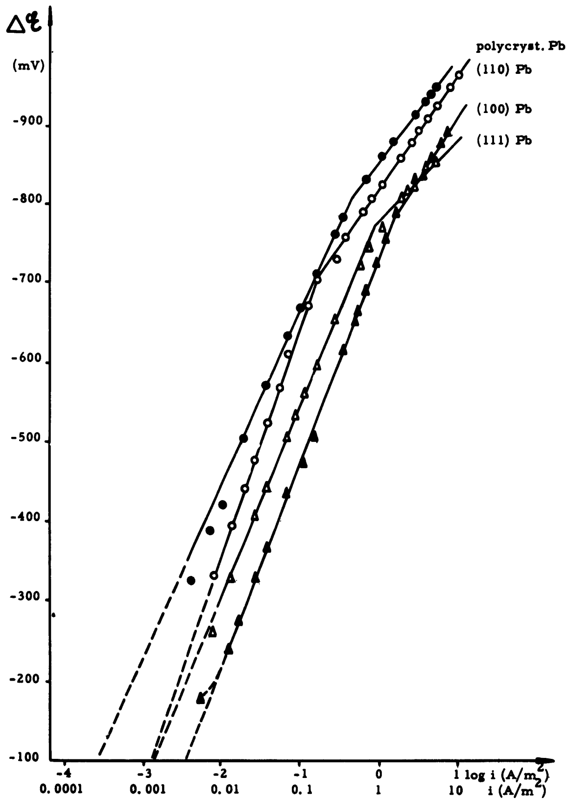
Fig. 10 - Behavior in dilute perchloric acid t = 25^\circ\text{C}
