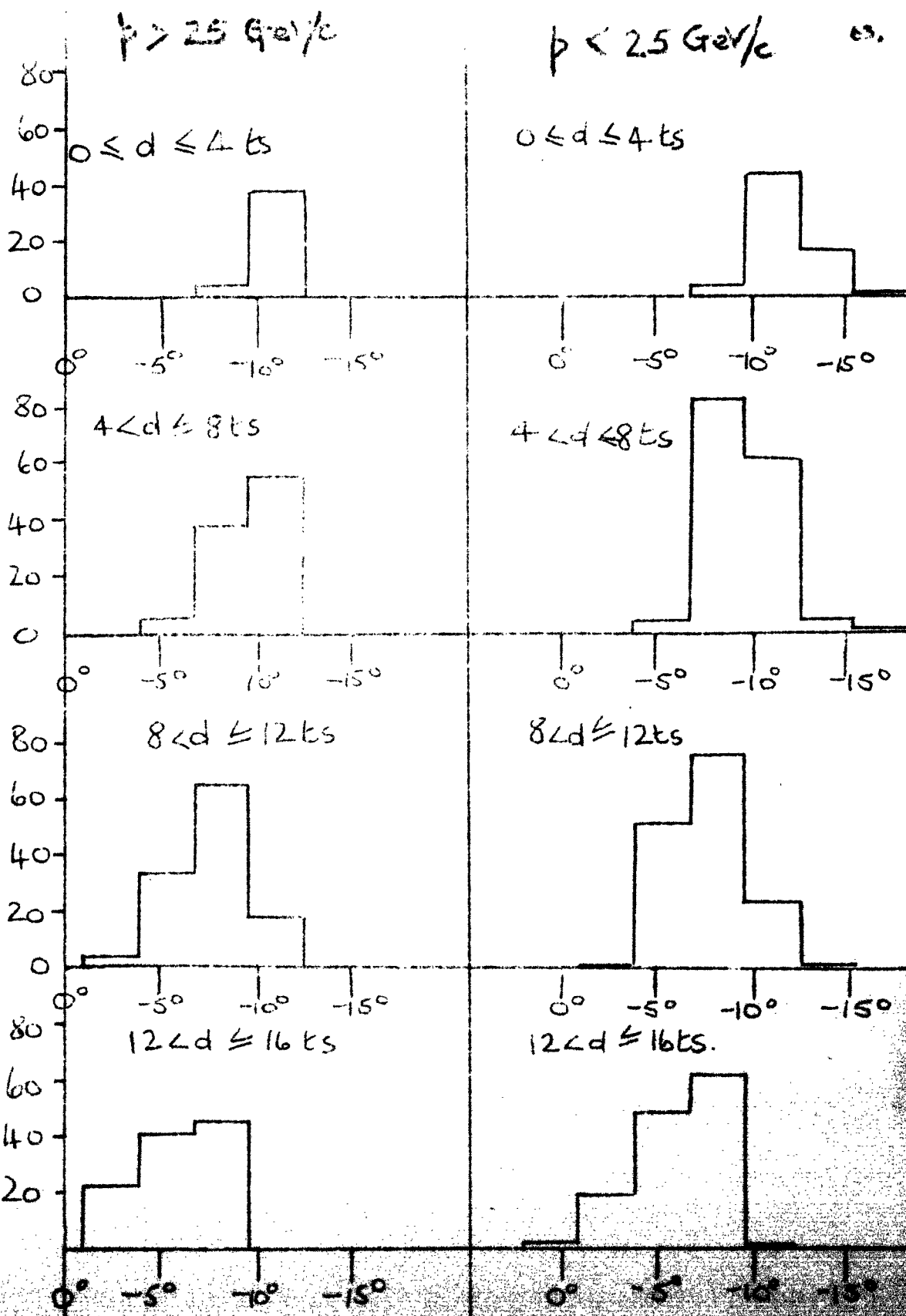
Fig 3.11 Angular distribution of particles at energies 2.5-9.0 GeV/c
