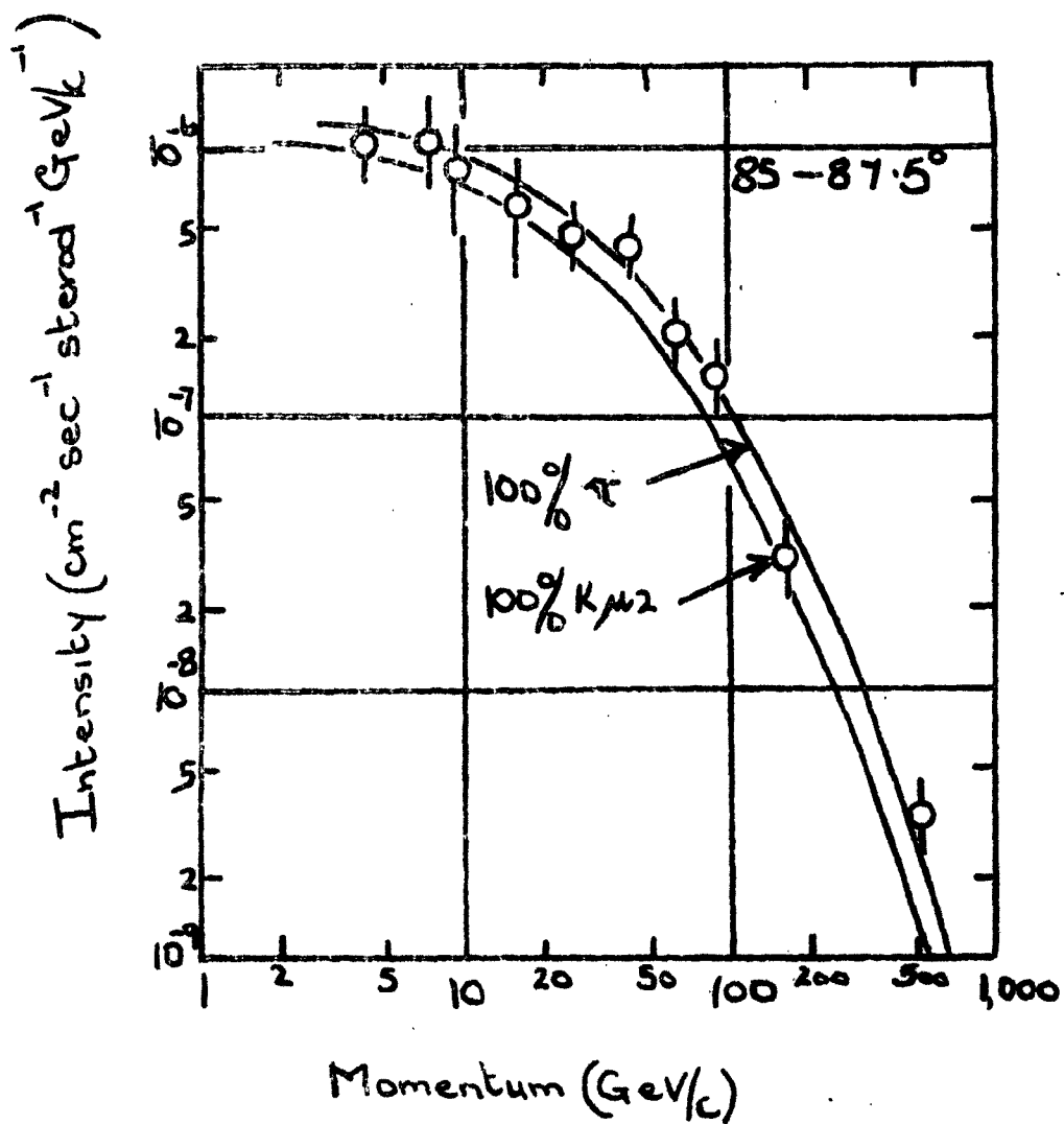
Fig 6.6 The Measured Momentum Spectrum in the range 85-87.5°
