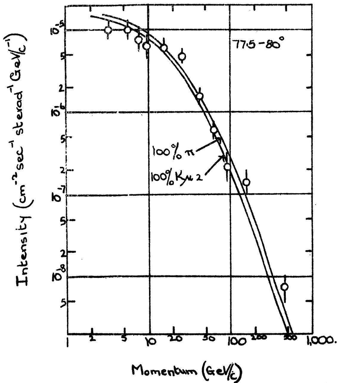
Fig 6.3 The Measured Momentum Spectrum in the range 77.5-80^\circ
