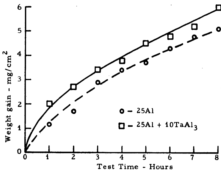
Fig. 5. Oxidation weight gains of Sn-Al coatings on Ta-10W in furnace tests at 2800°F. Samples were 0.010" x 1/2" x 3/4" and end lump was not removed.
