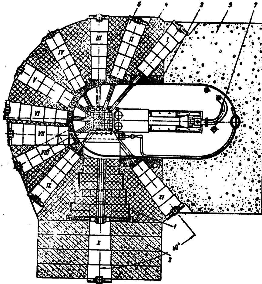
Fig. 4. Horizontal cross section of the reactor [1]
