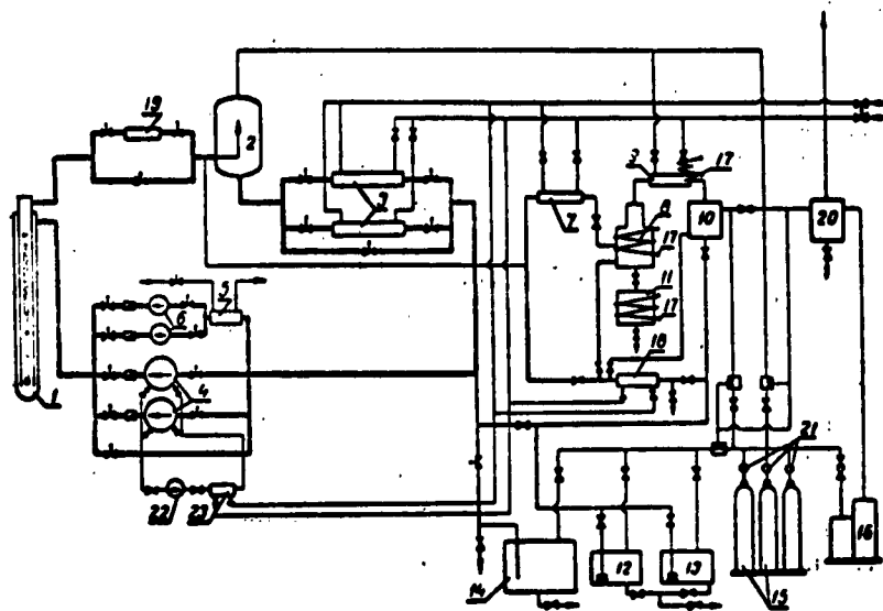
Fig. 14. Principal flow diagram of the experimental organic heat transfer loop of the Malyye Dubny reactor [19]
