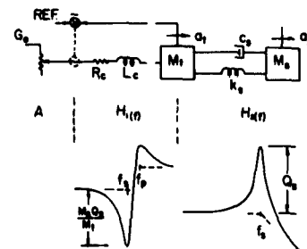
Fig. 2 - Schematic of vibration test system, simplified to retain only those elements necessary to compare vibration tests of differing types
