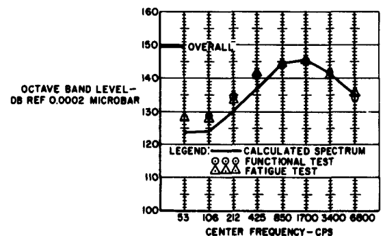
Fig. 13 - Synthesized noise spectra during functional and fatigue tests
