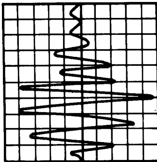
A. OUTPUT OF ACCELEROMETER NO. 1 (ON TABLE). SAME AS FIGURE 20 A EXCEPT PHOTOCELL FLASHBACK ERROR AT THE END OF THE WAVEFORM WAS ELIMINATED. SWEEP: 10-MILLISEC/DIV VERTICAL: 5-g/DIV
