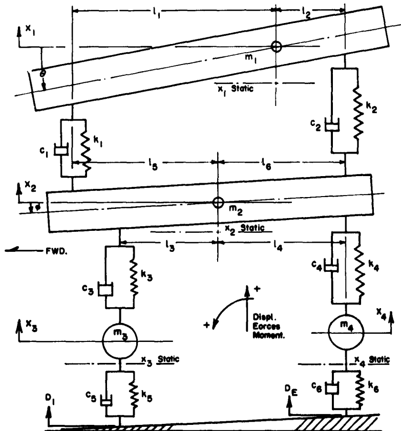
Fig. 16 - Idealized missile-transtainer system
