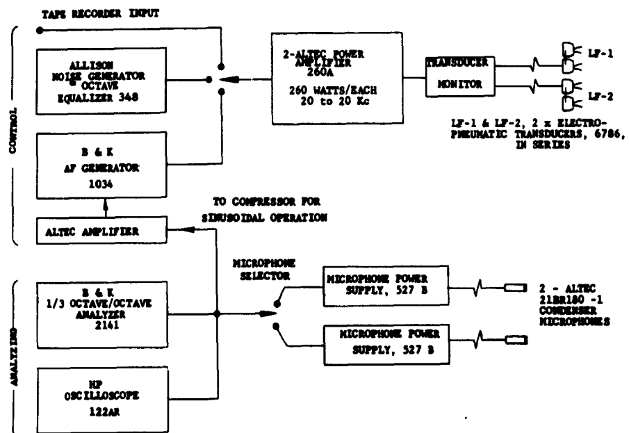
Fig. 7 - Control and analyzing equipment for sonic environmental system
