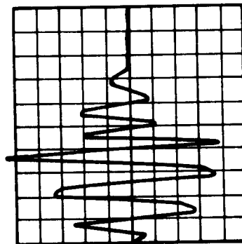
B. SWEEP: 250-MILLISEC (50-MILLISEC/DIV) VERTICAL: 40-g FULL SCALE (4 g/DIV)
