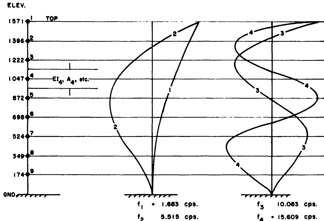
Fig. 11 - First stage umbilical tower flexural frequencies and mode shapes
