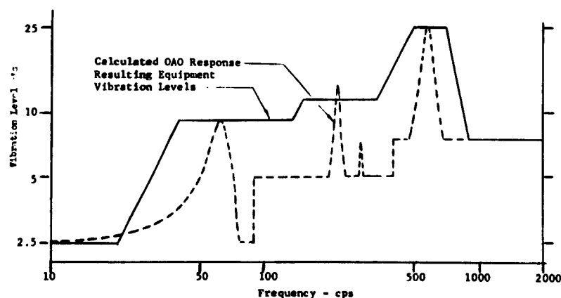
Fig. 3 - Results of vibration analysis
