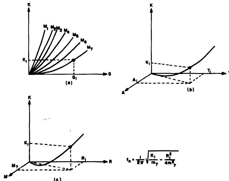
Fig. 5 - Procedure for selecting a package cushioning system
