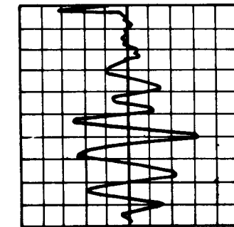
B. OUTPUT OF ACCELEROMETER NO. 2 (ON FIXTURE). SAME AS FIGURE 19 B EXCEPT 180^\circ OUT OF PHASE SWEEP: 10-MILLISEC/DIV VERTICAL: 5-g/DIV
