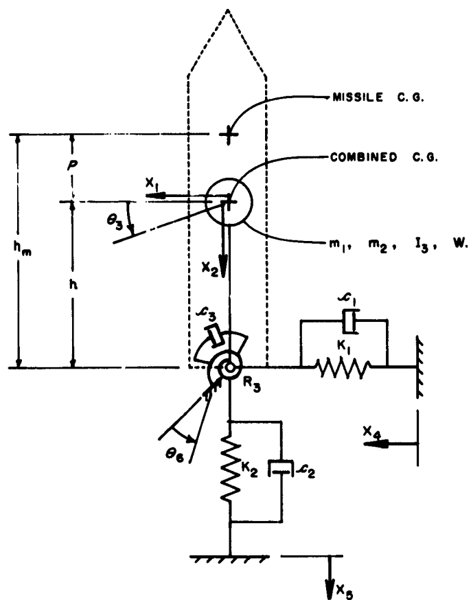
Fig. 18 - Dynamic model, hard condition
