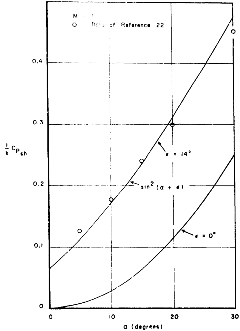
Figure 20. Induced Pressure Correlation of Blunt Leading Edges
