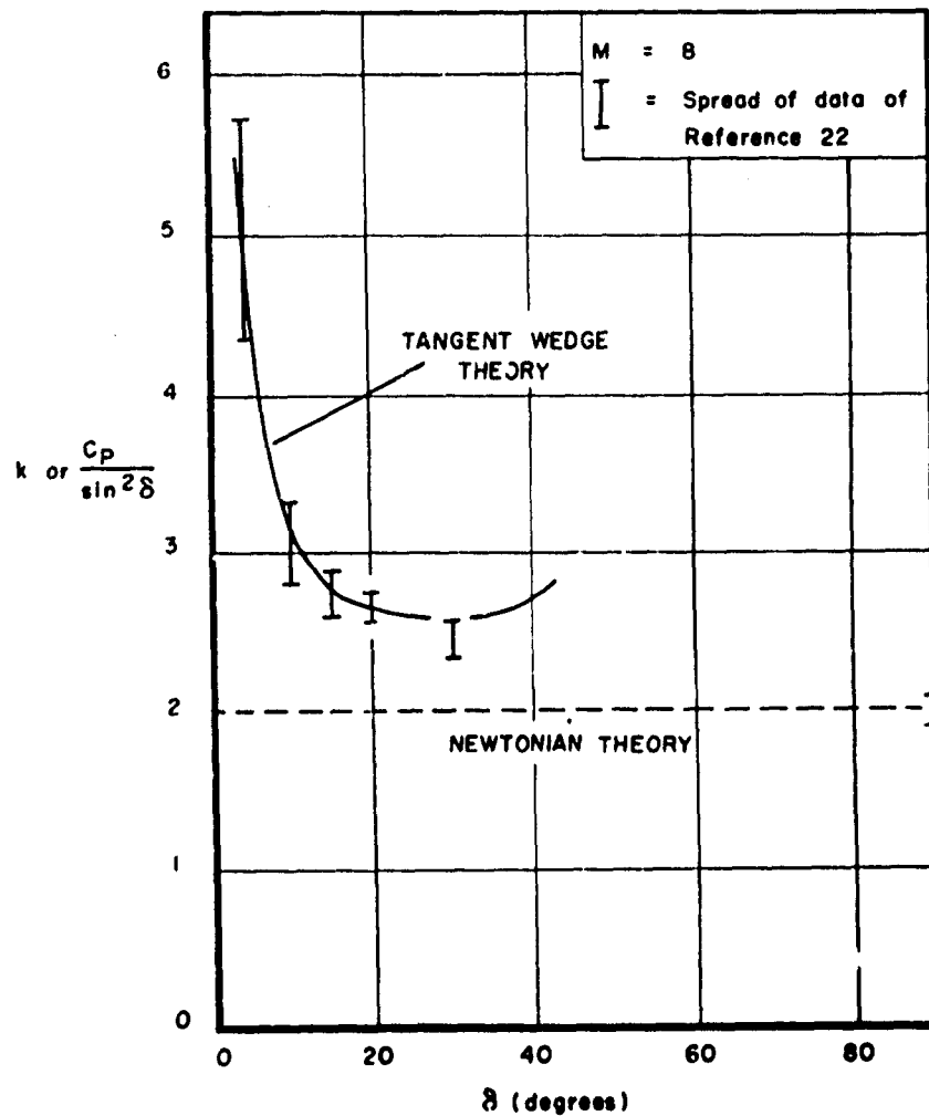
Figure 18. Lower-Surface Pressure Coefficients
