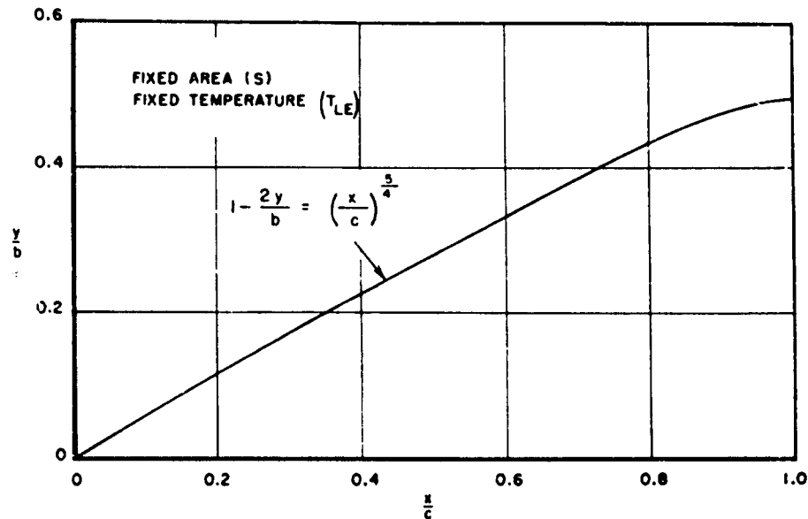
Figure 2. Geometry of Minimum Drag Planform
