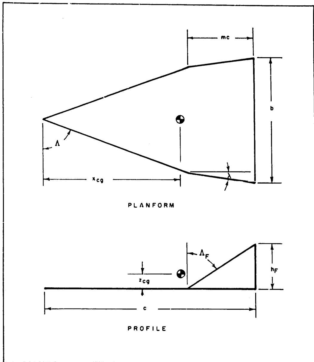
Figure 3. Geometry Model for Optimizing Taper Ratio
