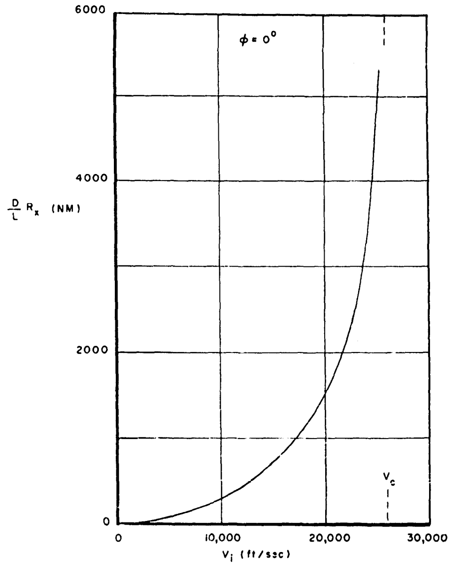
Figure 10. Longitudinal Range Versus Initial Velocity
