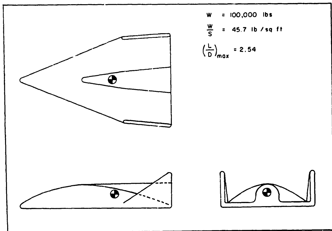
Figure 9. Typical Optimum Geometry
