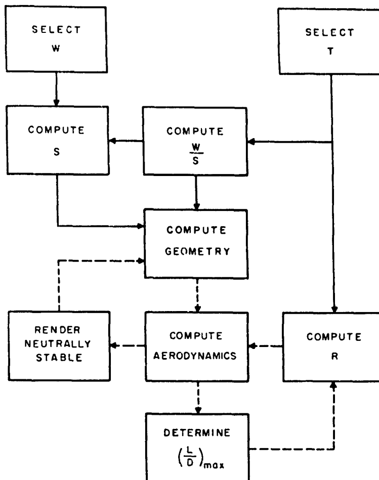
Figure 5. Block Diagram of Configurational Optimization Process
