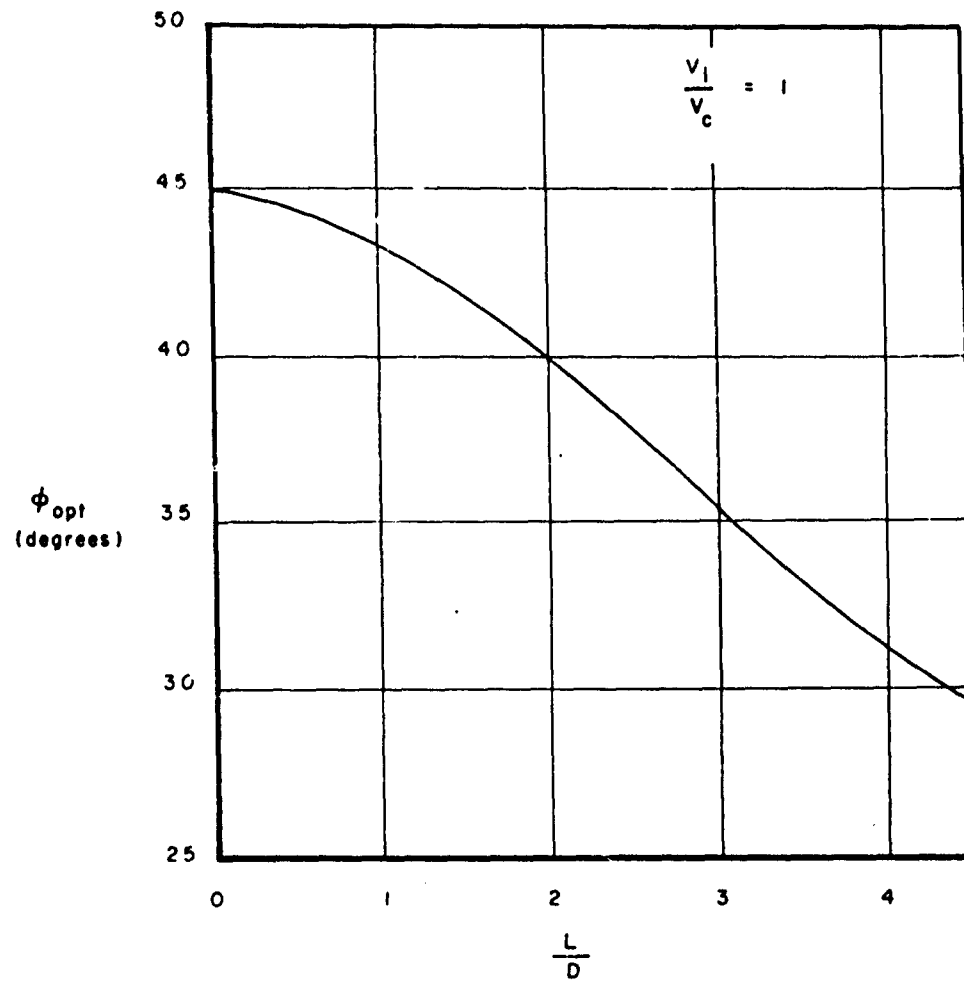
Figure 11. Optimum Bank Angle for Achieving Maximum Lateral Range
