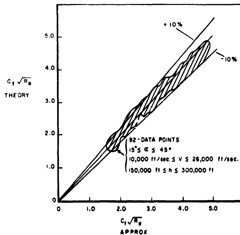
Figure 21. The Comparison of the Empirically Determined Laminar-Skin Friction Equations
