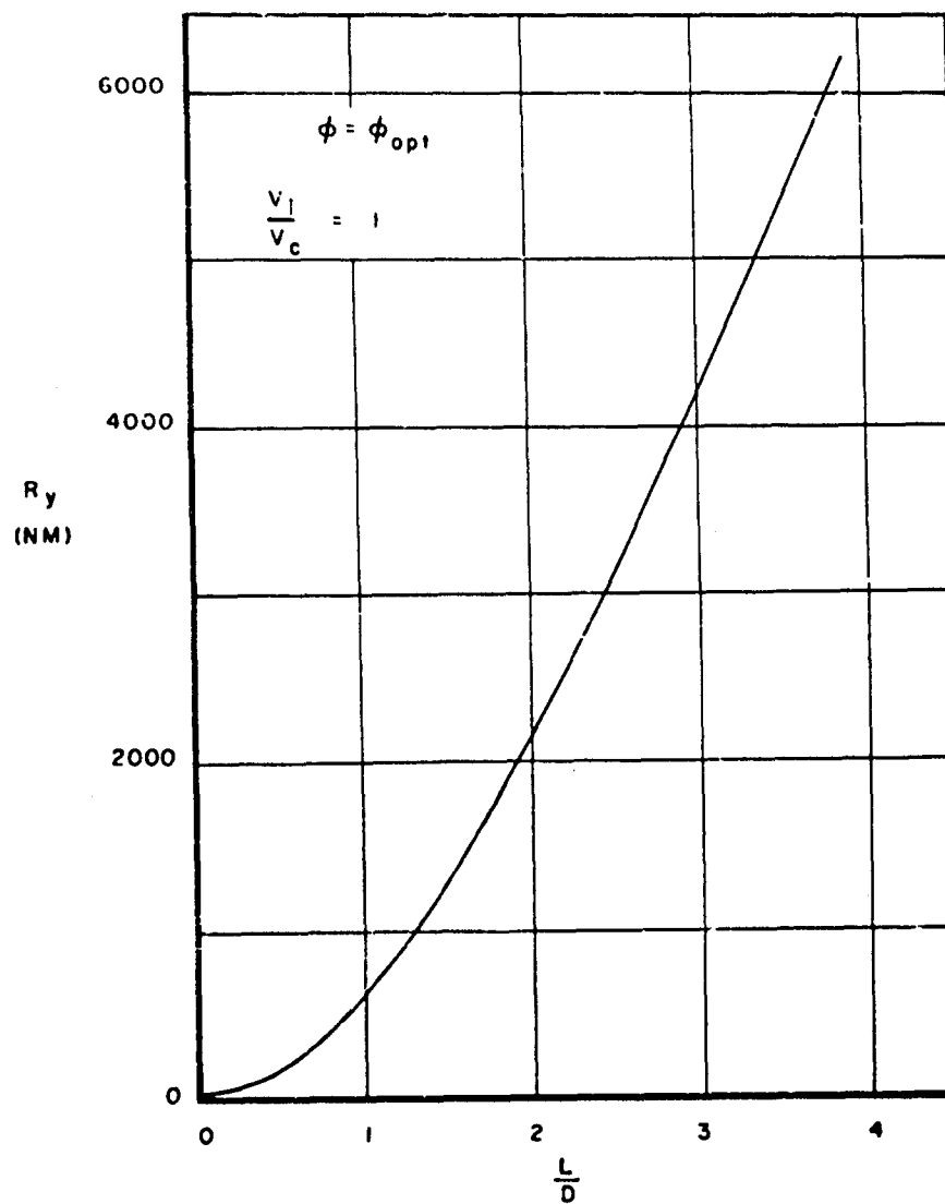
Figure 12. Maximum Lateral Range Versus L/D
