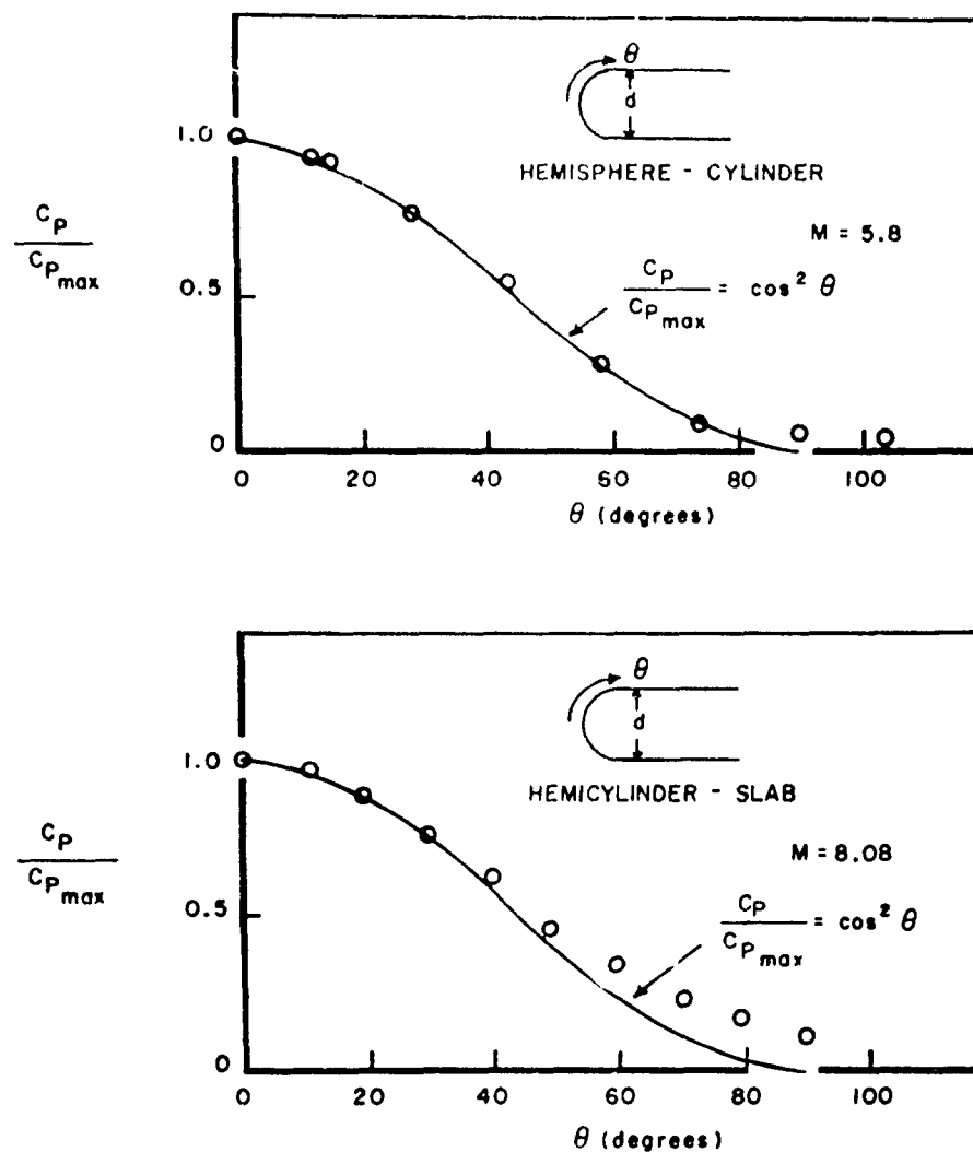
Figure 17. Applicability of Newtonian Theory to Hemispheres and Hemicylinders
