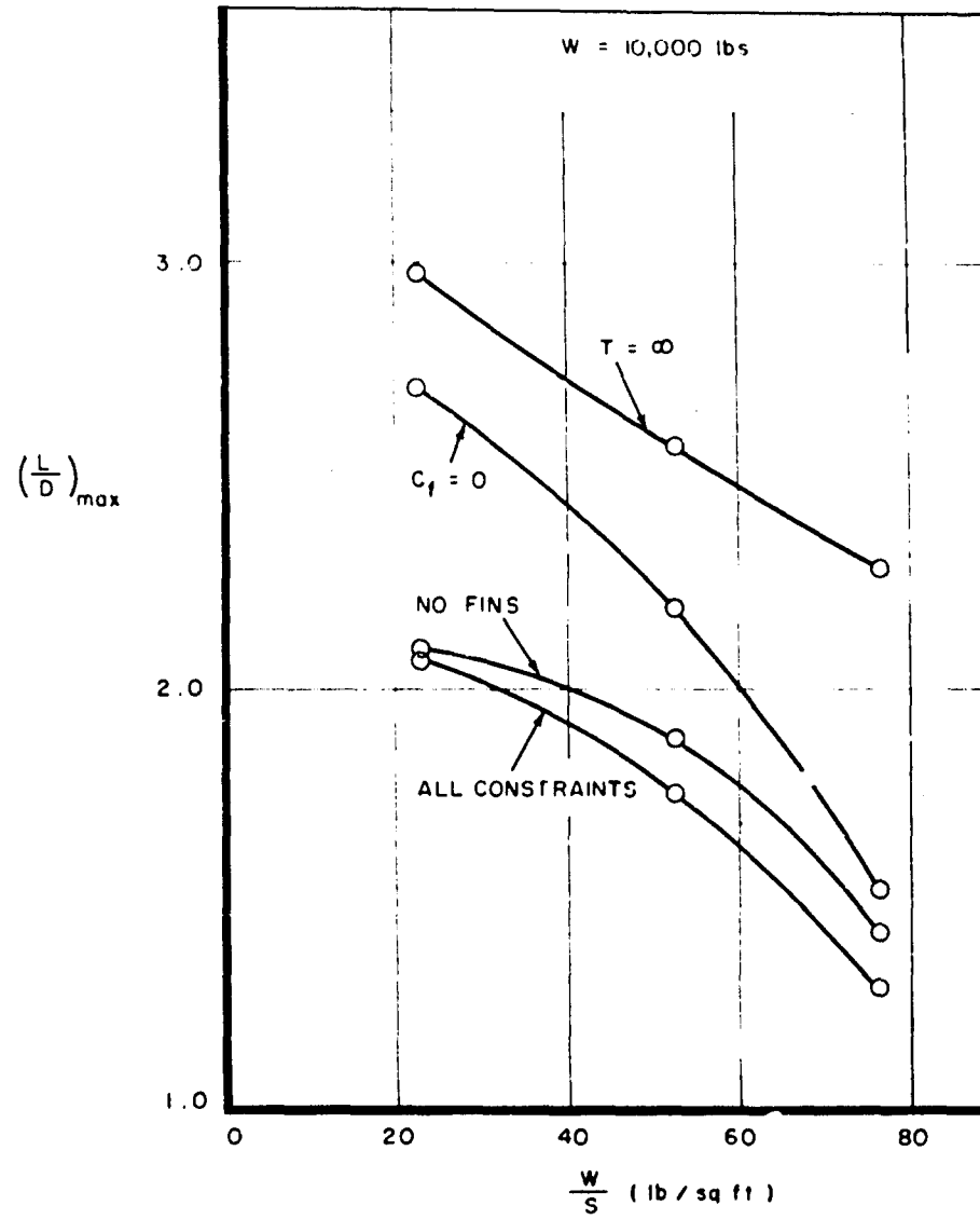
Figure 7. Constraint Influence on (L/D)_{\max} ; W = 10,000 Pounds
