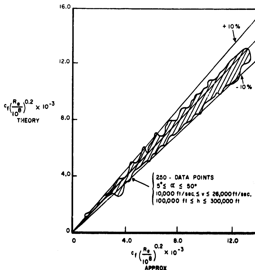
Figure 22. The Comparison of the Empirically Determined Turbulent-Skin Friction Equations
