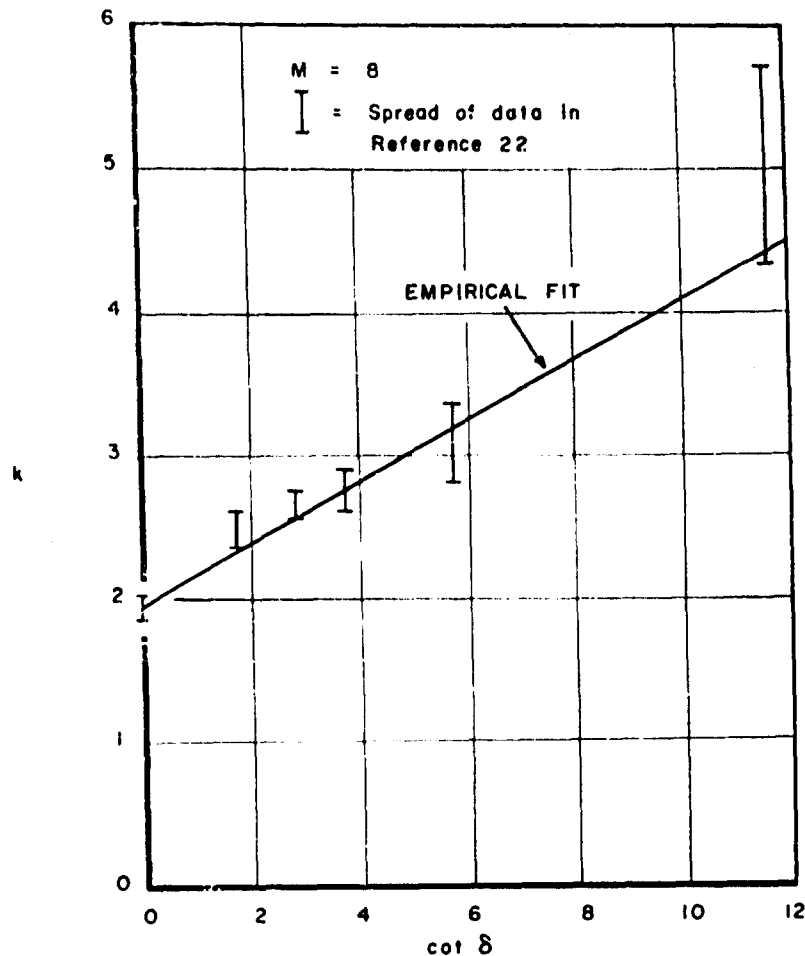
Figure 19. Empirical Correlation of Lower-Surface Pressure Coefficients
