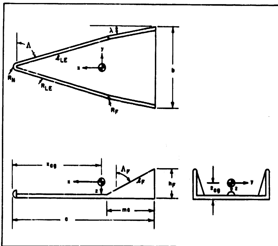
Figure 23. The Generalized Configuration Geometry
