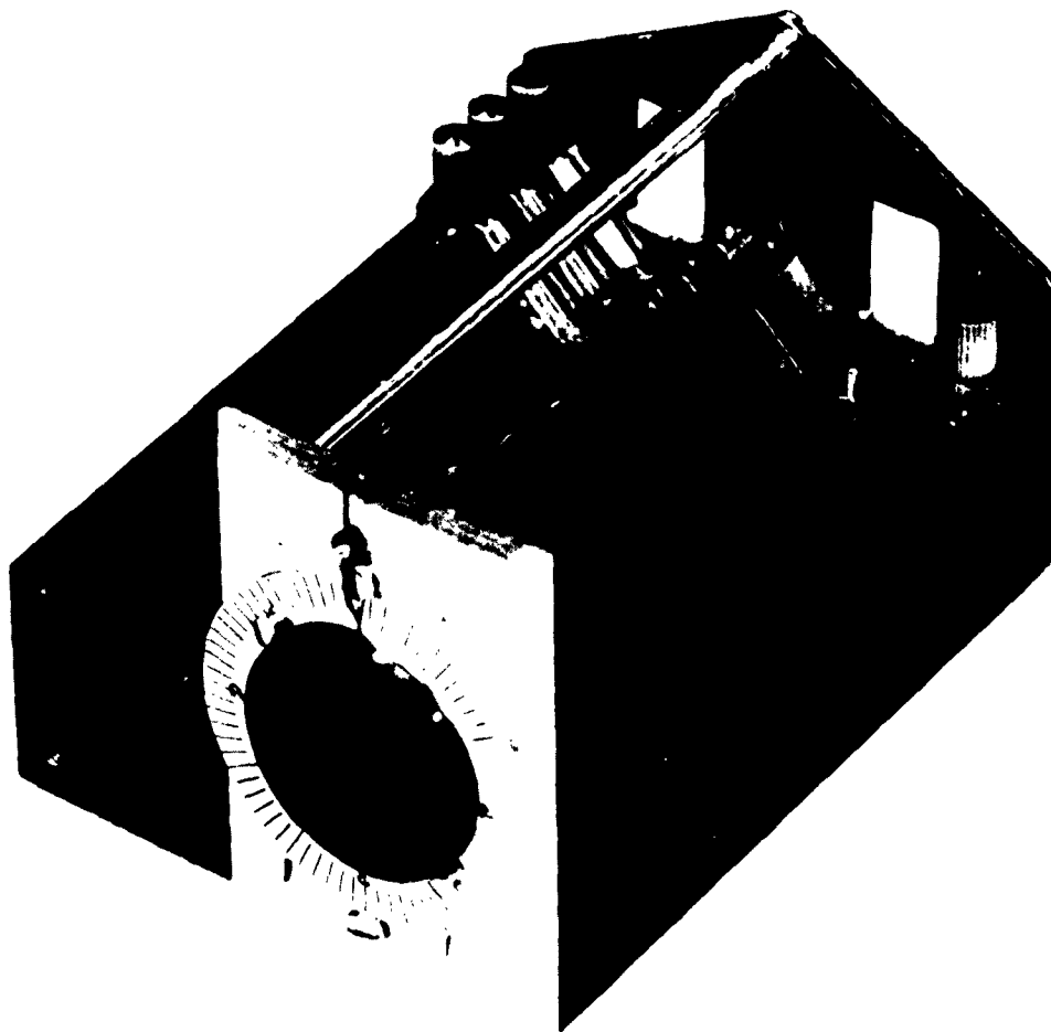
FIG. 6. Specimen Holder Mounted for Use in the Cary Model 14 Spectrophotometer.
