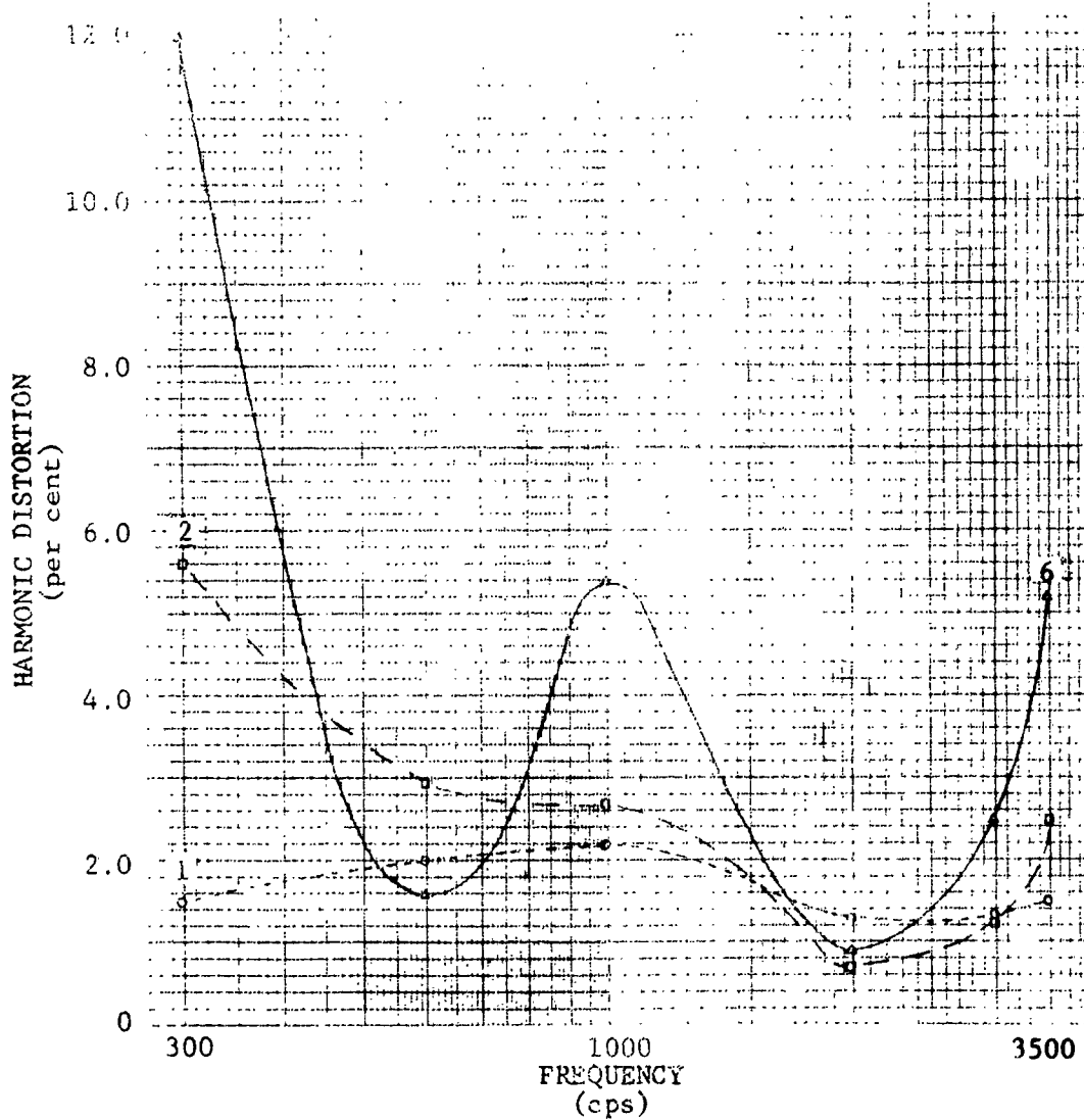
FIGURE B-183 SYSTEM HARMONIC DISTORTION Wire Carrier System Configurations 1, 2 and 4 Input Level -4 dbm
