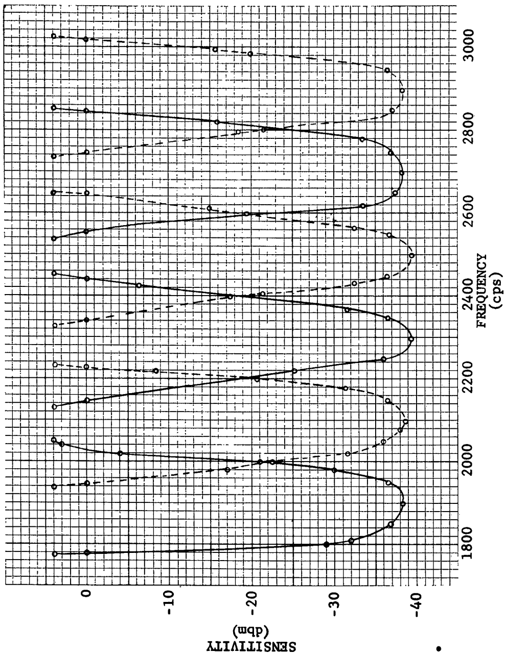
FIGURE B-22 RELEASE AND RECALL MONITOR SELECTIVITY CURVES AN/ITC-12 SN 3 Monitor Tested - Group 1
