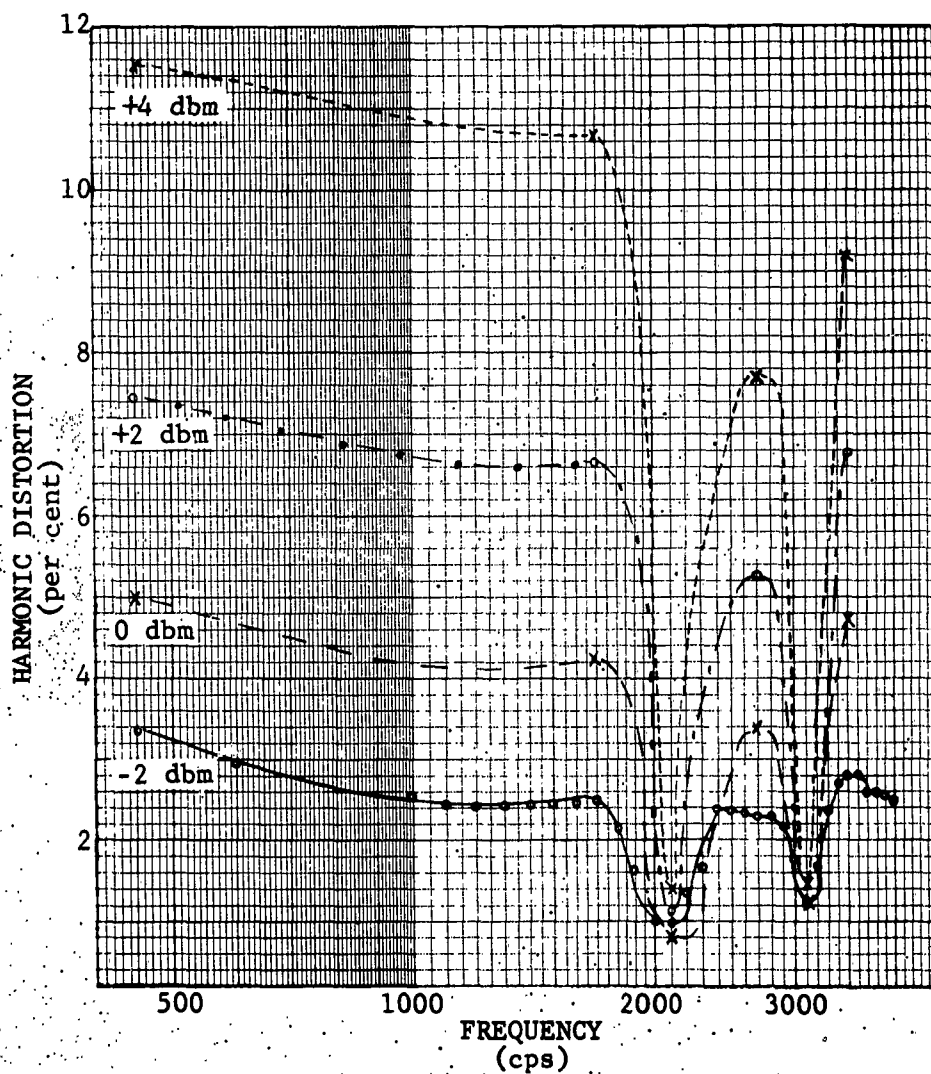
FIGURE B-7 EFFECT OF LIMITING ON HARMONIC DISTORTION - AN/TTC-12 SN 1 Lines Tested 1
