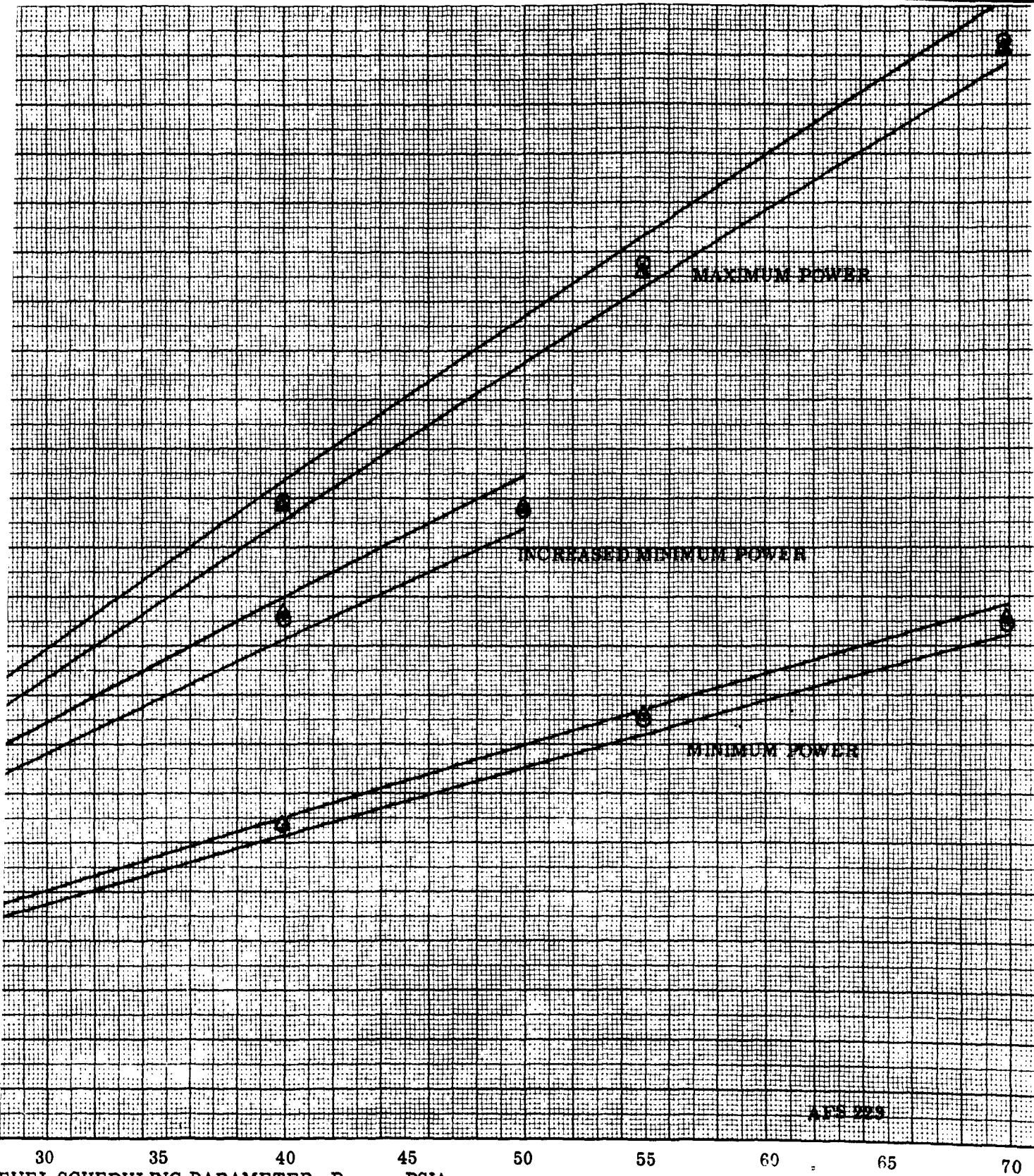
FUEL SCHEDULING PARAMETER, P_{t1.4} \sim \text{PSIA} Power Control System Calibration Data Before and After the RJ43-MA-11 Phase I Long-Term Storage Test.
