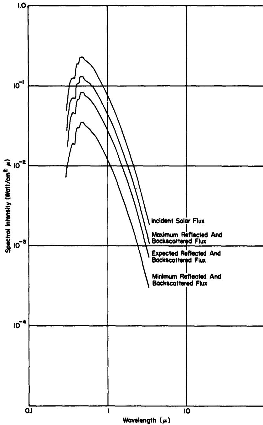
Fig. 2 Reflected and Backscattered Flux Compared to Incident Solar Flux over the 0.3 - 3.2 \mu Spectral Region
