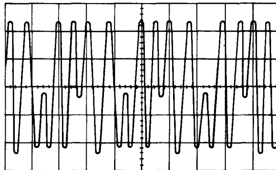
D. TP5 (OUTPUT Q9) PHASE SHIFTED CARRIER MODULATED WITH 1200 BPS SQUARE WAVE 0.11 V P/P TP1 (OUTPUT Q11) PHASE SHIFTED CARRIER 22VP/P TP2 (OUTPUT Q12) PHASE SHIFTED CARRIER 2.2VP/P
