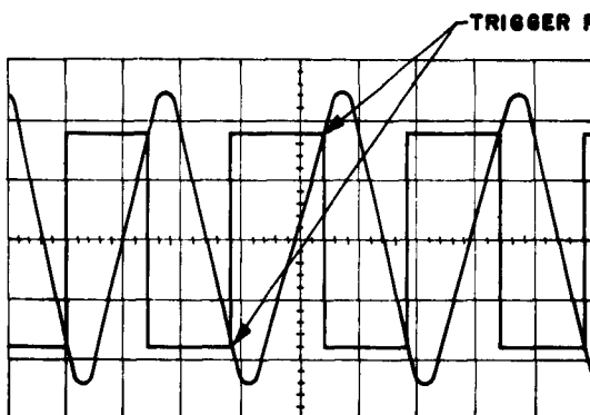
J. TP7 & TP9 - RELATIONSHIP OF LOW PASS VERSUS SCHMITT TRIGGER OUTPUT
