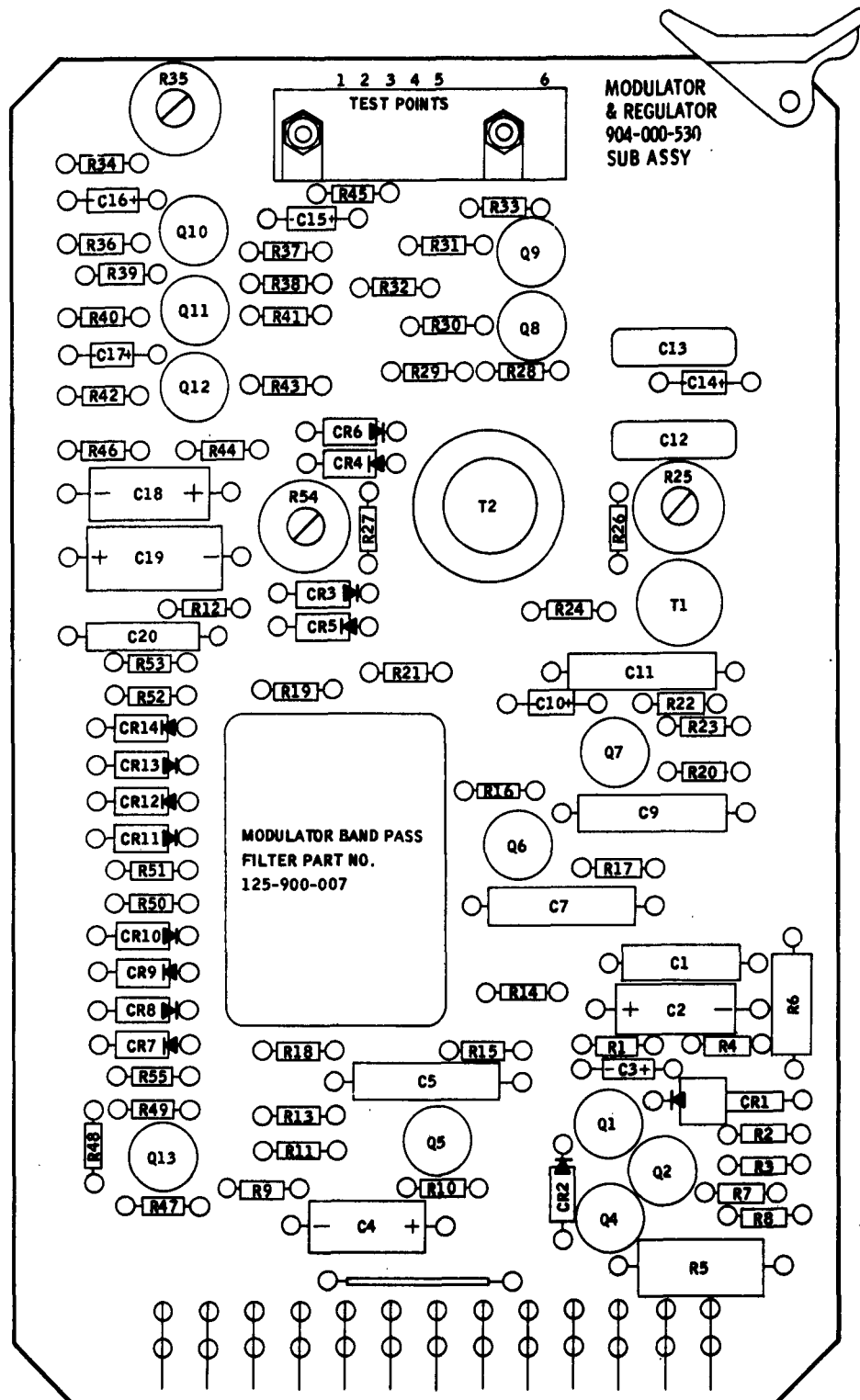
Figure 5-3. Modulator and Regulator Component Layout
