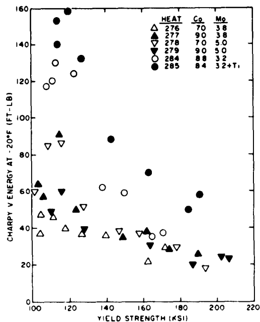
Fig. 3 - Charpy V impact energy at -20°F vs yield strength for the six compositions which responded to aging
