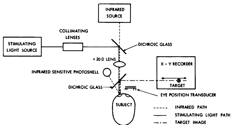
Fig. XVII-5. Experimental arrangement.
