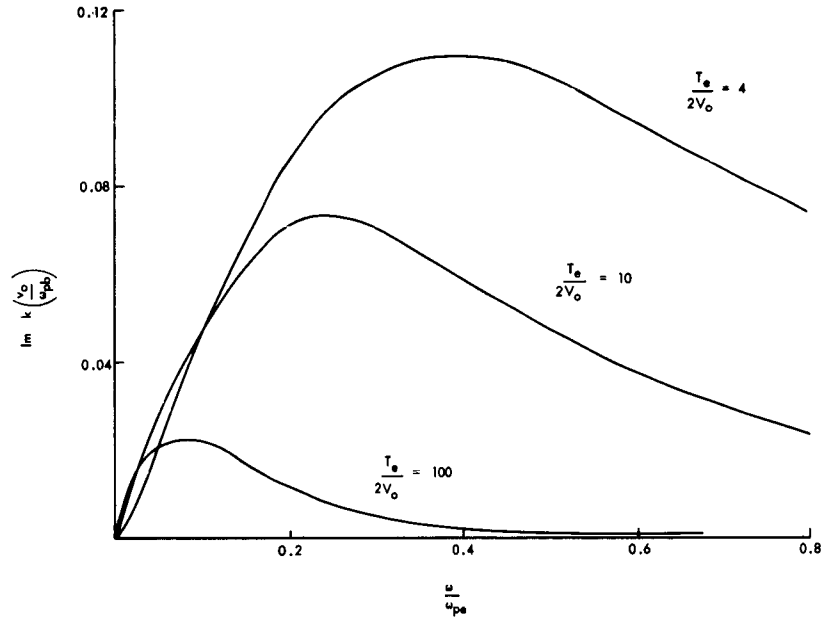
Fig. VII-13. Resistive-medium amplification.
