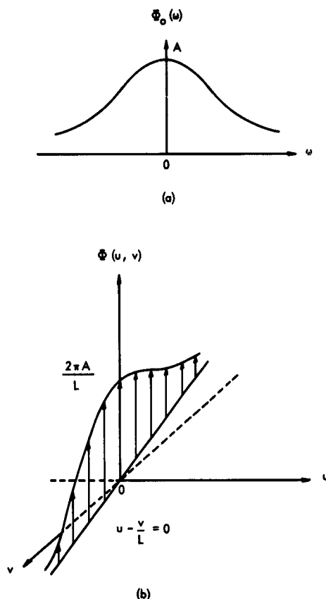
Fig. X-2. Relation between \Phi(u, v) and \Phi_o(\omega) .
