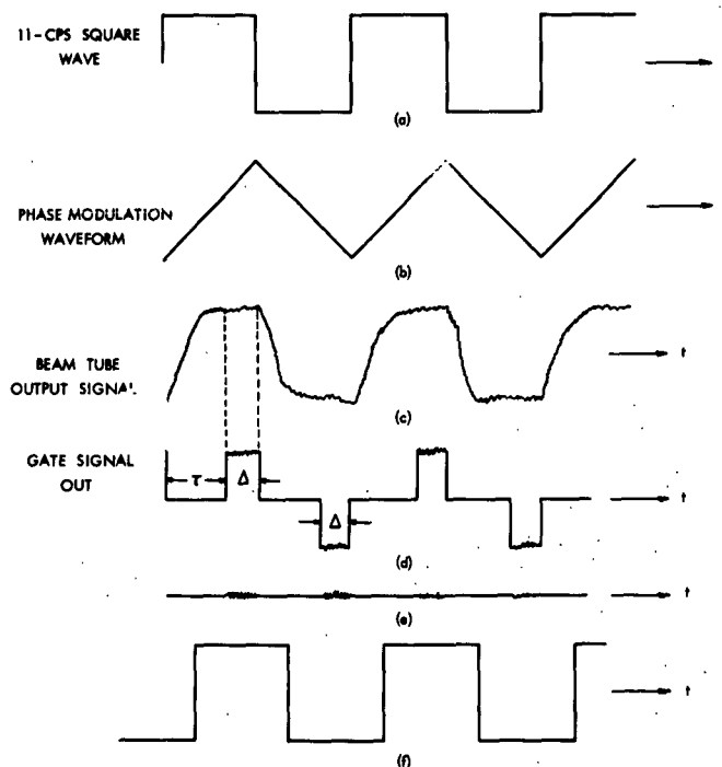
Fig. III-1. Waveforms present in the cesium clock system.
