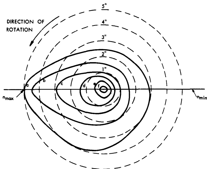
Fig. VII-5. Density Contour Map. Density in particles per \text{cm}^3 : a, 10^{10} ; b, 2 \times 10^{10} ; c, 4 \times 10^{10} ; d, 8 \times 10^{10} ; e, 1.8 \times 10^{11} ; f, 2.5 \times 10^{11} . Magnetic field into the page.
