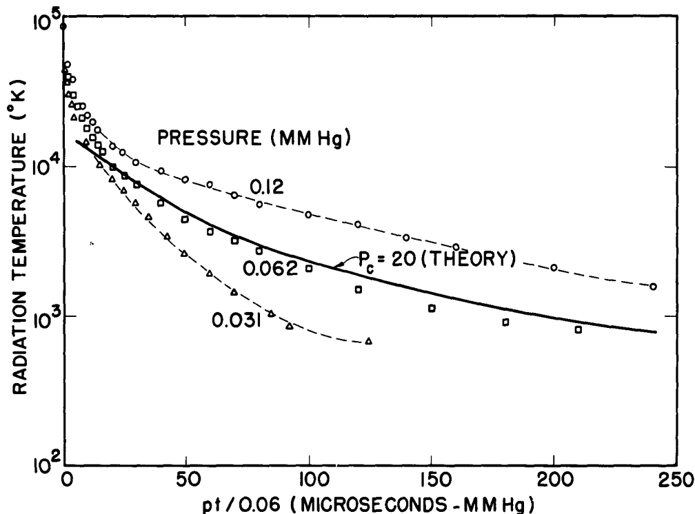
Fig. VI-2. Electron temperature decay for low pressures.
