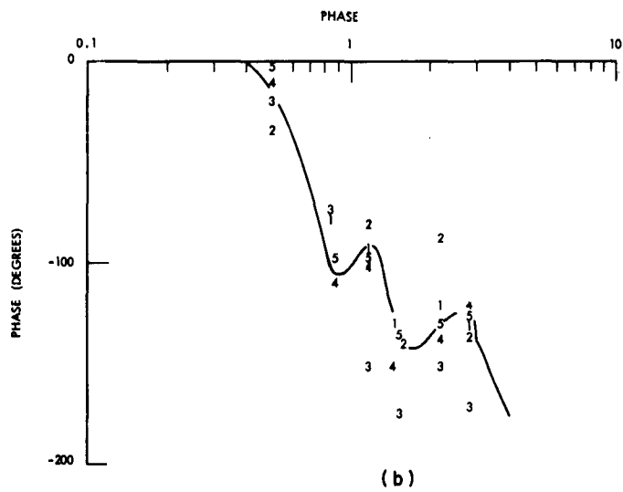
Fig. XVII-8. Bode plot of eye-tracking movement control system.
