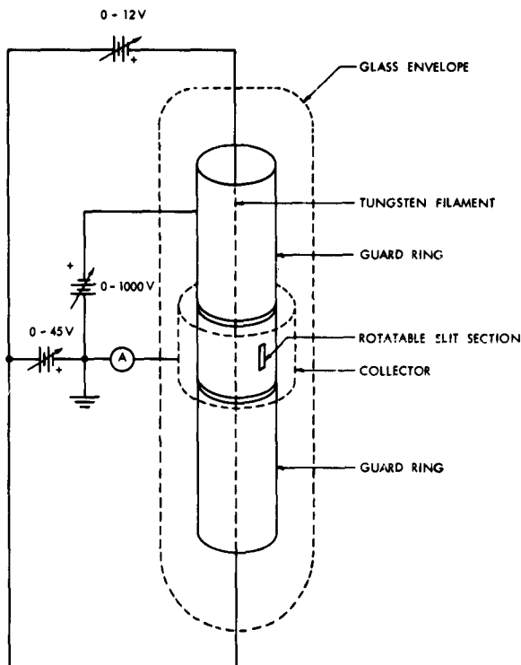
Fig. VIII-1. Experimental apparatus.
