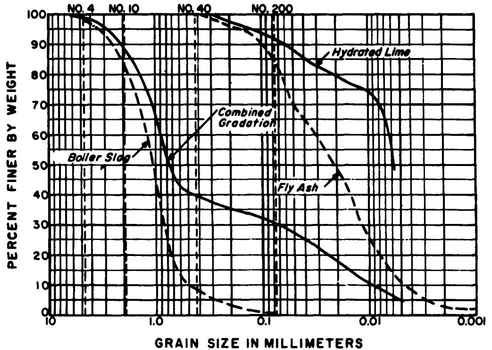
Figure 1. Grain size distribution of combined mixture and components.
