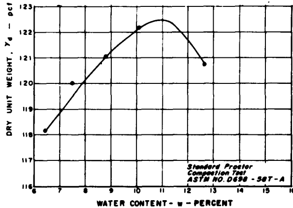
Figure 2. Relationship between dry unit weight and molding water content.
