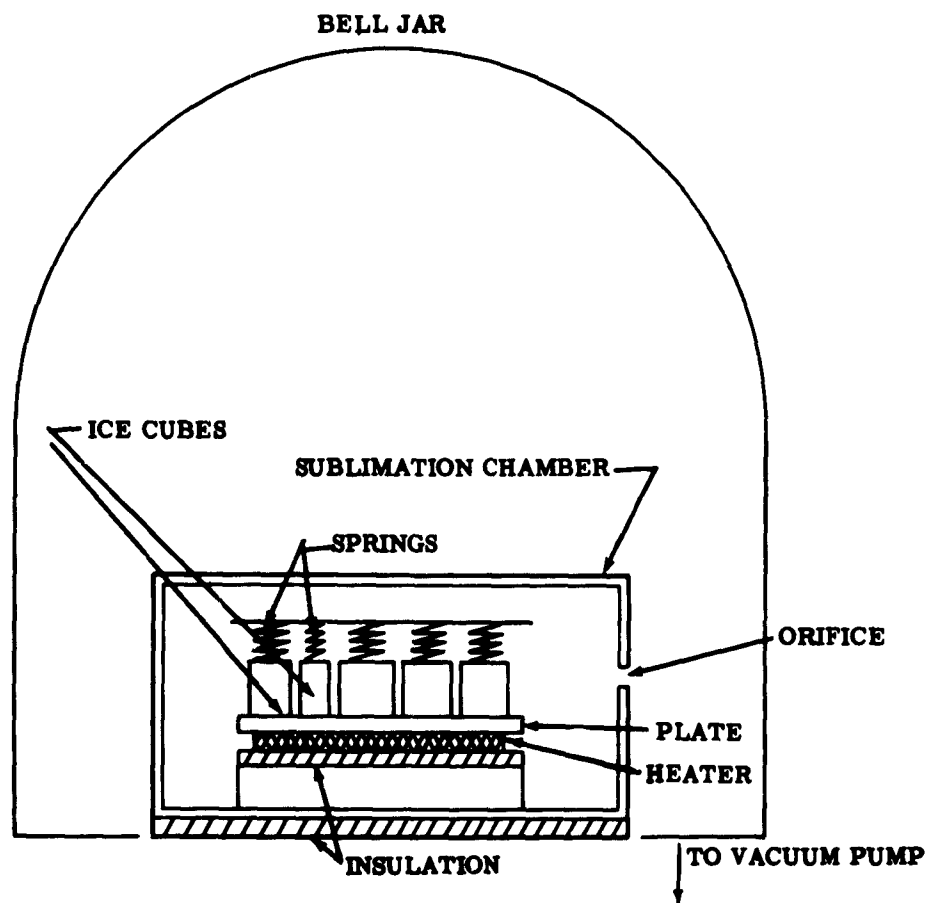
TEST SETUP FOR ICE SUBLIMATION SYSTEM
