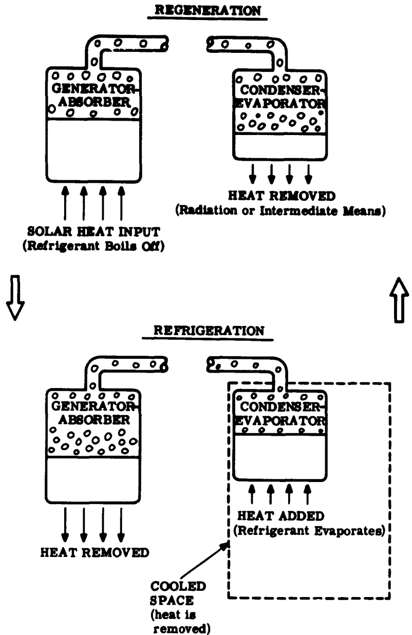
INTERMITTENT ABSORPTION COOLER WITH SOLAR REGENERATION (ALTERNATING CYCLES)
