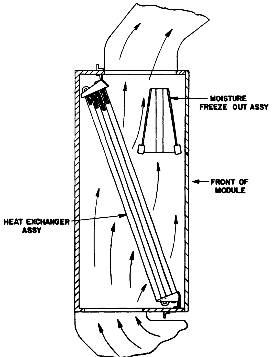
FIGURE 13 HEAT EXCHANGER & FREEZE OUT INSTALLATION ATTITUDES
