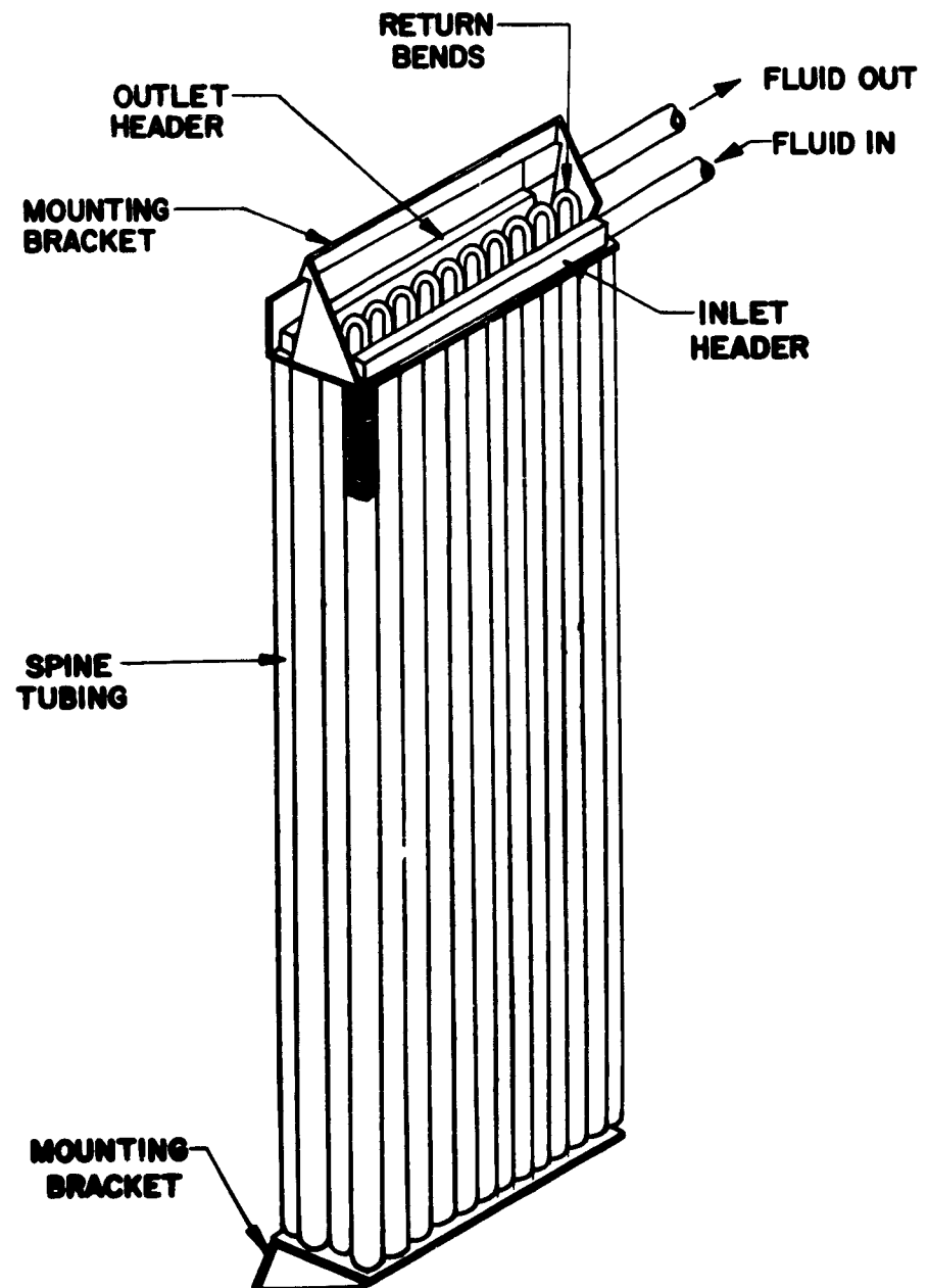
FIGURE II HEAT EXCHANGER
