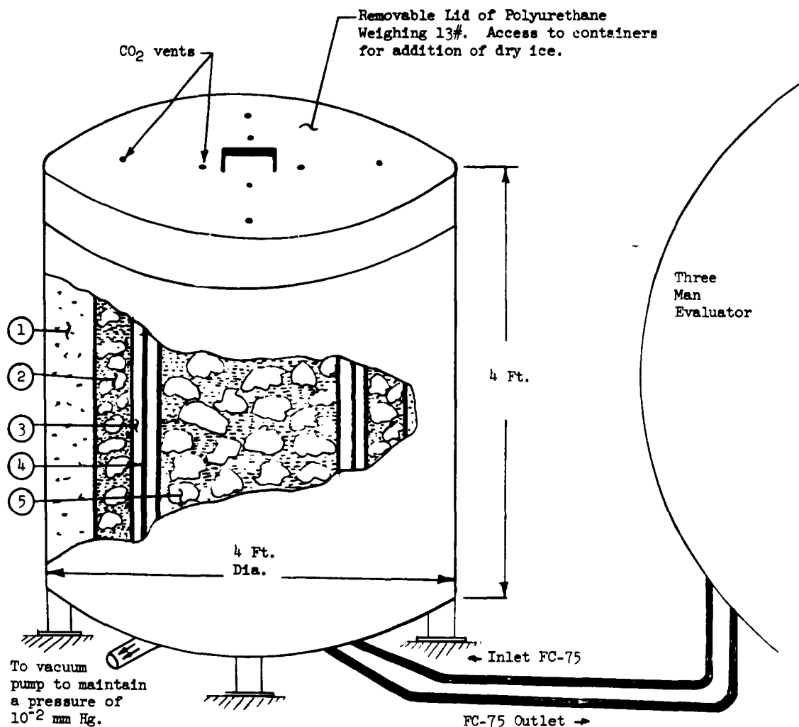
FIGURE 18 LOW TEMPERATURE HEAT SINK
