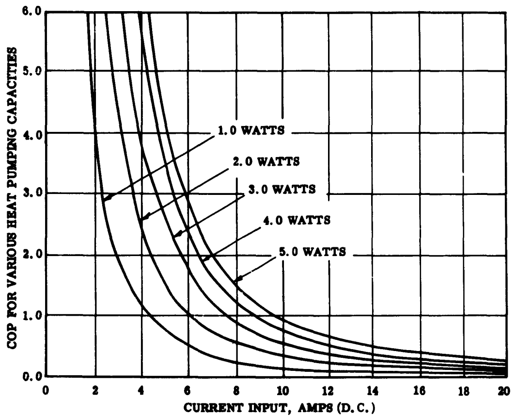
TYPICAL THERMAL AND ELECTRICAL CHARACTERISTICS OF COMMERCIALY AVAILABLE THERMO-ELECTRIC COUPLES COP VS CURRENT
