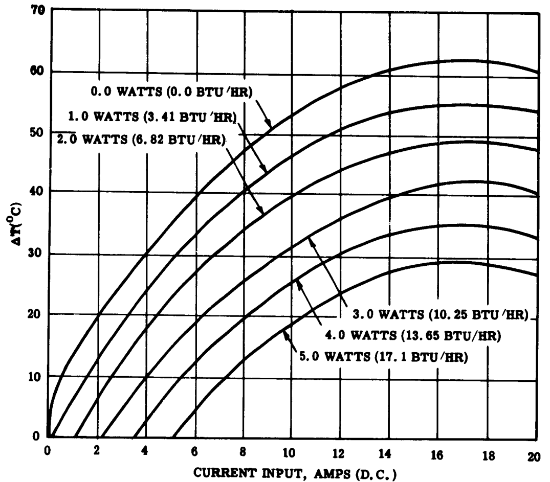
TYPICAL THERMAL AND ELECTRICAL CHARACTERISTICS OF COMMERCIALLY AVAILABLE THERMO-ELECTRIC COUPLES \Delta T VS CURRENT
