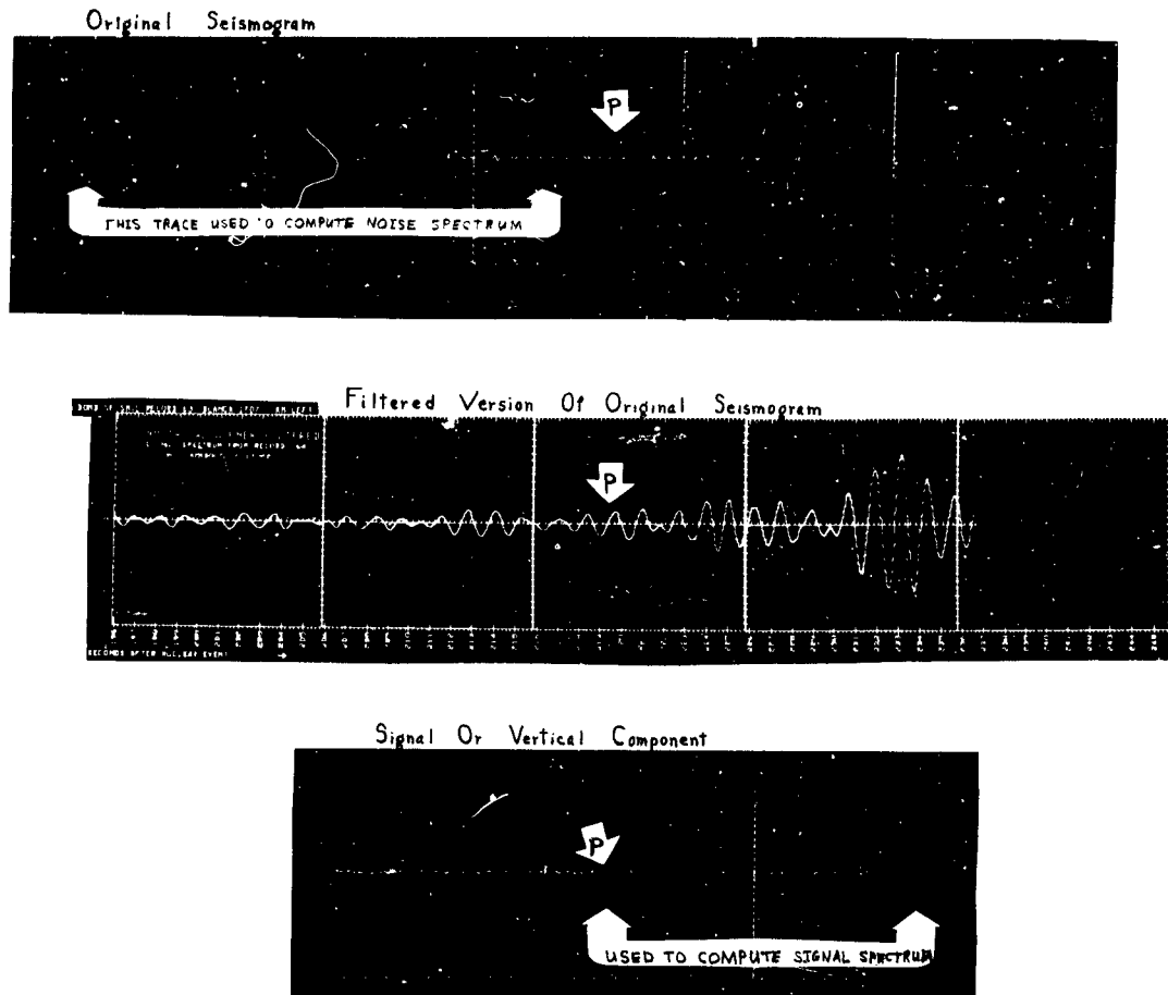
Figure II-2 Example Of Wiener Filtering Noise spectra is taken from before the p-wave on the left component (top) and signal spectra is taken from the higher quality vertical component (bottom). These spectra are used to generate a filter which is used on the original seismogram (top) to produce a filtered version (middle). Considerable signal-to-noise ratio improvement is noted, but the first motion is not any more apparent. The exact time of first motion is known from the vertical.
