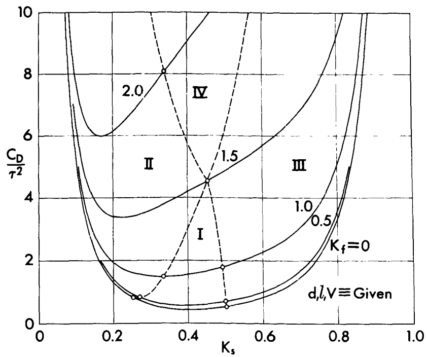
Fig. 15. Drag coefficient for given diameter, length, and volume.
