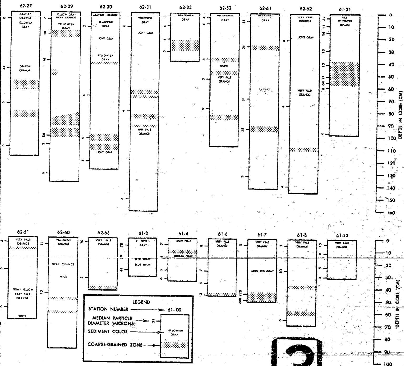
LONGITUDINAL CROSS SECTION OF AXIAL CORES
