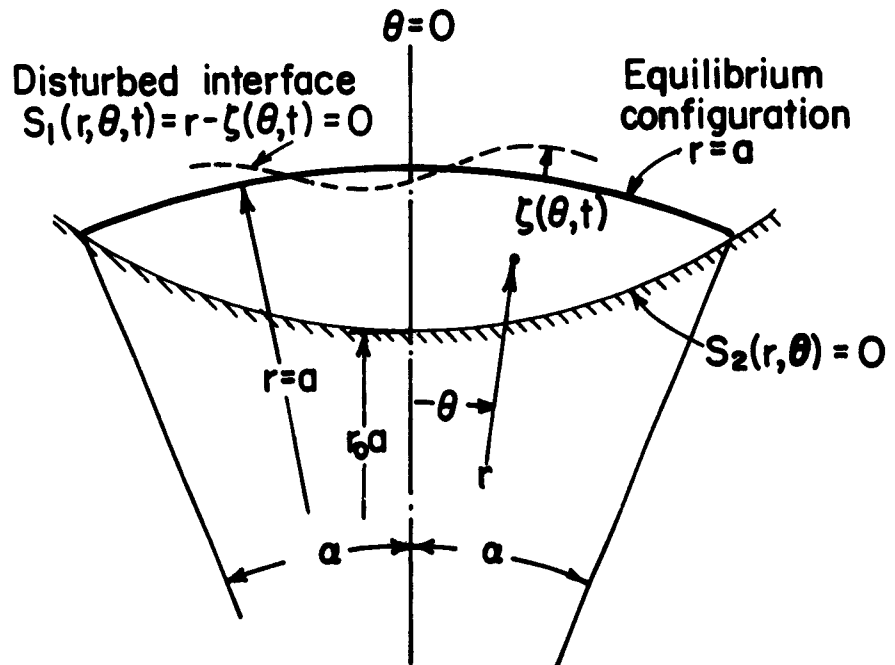
Fig. 9. Reference Frame for Two-Dimensional Layer with Curved Interface.
