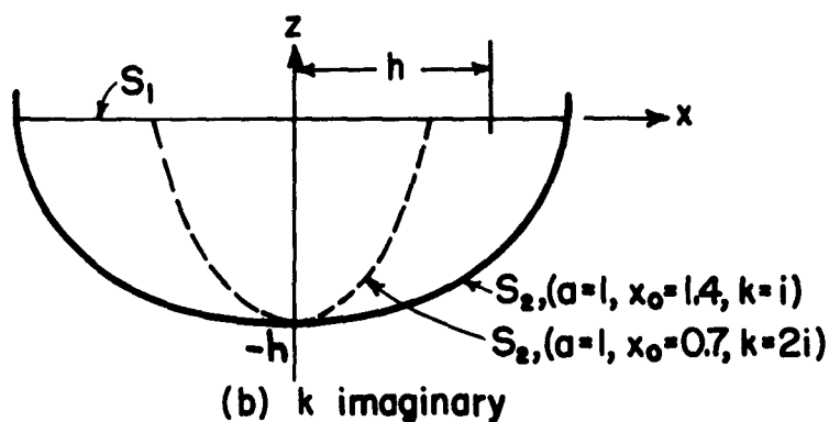
Fig. 3 Two-Dimensional Layers with Free Oscillations Defined by \Phi(x, z, t) = D \sinh(kx) [\cos k(a+z) - \cos(kz) \cosh(kx_0)] e^{i\sqrt{\sigma}t} ; (a) k real, (b) k imaginary.
