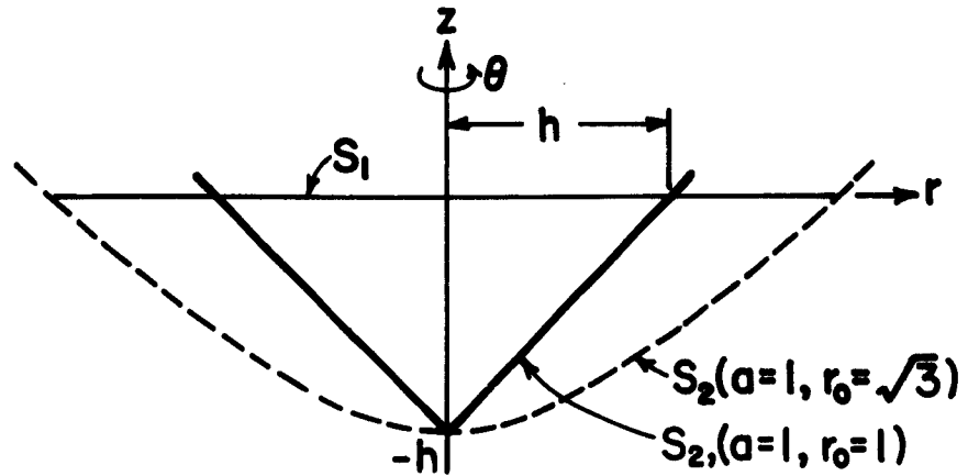
Fig. 8 Three-Dimensional Layers with Free Oscillations Defined by \Phi(r, z, \theta, t) = Ar[z + (a^2 + r_0^2)/2a]e^{i(\theta + \sqrt{\sigma}t)}
