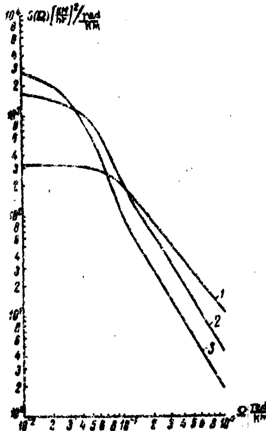
Fig. 4. Curves of spectral density: 1 -- in Cs clouds with \sigma^2 , 2 -- in Cs clouds with \sigma^2 , 3 -- outside clouds with \sigma^2 .
