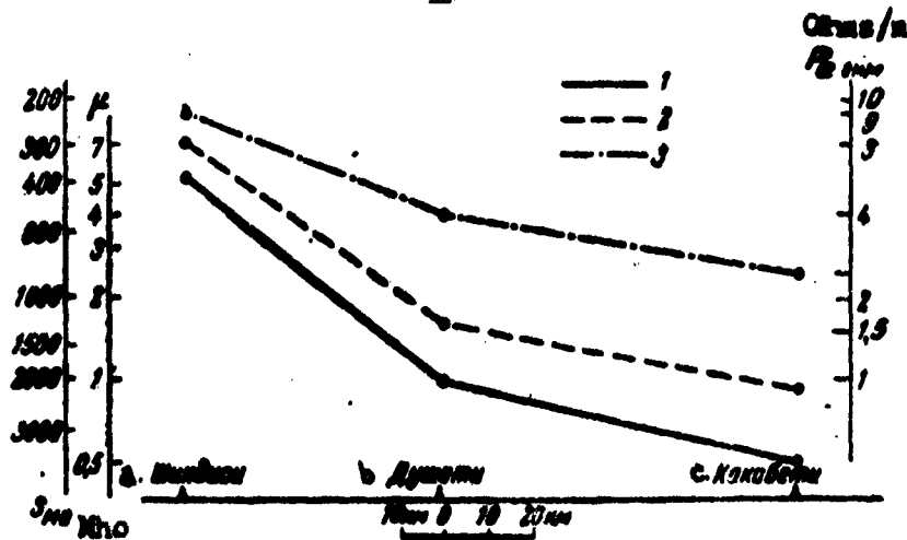
Fig. 2. Comparison of the results of magnetotelluric sounding and the data for a long-period telluric survey along the profile Shindisi-Dusheti-Kakabeti: 1 -- curve for the telluric parameter \mu , 2 -- curve of \sigma = total linear conductivity based on magnetotelluric sounding data, 3 -- curve of the mean linear resistivity based on magnetotelluric sounding data. a -- Shindisi, b -- Dusheti, c -- Kakabeti.
