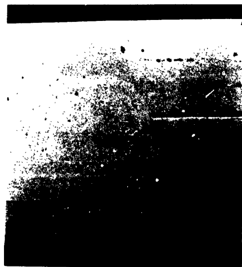
Figure 20. Photomicrograph (100X) of the right side of Section A-A of the as-polished spot weld shown in Figure 18. The section also contains the foil-to-nugget line of demarcation. This section represents the area on the radiograph which does not contain the dark peripheral line image.
