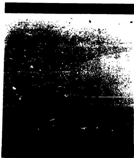
Figure 19. Photomicrograph (100X) of the left side of Section A-A of the as-polished spot weld shown in Figure 18. Note the line of demarcation between the nickel foil and the weld nugget. This section represents the area on radiograph which contains the dark peripheral line image. No cracks are present in this spot weld.
