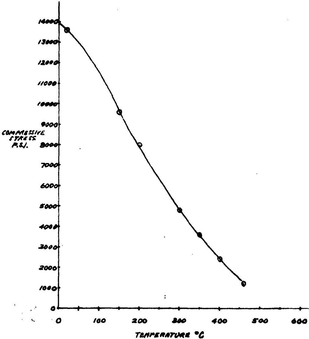
TYPICAL COMPRESSIVE YIELD STRESS. (SHORT TIME) LEAD TELLURIDE COLD PRESSED AND HEAT TREATED
