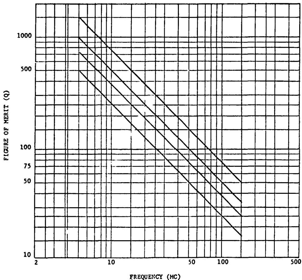
Figure VIII-4. Typical Figure of Merit (Q) Versus Frequency Characteristics at 25°C
