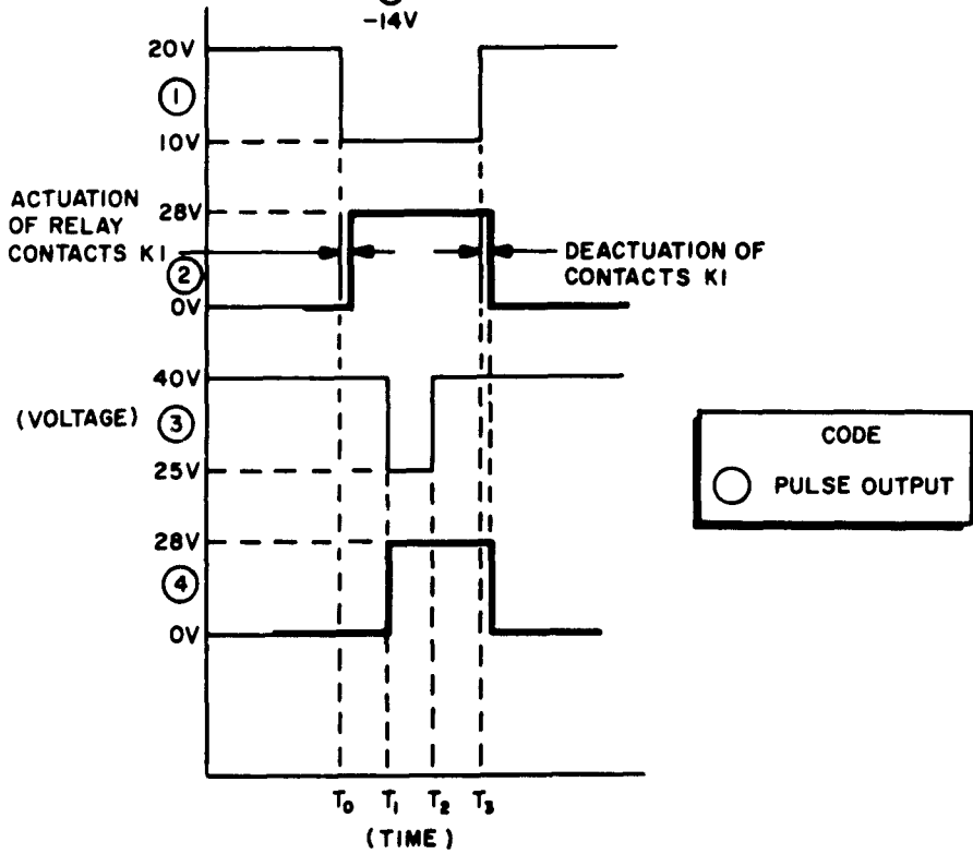
Figure 2. Circuitry Used to Switch Relay Box
