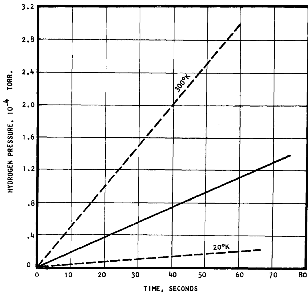
Figure 10 - Hydrogen Pressure During Condensation of \text{CH}_4 Containing 0.15% Hydrogen. Condensation Rate = 1.11 \times 10^{17} \text{cm}^{-2} \text{sec}^{-1} . The Dotted Lines are Calculated Pressures Assuming No Trapping.
