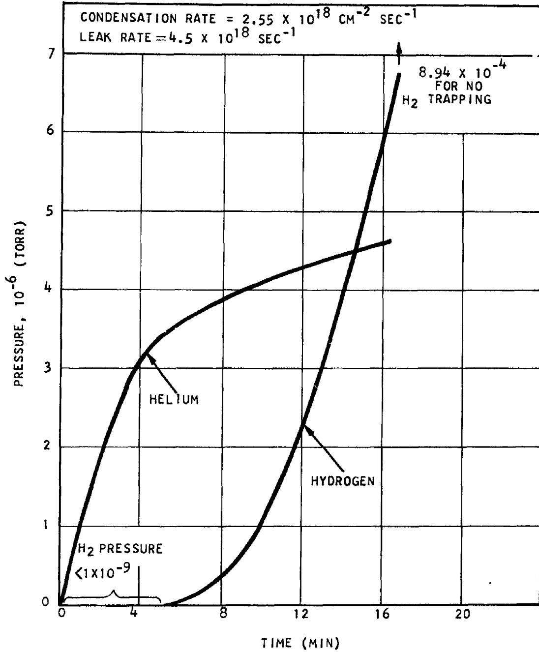
FIG. 14 HELIUM AND HYDROGEN PRESSURES DURING CONDENSATION OF OXYGEN CONTAINING 10.8 PPM H 2
