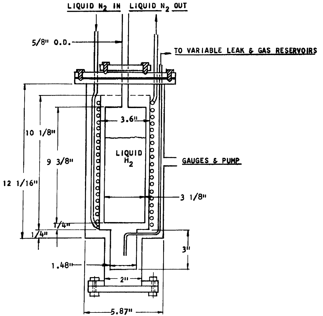
Figure 1 - Cryopump Diagram
