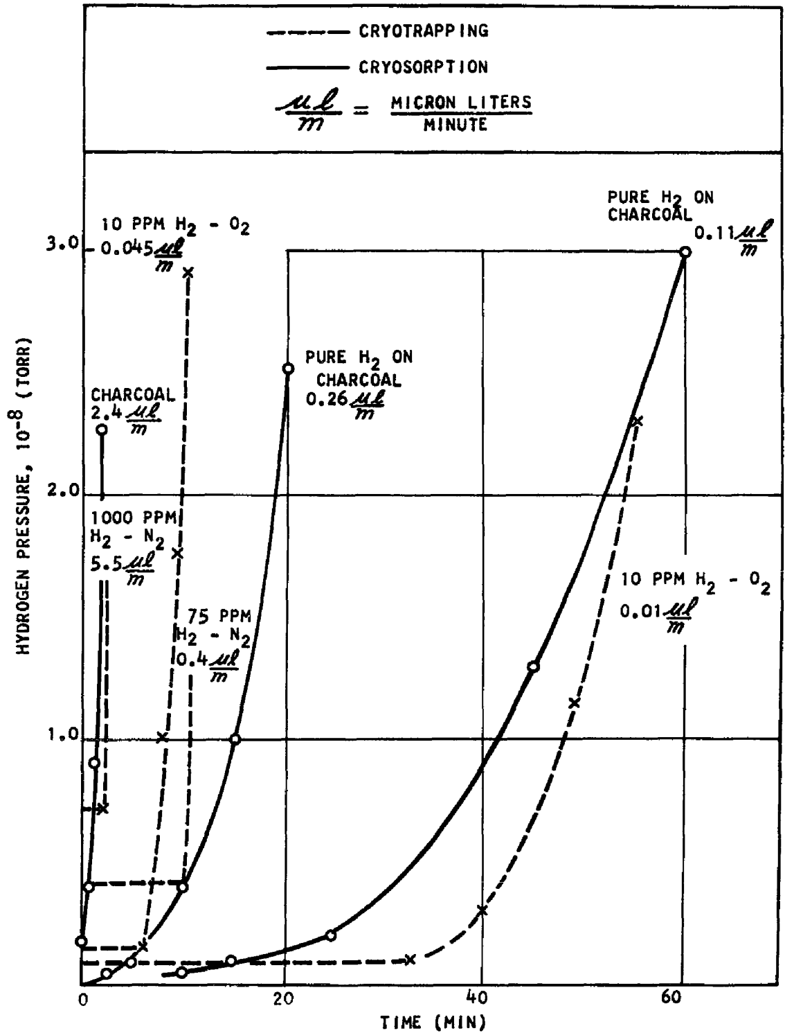
FIG. 21 COMPARISON OF HYDROGEN PRESSURE CURVES DURING CRYOTRAPPING AND CHARCOAL CRYOSORPTION
