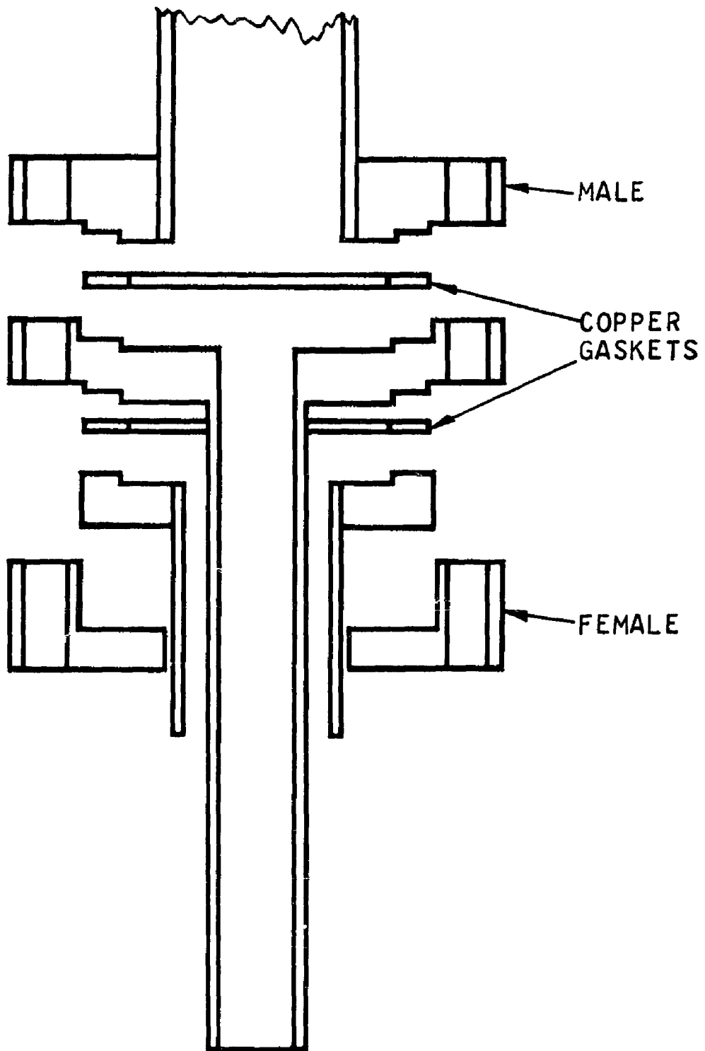
FIG. 2 HERMAPHRODITE FLANGE
