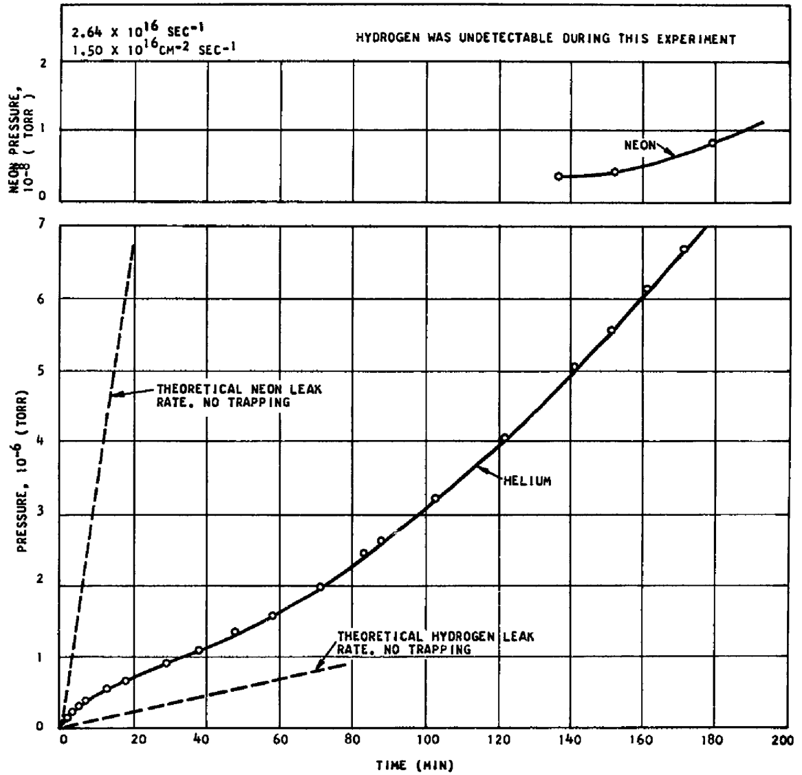
FIG. 24 NEON AND HELIUM PRESSURES DURING CRYOPUMPING OF AIR AT 20°K
