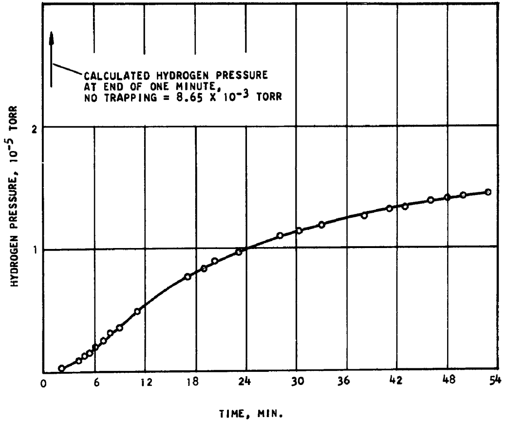
Figure 13 - Hydrogen Pressure During Condensation of \text{CHClF}_2 Containing 1.4% Hydrogen. Condensation Rate = 3.3 \times 10^{16} \text{cm}^{-2} \text{sec}^{-1} .
