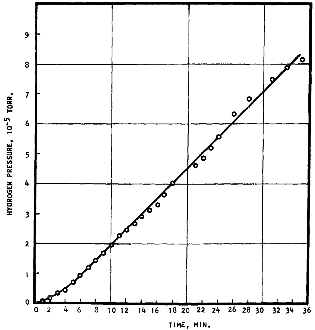
Figure 9 - Hydrogen Pressure During Condensation of \text{CF}_4 Containing 0.17% Hydrogen. Condensation Rate = 6.5 \times 10^{16} \text{cm}^{-2} \text{sec}^{-1} . Assuming No Trapping, Pressures at the End of the Experiment were Calculated to be 7.5 \times 10^{-3} Torr. ( 300^\circ\text{K} ) or 5.03 \times 10^{-4} Torr. ( 20^\circ\text{K} ).
