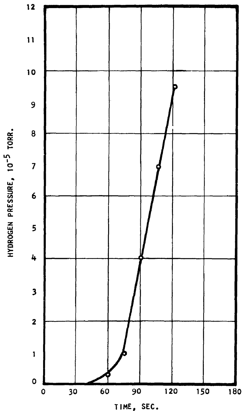
Figure 8 - Hydrogen Pressure During Condensation of \text{CF}_4 Containing 0.17% Hydrogen. Condensation Rate = 9.26 \times 10^{17} \text{cm}^{-2} \text{sec}^{-1} . Assuming No Trapping, Pressures at the End of the Experiment were Calculated to be 1.01 \times 10^{-2} Torr. ( 300^\circ\text{K} ) or 6.71 \times 10^{-4} Torr. ( 20^\circ\text{K} ).
