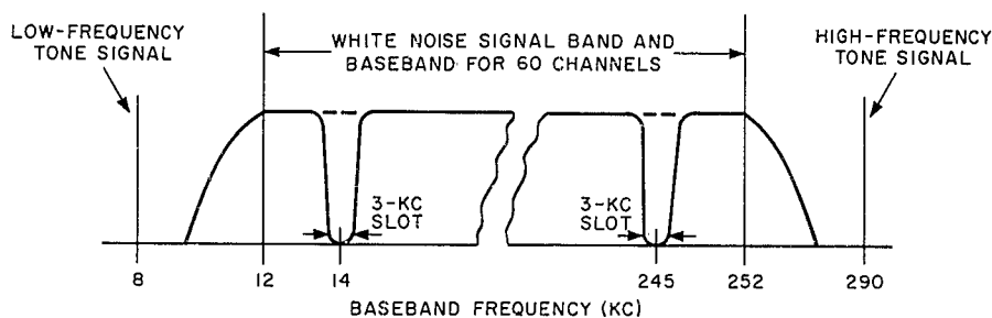
Figure 4. Test Signal for Modulating Carrier
