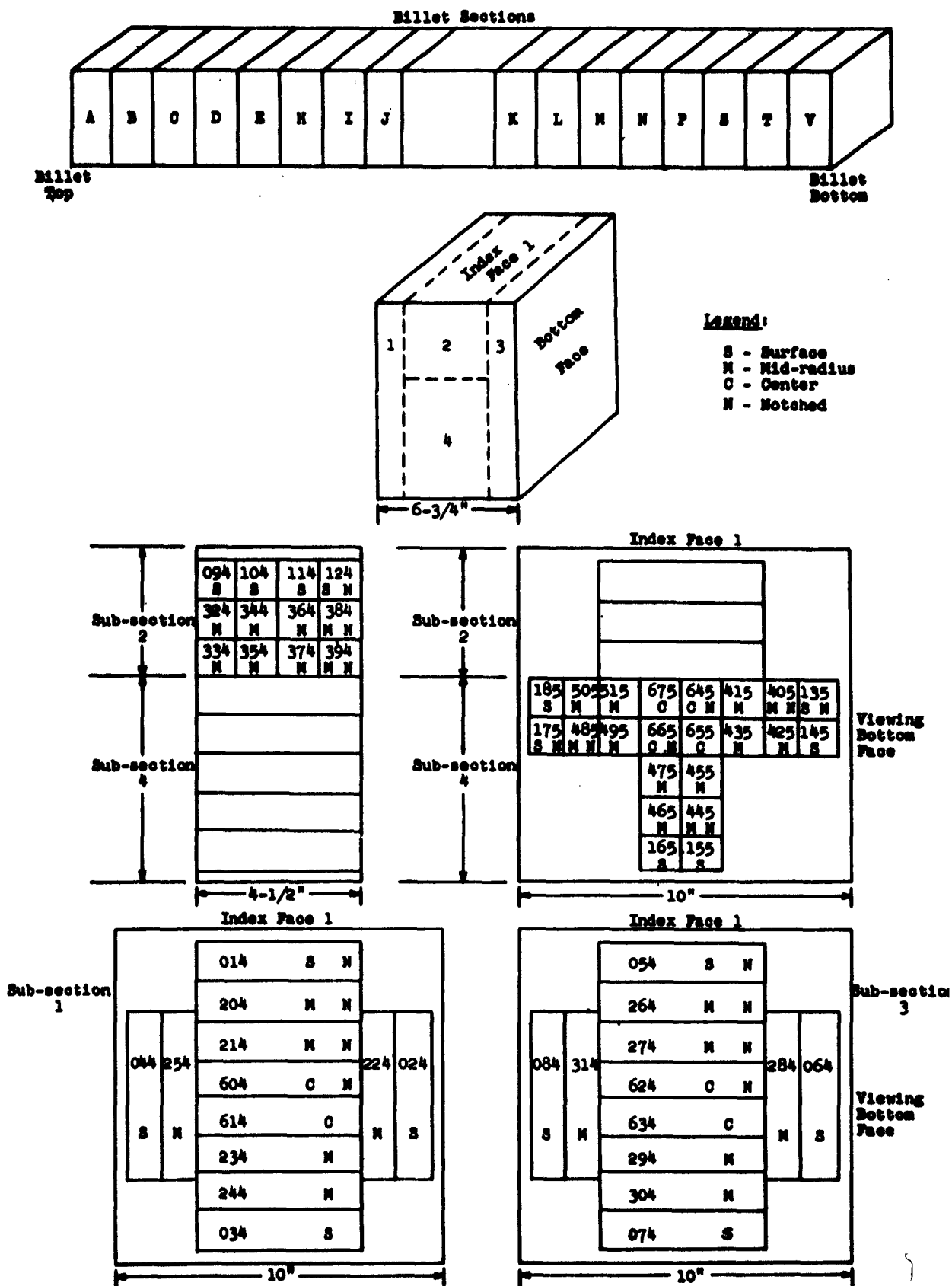
FIGURE 18 BILLET SECTIONING DIAGRAM
