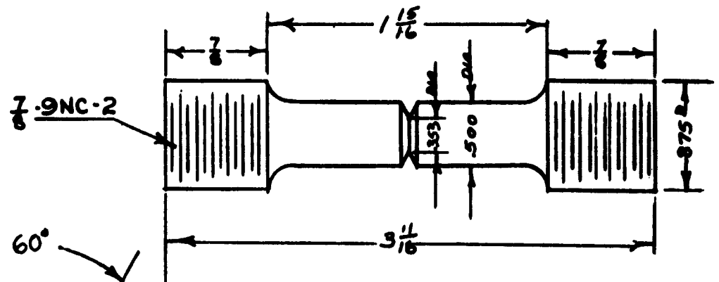
"NOTCHED" TENSILE SPECIMEN K_T = 5
