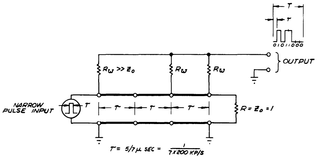
FIGURE 12 CODE-PRODUCING NETWORK
