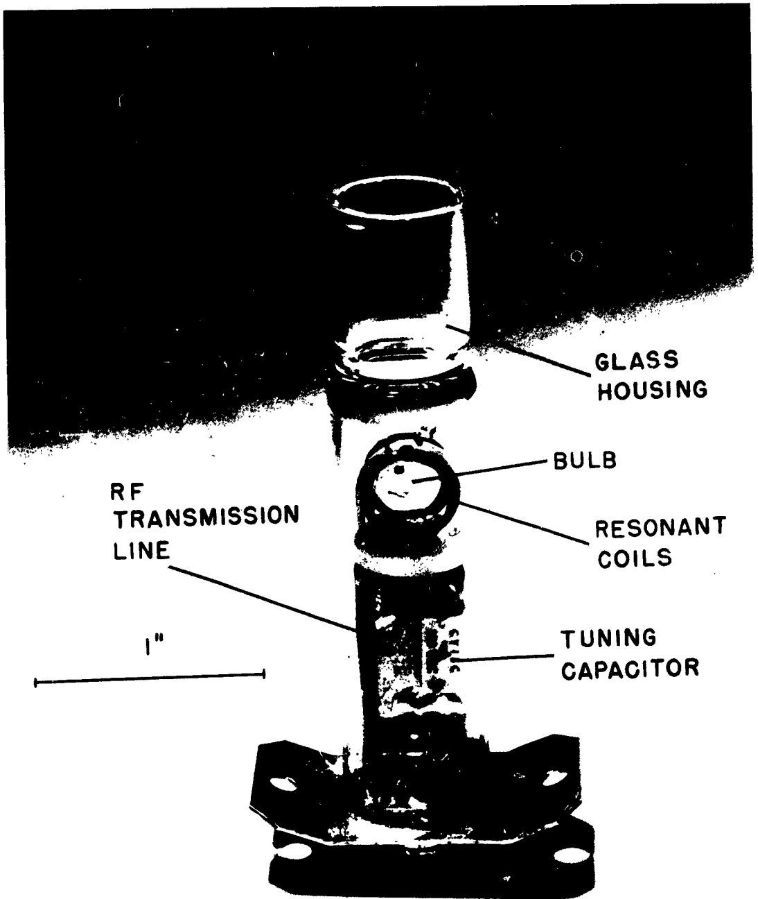
FIGURE 5 LAMP ASSEMBLY
