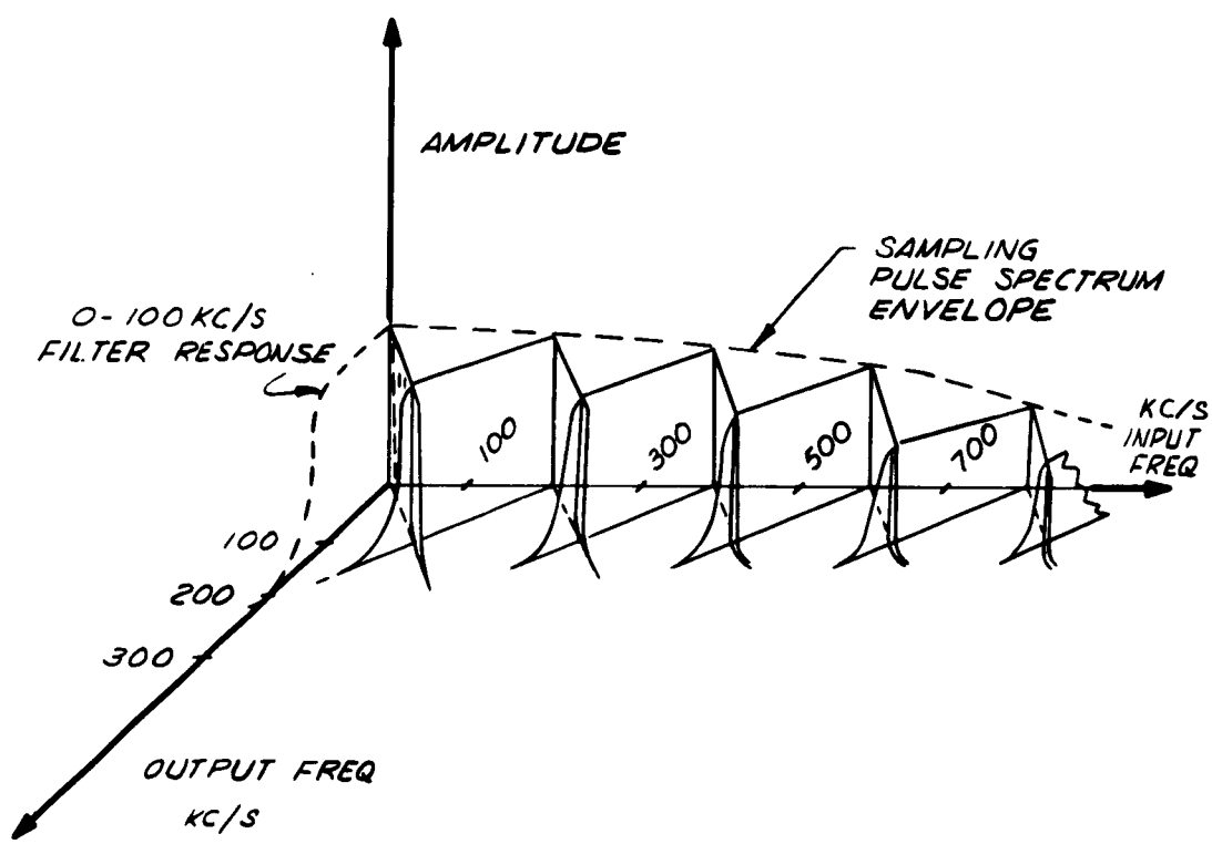
FIGURE 10 SIGNAL PROCESSOR RESPONSE
