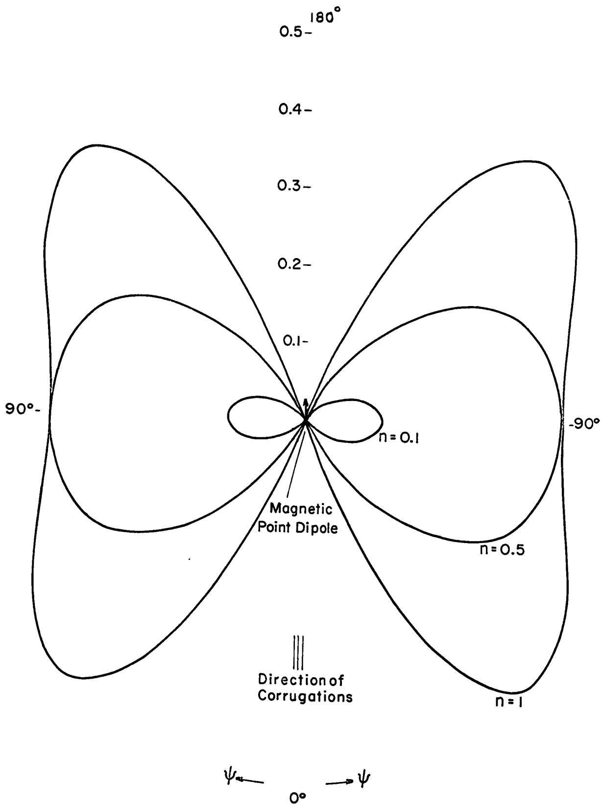
Figure 4. Surface Wave Power Angular Density \times (8\pi\omega\mu) .
