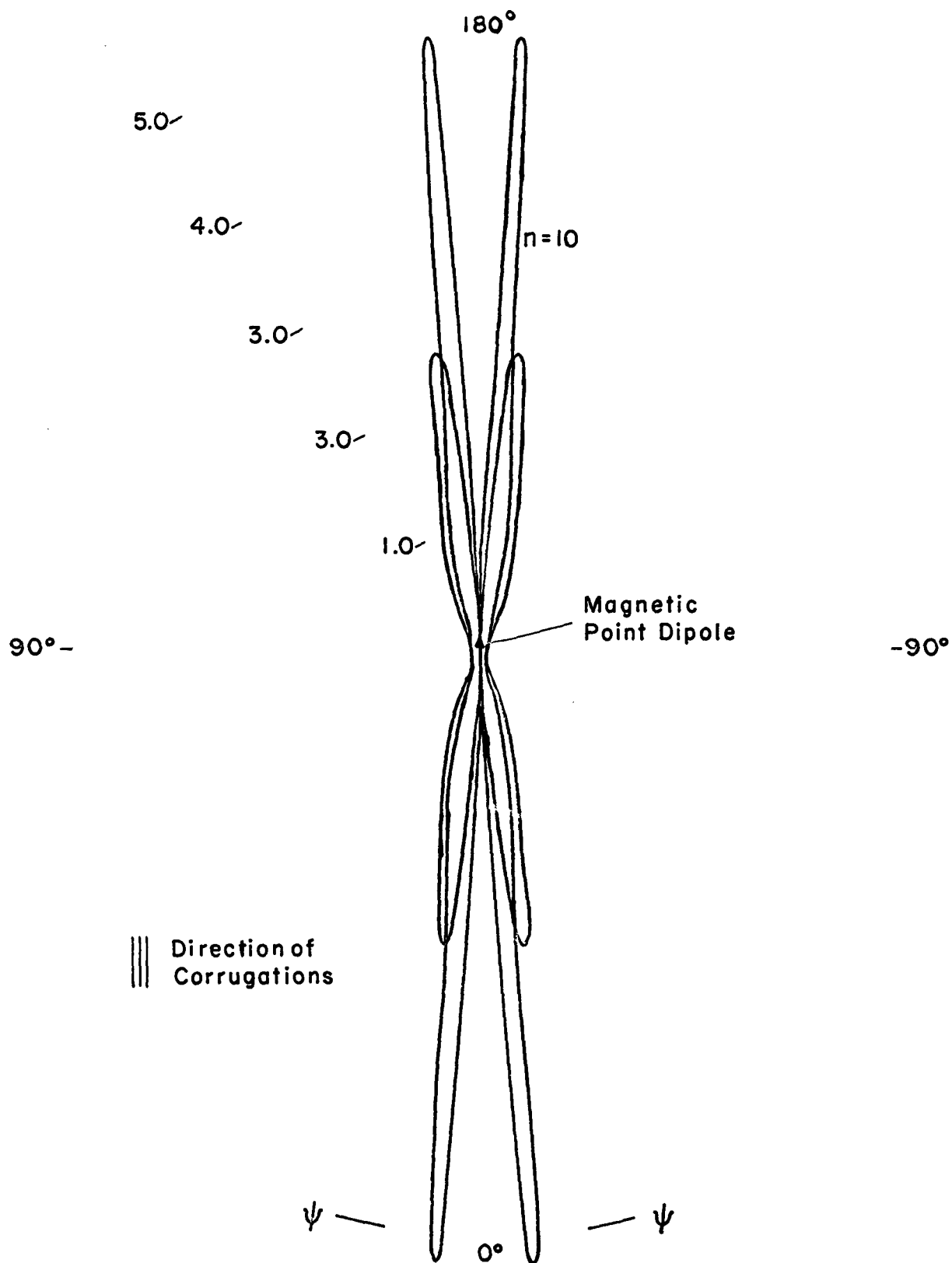
Figure 5. Surface Wave Power Angular Density x(8\pi\omega\mu) .
